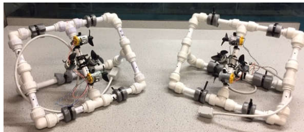
Figure 1. Two Seaperch UUVs.
