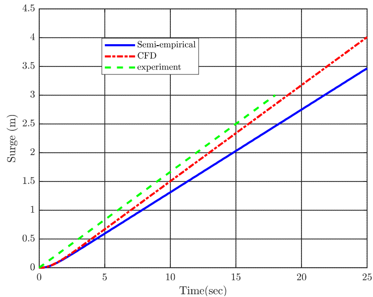
Figure 10. Surge response (developed with MATLAB [67]).
