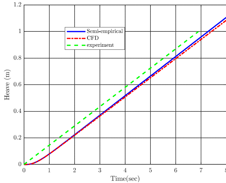
Figure 9. Heave response (developed with MATLAB [67]).
