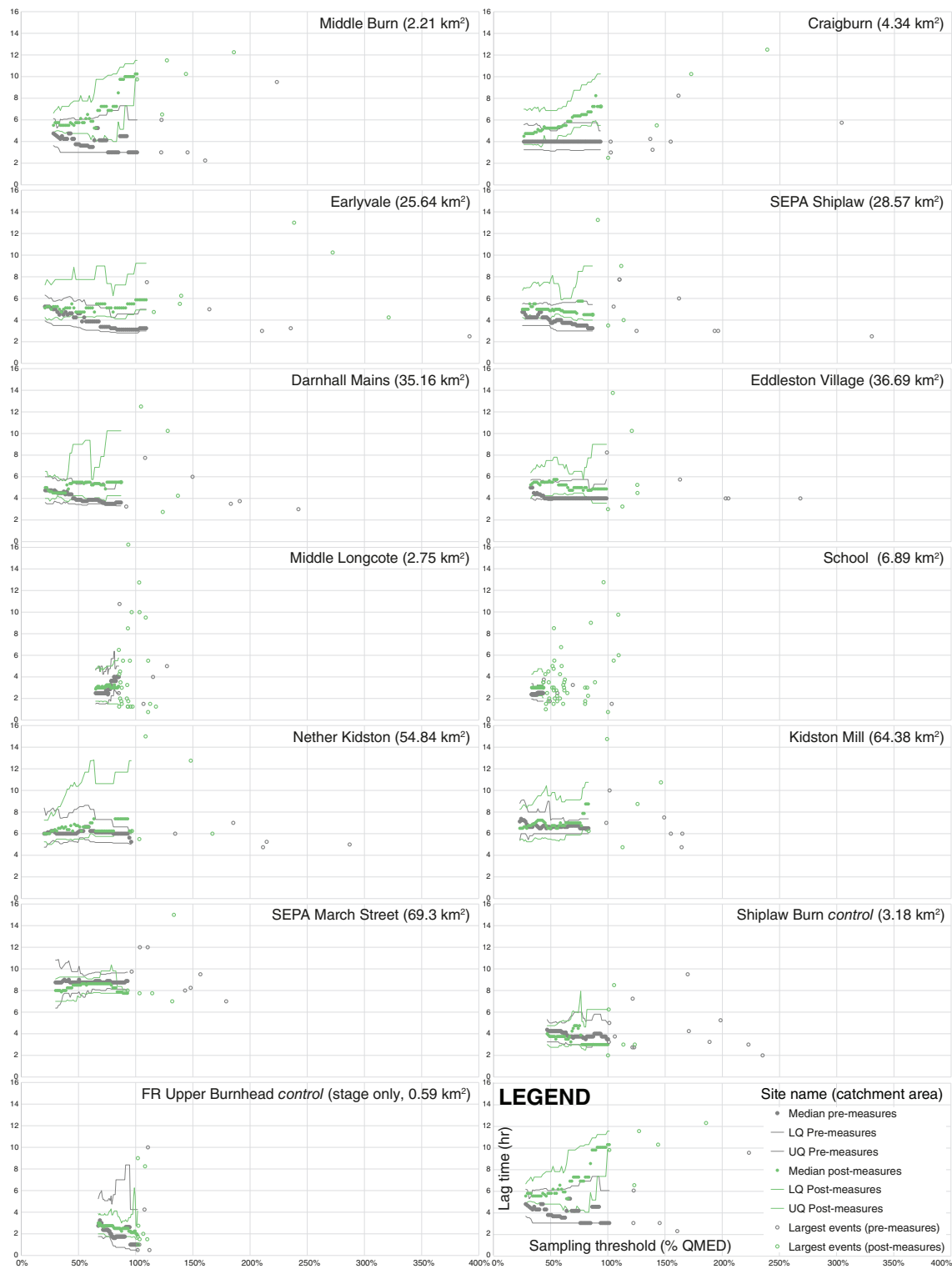
FIGURE 3 Median lag time for events in the baseline and experimental periods at different flow sampling thresholds (shown as a fraction of the median annual flood QMED). Median at each threshold in the different periods calculated as the median lag time for all events above the threshold, up to the point where the sample size in either period is <5. Open circles show lag for the largest individual events above this point. LQ/UQ: lower/upper quartiles. Sites are arranged upstream to downstream, with catchment area shown in each plot title. Sites are located on Figure 1. Details of natural flood management (NFM) interventions are in Table 1
