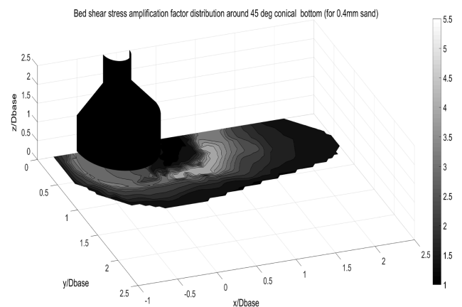
Figure 4: : Initiation of scour at 45° conical base structure (top), bed shear stress amplification contour map for same structure (bottom); flow direction from left to right.
