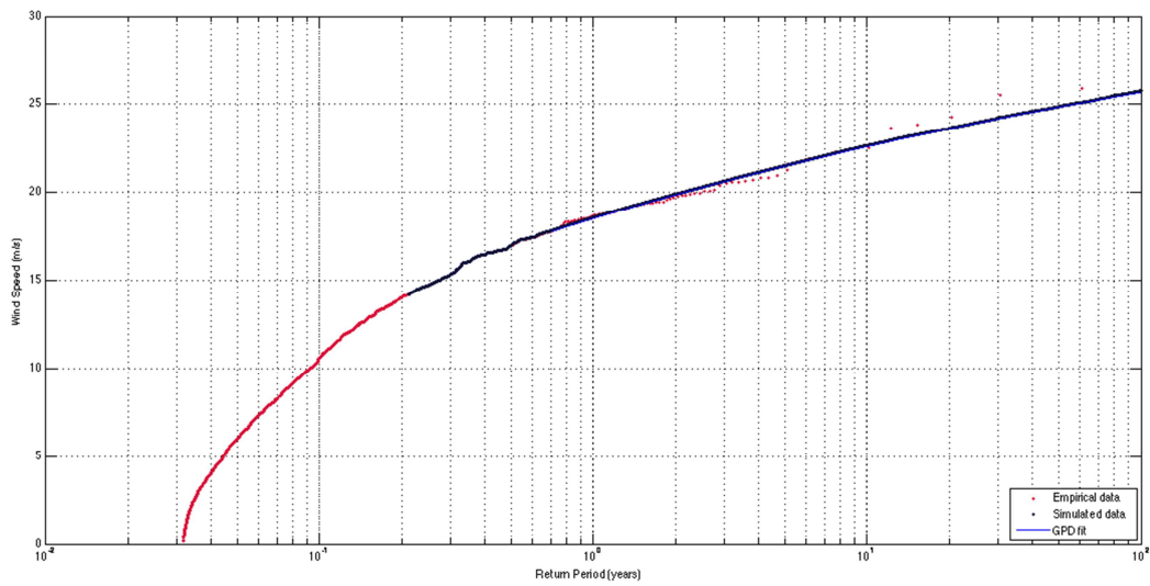
Figure 8 Comparison of the marginal distribution of U: empirical, simulated and GPD fit
