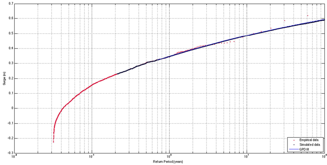
Figure 7 Comparison of the marginal distribution of S: empirical, simulated and GPD fit
