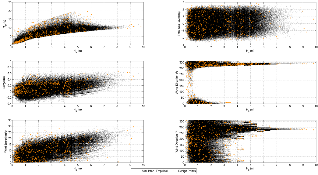
Figure 9 Simulated offshore data and design points output from the MDA algorithm
