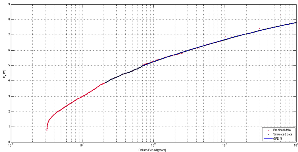
Figure 6 Comparison of the marginal distribution of HS: empirical, simulated and GPD fit
