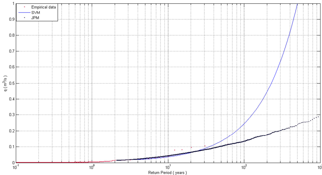
Figure 11 SVM V's JPM comparison for wave overtopping rates
