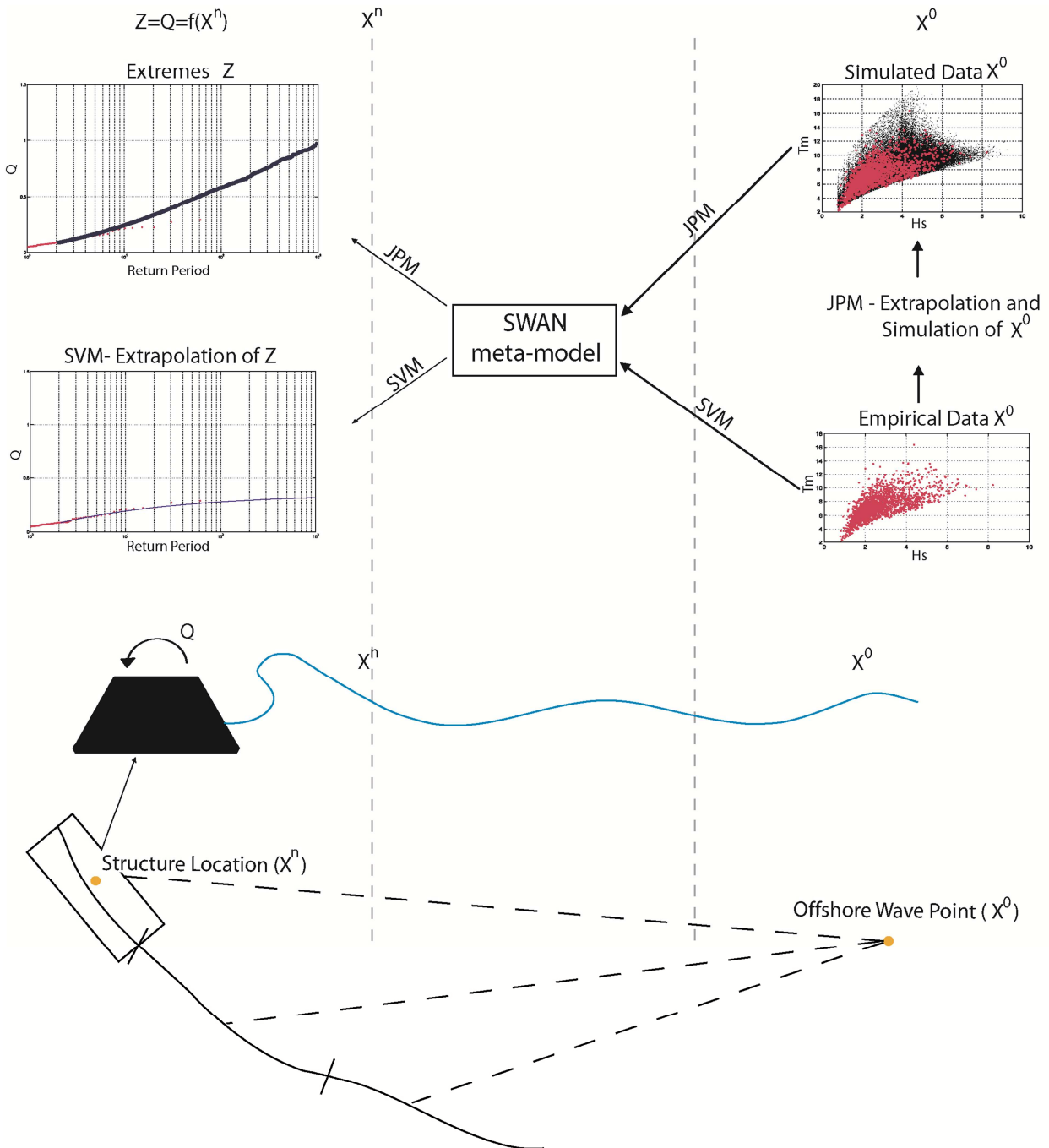
Figure 2 Conceptual diagram showing the SVM and JPM approaches
