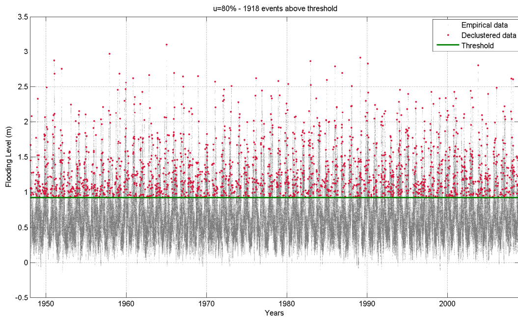
Figure 4 Flood level index time series and de clustered events
