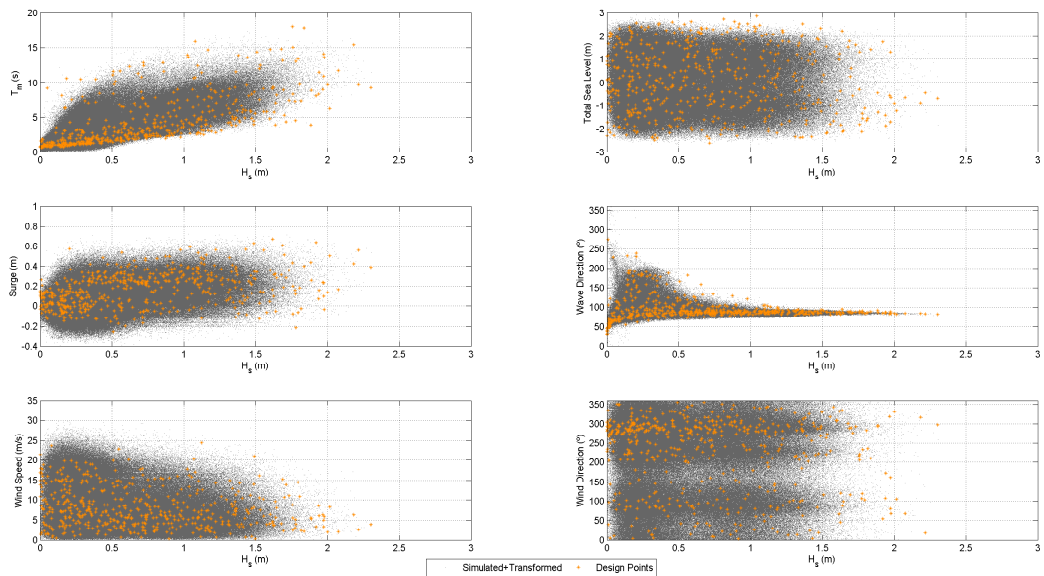
Figure 10 Simulated and transformed nearshore data with design points highlighted
