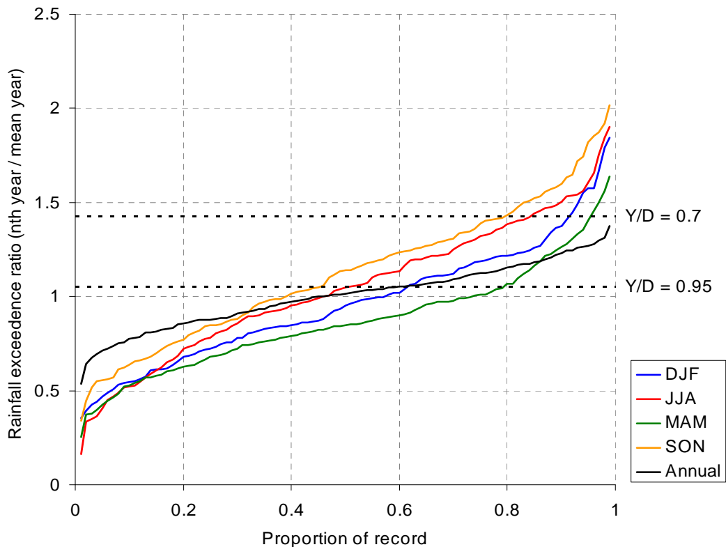
Figure 7.9 Rainfall exceedence – annual and seasonal and impact on Y/D ratio
