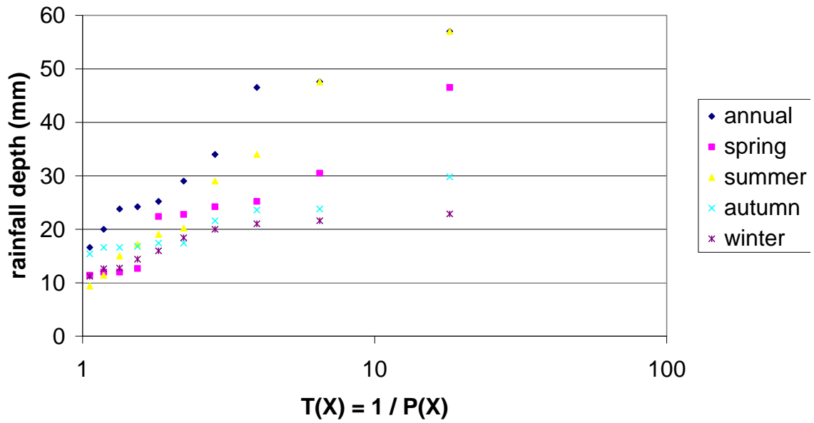
Figure 7.3 Observed event analysis by season – 6 hours
