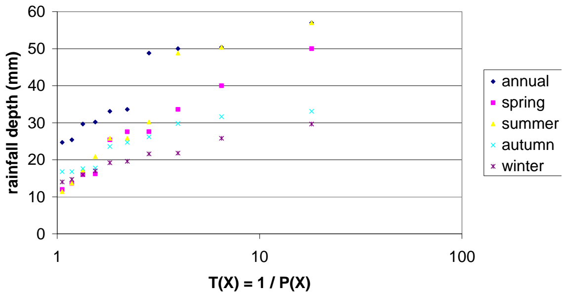
Figure 7.4 Observed event analysis by season – 24 hours
