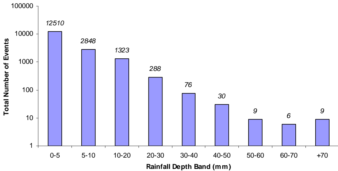
Figure 7.7 Events by depth bands in the 100 year series
