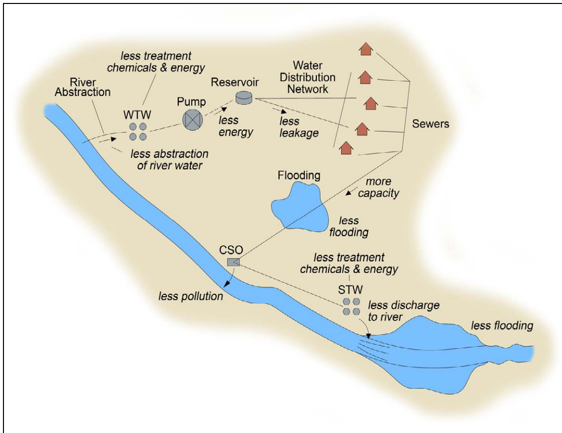
Figure 2.1 The benefits of rainwater harvesting
