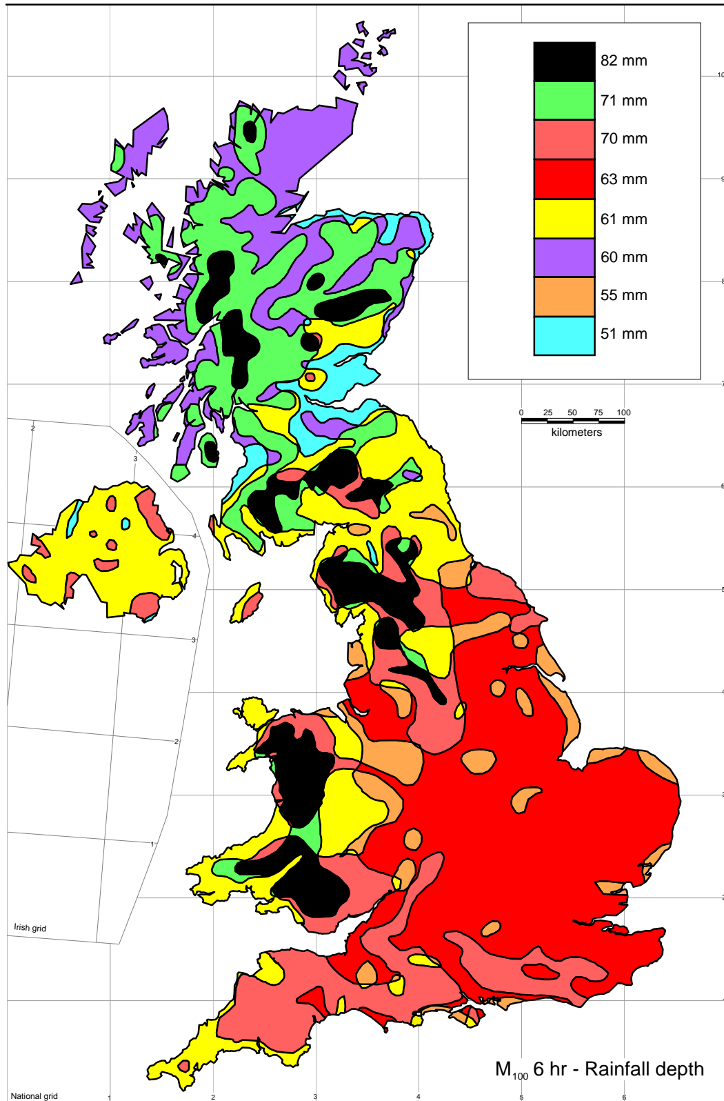
100 year 6 hour rainfall depths (based on FSR)
