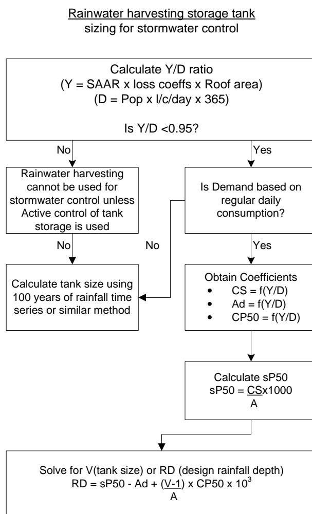
Figure A1 Flow chart for sizing of rainwater harvesting tanks for stormwater control
