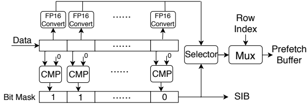
Fig. 12: The overview of the compaction processing unit.
