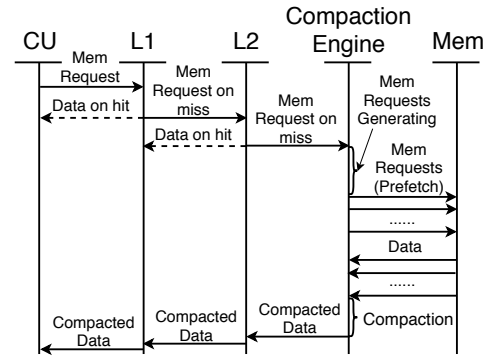
Fig. 8: An example of handling a data read request.
