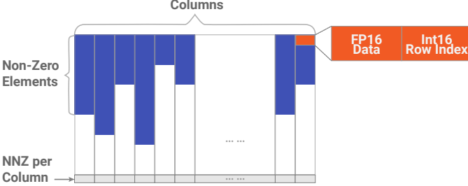
Fig. 5: The format of ELLPACK-DIB.
