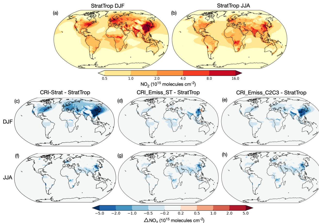
Figure 12. Average tropospheric column NO 2 in StratTrop simulations for DJF (a) and JJA (b). Differences in tropospheric NO 2 column in DJF and JJA between CRI-Strat and StratTrop (c and f), CRI_Emiss_ST and StratTrop (d and g), and CRI_Emiss_C2C3 and StratTrop (e and h).
