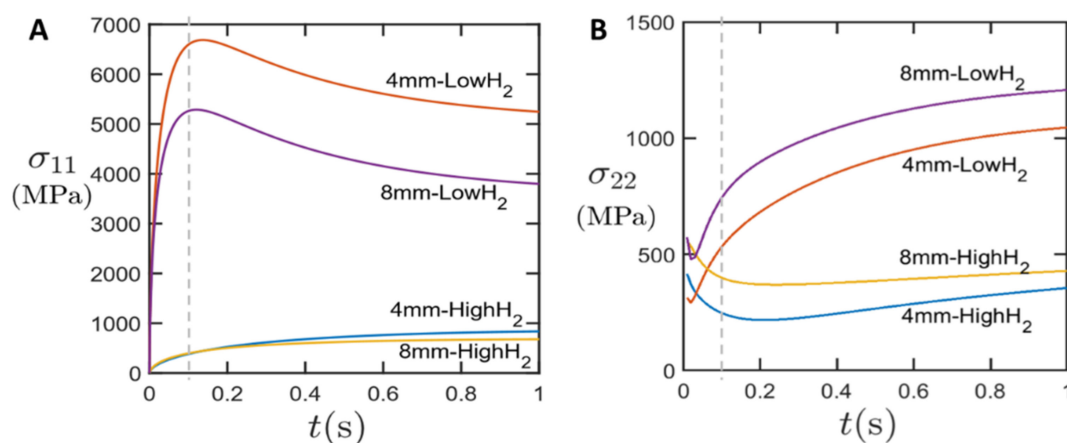
Figure 3. (A) Longitudinal stress \sigma_{11} between sample ends and (B) lateral stress \sigma_{22} at the laser spot (marked by red boxes in Figure 2). The dashed line marks 100 ms, where the snapshots for Figure 2 were taken.
