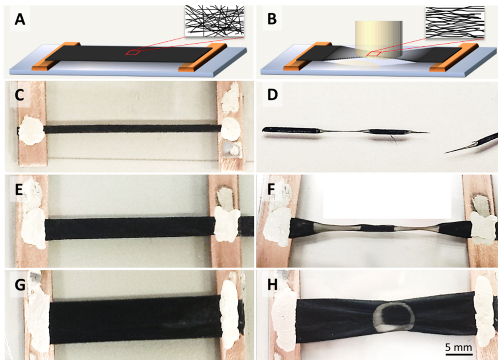
Figure 1. Schematics and photographs carbon nanotube (CNT) film samples of different widths before (A,C,E,G) and after (B,D,F,H) single point laser irradiation. The laser irradiated areas are visibly more transparent and contract into an hourglass shape, provided that the sample width is smaller than the laser spot. If the sample width matches or is larger than the laser spot, the network contracts in a non-uniform manner, in certain cases (H) even showing annular transparent regions. The insets in A and B show schematically the changes in microstructure alignment.
