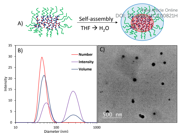
Figure 3. A) Self-assembly of HBP2 using a solvent switch method (slow addition of H 2 O into THF/polymer solution) leading to the formation of spherical core-shell particles; B) Dynamic light scattering (DLS) analysis of HBP2-g-PEGMEA 50 micelles (1 mg mL -1 ), and C) TEM micrograph of HBP2-g-PEGMEA 50 micelles.
