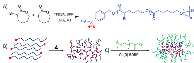
Figure 1. A) The copolymerisation of CL and BrCL catalysed by DPP and initiated by TFDBA leading to the gradient blocky \alpha -diazirine copolymers; B) Thermal activation of the diazirine leading to the unmasking of the carbene and the subsequent hyperbranching of the linear precursor polymers; C) Application of Cu(0)-RDRP techniques enables 'grafting-from' the PCL-based materials, leading to amphiphilic polymers.
