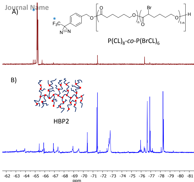
number of arms ( N_{\text{arms}} ) 52-54 of each of the HBPs (Table S6). 47 Based on the absolute molar masses (obtained via SEC-td), Figure 2. Stacked 19 F NMR spectra of the linear P(CL) 8 -co-P(BrCL) 6 (top) and the branched structure HBP2 (bottom, after 6 h of branching – end point data). The diazine has decomposed, thereby unmasking the carbene, which has then inserted in various C-H and C-O bonds of the polymer, thus creating a random hyperbranched structure (CDCl 3 ).
