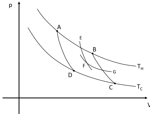
Figure 4: This diagram shows the original Carnot cycle, as well as another smaller Carnot cycle, EBGFE. By cutting more corners, i.e. by having many infinitesimal adiabats and isotherms, any quasi-static reversible cycle in the plane can be considered.
