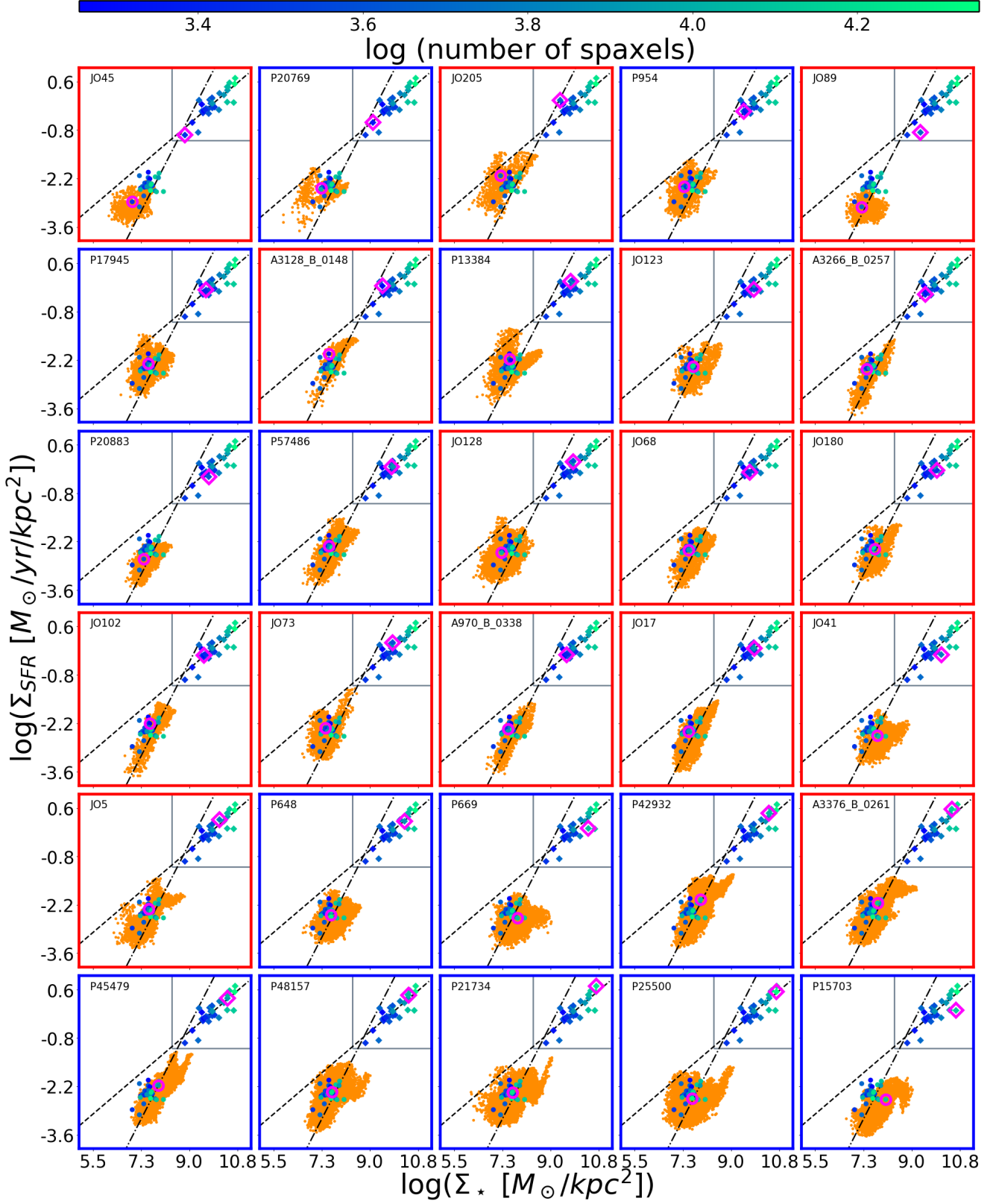
Figure 14. Comparison between the local and the global SFR- M_{*} relations. In each panel, the \Sigma_{\text{SFR}}-\Sigma_{*} relation of the galaxy listed in the upper corner is shown with orange dots. The mean \Sigma_{\text{SFR}} and \Sigma_{*} values of same galaxy is shown with an empty magenta circle. Filled circles show the mean \Sigma_{\text{SFR}} and \Sigma_{*} values for all the galaxies. They are colour coded by the number of spaxels in each galaxy and are all the same in all the panels. The axis aligned sub-panels show the global relation, obtained by summing the values of all the spaxels in each galaxy. The x-axis shows the \log(M_{*}[M_{\odot}]) , the y-axis shows the \log(\text{SFR}[M_{\odot}\text{yr}^{-1}]) . Filled diamonds are colour coded by the number of spaxels in each galaxy, the empty magenta diamond indicates the position of the galaxy shown in that panel. In all the panels, the dash-dotted line shows the fit from the upper left panel of Fig.3, the dashed line shows the fit to the global SFR-Mass relation. Galaxies surrounded by a red square belong to clusters, galaxies surrounded by a blue square belong to the field.
