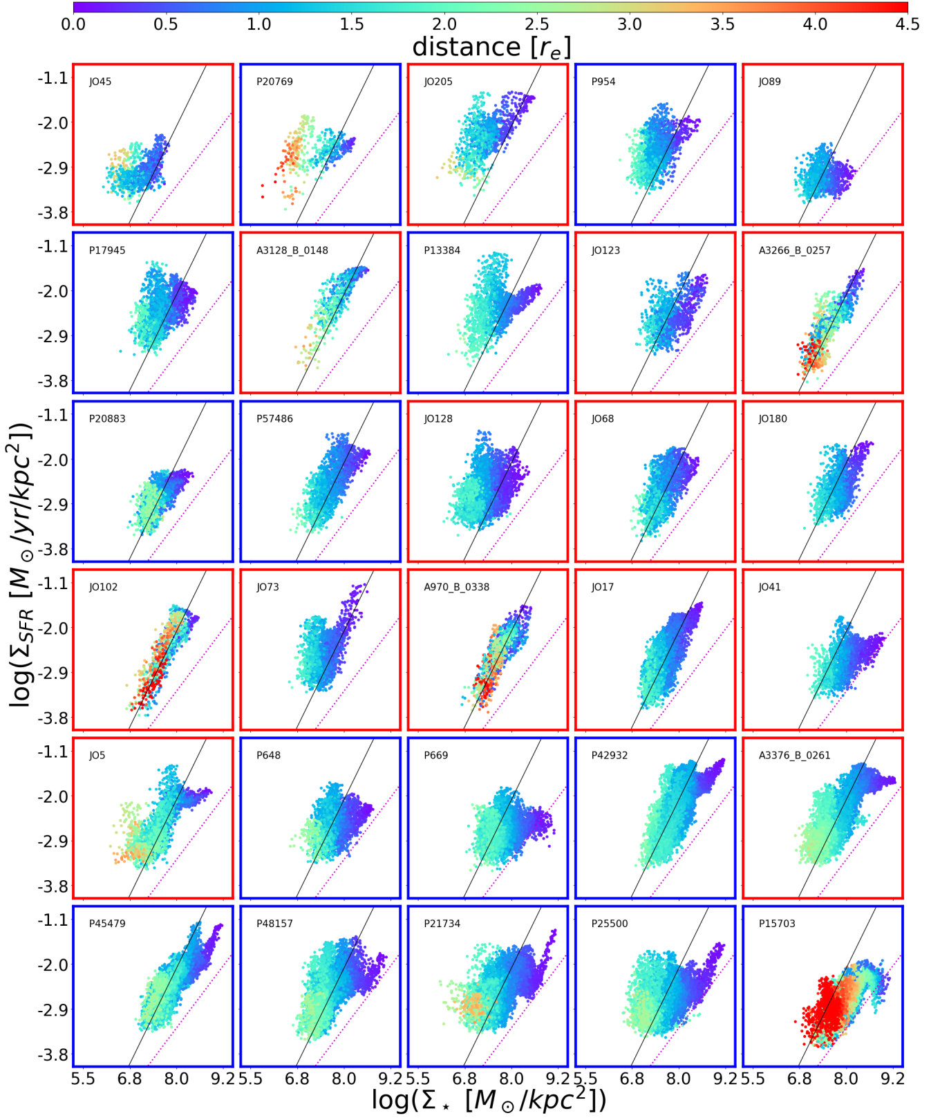
Figure 4. \Sigma_{\text{SFR}} - \Sigma_* relation for all galaxies in the sample, sorted by increasing stellar mass and colour coded by the galactocentric distance of each spaxel, in unit of r_e . Galaxies surrounded by a red square belong to clusters, galaxies surrounded by a blue square belong to the field. The black line represents the fit to the whole sample, from Fig.3. The magenta dotted line represents the effective threshold in spatially resolved specific SFR entailed by the adopted cuts in S/N corresponds to 10^{-11.2} \text{ yr}^{-1} \text{ kpc}^{-2} .
