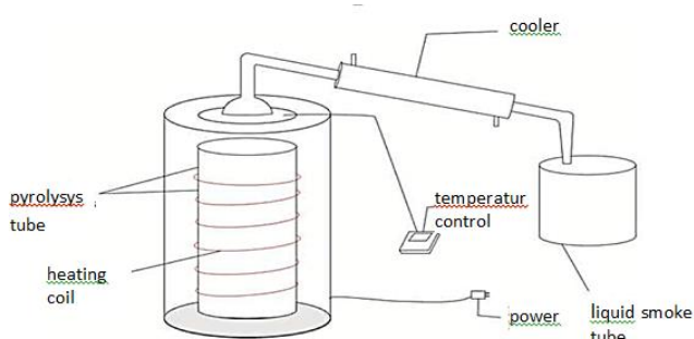
Figure 1. Pyrolysis Apparatus
