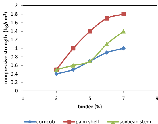
Figure 7. Effect of binder concentrations on compressive strength
