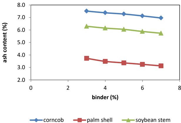
Figure 3. Effect of binder concentrations on ash content
