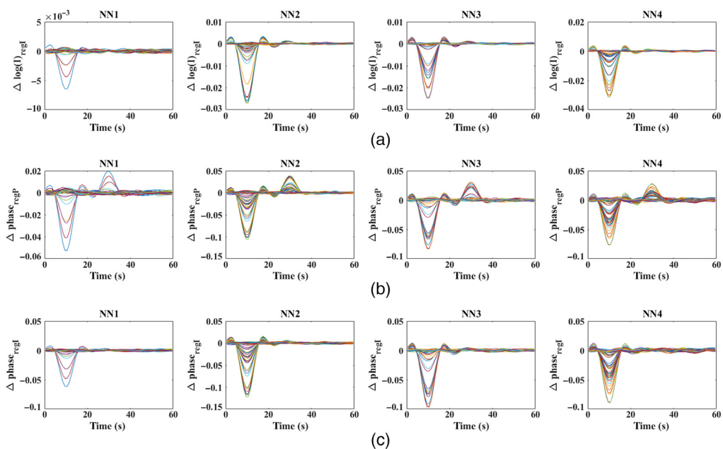
Fig. 8 (a) Regressed intensity measurements with short-distance intensity measurement; (b) regressed phase measurements with short-distance phase measurement; and (c) regressed phase measurements with short-distance intensity measurement post filtering and all noise-reduction steps.
