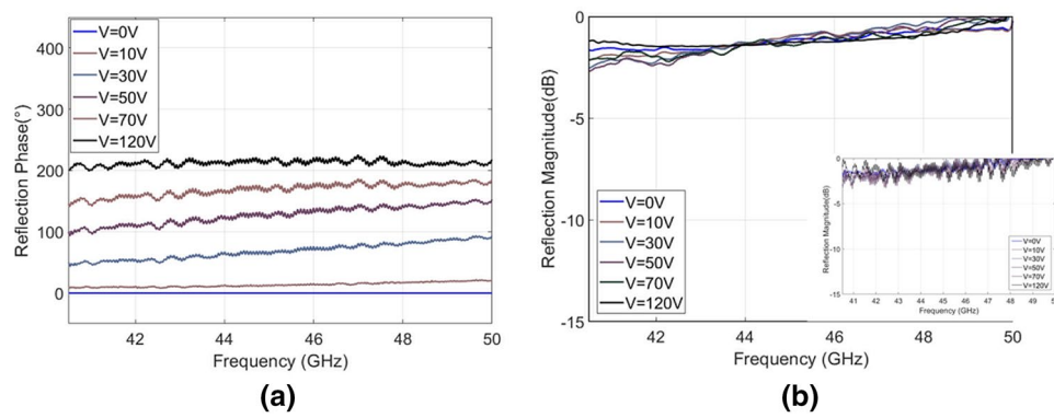
Figure 5. Wide bandwidth metasurface (40.5–50 GHz). (a) Reflection phase shift with respect to 0 V (approx. 0.10 mm cavity height) state. (b) Average reflection magnitude for different applied voltages (raw data shown in insert).
