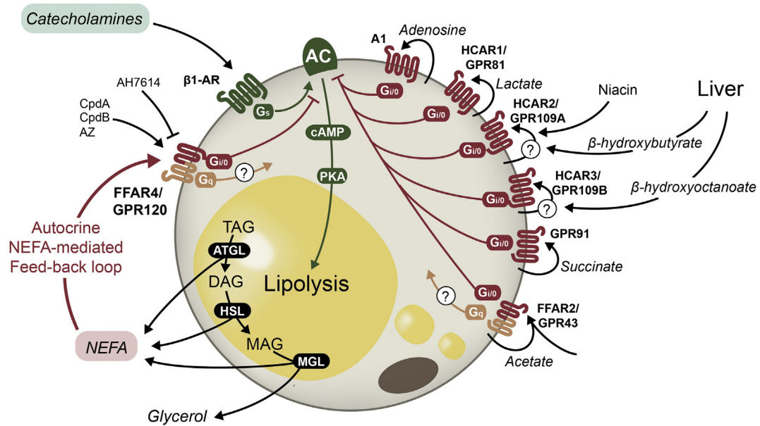
Figure 5: Simplified schematic overview of control of lipolysis by GPCRs with focus on FFAR4 in the context of the other putative autocrine feedback mechanisms. The left side indicates the autocrine NEFA and FFAR4 and Gi-mediated autocrine negative feedback loop on lipolysis characterized in the present study, including the pharmacological FFAR4 tool compounds used. The classical catecholamine, \beta 1-receptor, Gs, and adenylate cyclase (AC)-mediated stimulatory control of lipolysis are indicated in green. The right side indicates six different Gi-coupled metabolite sensing GPCRs, which all act as autocrine regulators of lipolysis and other adipocyte functions under different physiological circumstances: The adenosine A1 receptor, which is responsible for the original, classical autocrine effects of adenosine [52]; the lactate receptor, HCAR1/GPR81, which is responsible for the insulin, glucose-mediated inhibition of lipolysis [47]; the HCAR2/GPR109A receptor for circulating and possibly also locally produced \beta -hydroxybutyrate and the prototype anti-lipolytic drug niacin [53]; the HCAR3/GPR109B receptor for \beta -hydroxyoctanoate [54]; the SUCNR1/GPR91 receptor sensing stress and hypoxia-induced succinate excretion [39]; and FFAR2/GPR43, which senses acetate conceivably both through autocrine and paracrine mechanisms from certain subtypes of adipocytes [55].
