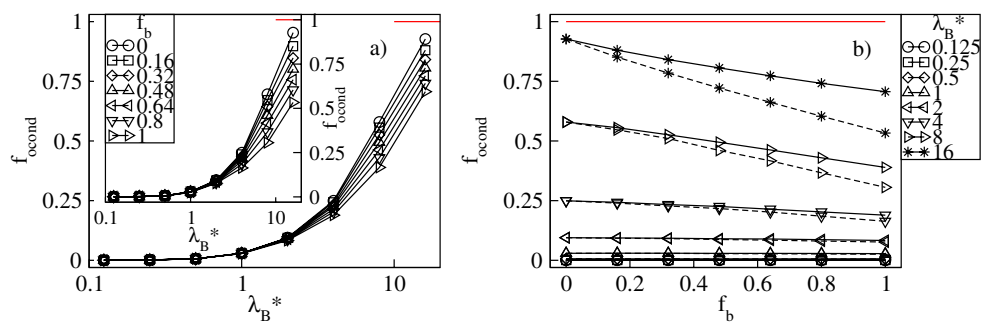
Figure 9. Overall fraction, f_{ocond} , of the condensed counterions versus the Bjerrum length, \lambda_B^* , plotted for a fixed number fraction, f_b , of the bulky counterions with a diameter \sigma_b^* = 2 ( \sigma_b^* = 3 in the inset) on the lin-log scale (a), and versus f_b at fixed values of \lambda_B^* on the lin–lin scale (b). In (b) the solid (dashed) lines represent the data for \sigma_b^* = 2 ( \sigma_b^* = 3 ). The red lines indicate f_{ocond} = 1 .
