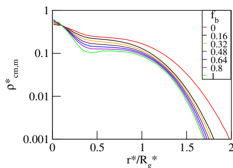
Figure 14. Log-lin plot of the radial density profiles, \rho_{cm,m}^* of the monomers around the center-of-mass of the dendrimer plotted for various fractions, f_b , of the bulky counterions with a diameter \sigma_b^* = 2 at \lambda_B^* = 16 . The maximum error bar for all the data sets is less than 5%.
