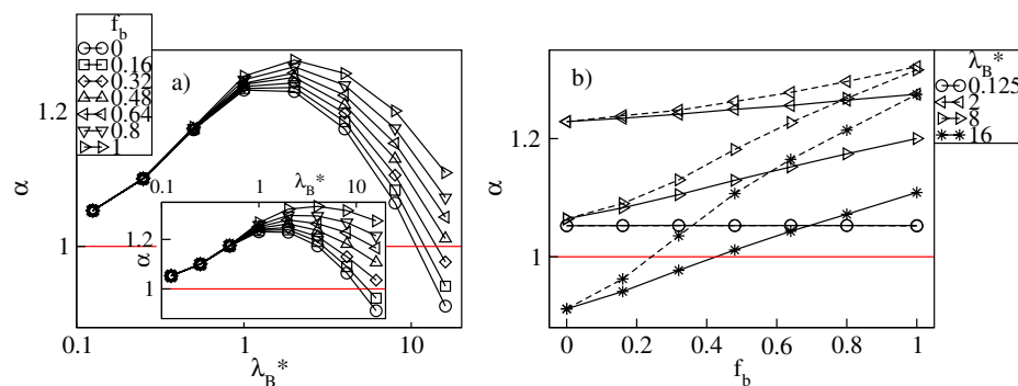
Figure 13. Swelling factor, \alpha , versus the Bjerrum length, \lambda_B^* , plotted for a fixed number fraction, f_b , of the bulky counterions with a diameter \sigma_b^* = 2 ( \sigma_b^* = 3 in the inset) on the lin-log scale (a), and versus f_b at fixed values of \lambda_B^* on the lin-lin scale (b). In (b) the solid (dashed) lines represent the data for \sigma_b^* = 2 ( \sigma_b^* = 3 ). The red lines indicate \alpha = 1 .
