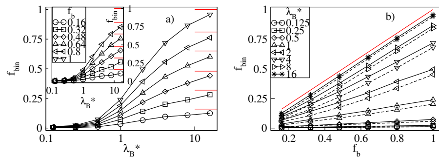
Figure 4. Fraction, f_{bin} , of the bulky counterions absorbed into the dendrimer versus the Bjerrum length, \lambda_B^* , plotted for a fixed number fraction, f_b , of the bulky counterions with a diameter \sigma_b^* = 2 ( \sigma_b^* = 3 in the inset) on the lin–log scale (a), and versus f_b for fixed \lambda_B^* on the lin–lin scale (b). In (b) the solid (dashed) lines represent the data for \sigma_b^* = 2 ( \sigma_b^* = 3 ). The red lines indicate the number fraction, f_b , of the bulky counterions.
