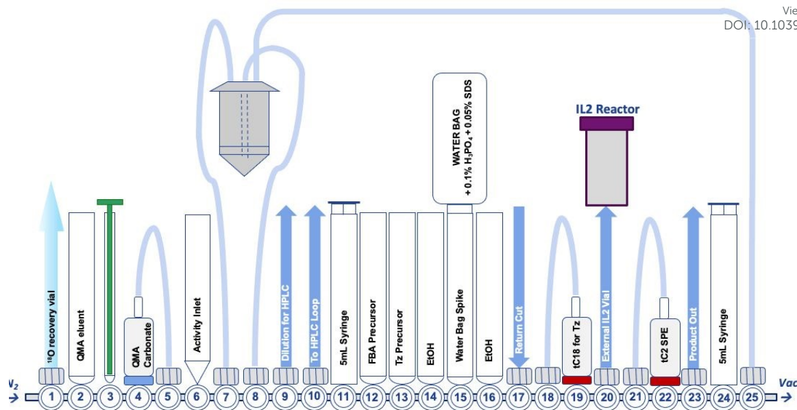
Figure 2. A schematic representation of the GE FASTLab™ cassette developed for the automated radiosynthesis of [ ^{18}\text{F} ]TTCO-IL2; a detailed description of the cassette setup appears in the supporting information (ESI Figure S14).
