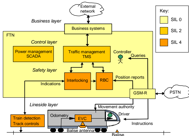
Fig. 1. Conceptual architecture of an ERTMS-enabled railway signalling system
