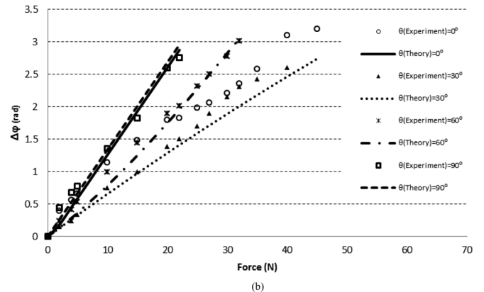
Fig. 4. Comparison of experimental and theoretical phase differences of the PM fibers when force is applied at different angles in relation to the slow axis of the (a) one-hole fiber and (b) two-hole fiber.
