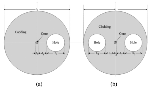
Fig. 1. (a) One-hole high-birefringence fiber that has a hole diameter b_1 of 30 \mu\text{m} and the distance between the right edge of the core to the left edge of the hole d_1 is 9 \mu\text{m} . (b) Two-hole high-birefringence fiber that has two holes with the same diameter b_2 of 27 \mu\text{m} and the distance between the right edge of the core to the left edge of the hole on the right d_2 is 14 \mu\text{m} .
