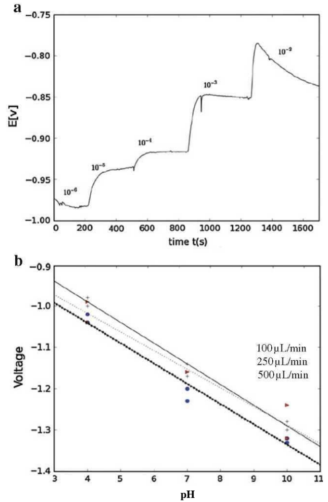
Fig. 2 a Potentiometric response of microfluidic devices for fixed flow rates Q = 100 \mu\text{l}/\text{min} , for \text{K}^2\text{ChemFET} . The concentration of KCl in M is given in the graph. b This shows the calculation curve for the pH sensor for different low rates, the red triangles represent low rate of 500 \mu\text{l}/\text{min} ; the blue circle represents 250 \mu\text{l}/\text{min} ; while the crosses represent flow rate of 100 \mu\text{l}/\text{min} . The trend lines for 100, 250, and 500 \mu\text{l}/\text{min} are shown by the dotted, straight, and thick dotted lines
