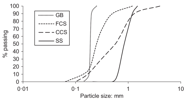
Fig. 2. Particle size distributions for the four materials: glass ballotini (GB), fine carbonate sand (FCS), coarse carbonate sand (CCS) and silica sand (SS)
