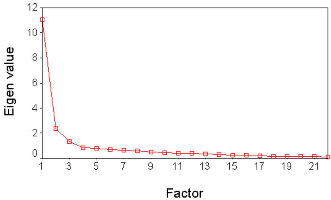
Scree-plot of the CES
