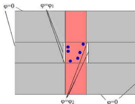
Figure 2. 2D finite element model showing boundary conditions.
