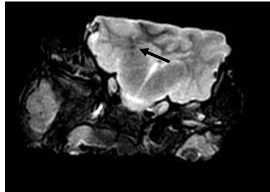
Fig. 5 MRI image using T1-w FSE in vitro.
