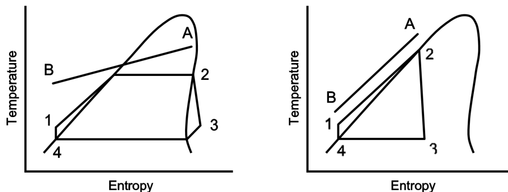
Figure 1: Illustrative T-s diagrams showing conventional ORC with dry saturated vapour at the expander inlet, and TFC with wet saturated vapour at the expander inlet
