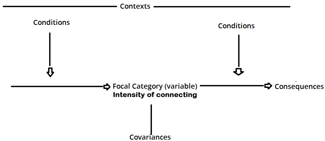
Figure 11: Axial coding
