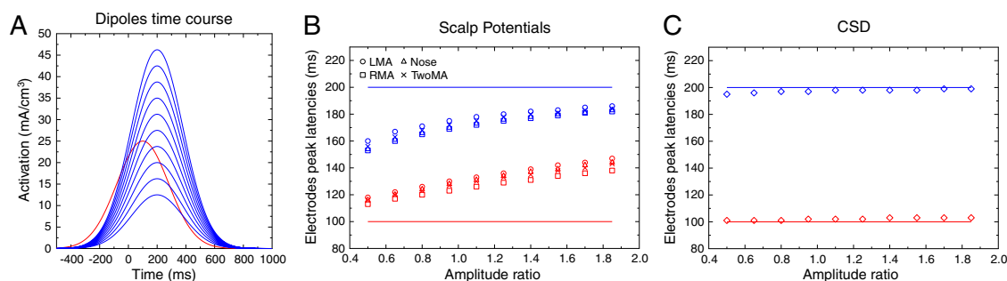
Fig. 6. A. Time courses of the simulated cortical dipoles. B. Peak latencies of the simulated dipoles (solid lines) for each dipole–amplitude ratio, and recovered potential peak latencies (empty symbols) for each reference electrode. Despite a constant time course of the underlying dipoles, the recovered scalp latencies differ dramatically as a function of the amplitude ratio. C. Same information after CSD transform: The recovered latencies are in close agreement with the underlying dipole time course.
