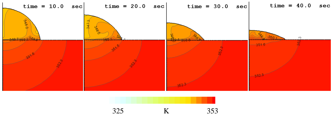
Figure 8: Predicted temperature distribution within the liquid and the solid during the vaporisation process using the full solution. [Initial surface temperature 80°C, initial contact angle 90 degrees]
