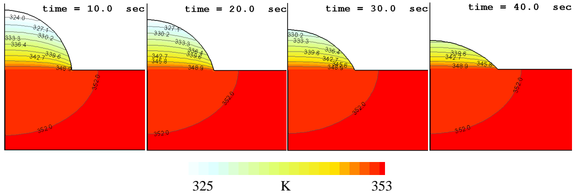
Figure 11: Predicted temperature distribution within the liquid and the solid during the vapourisation process, as predicted by the simplified model [Initial surface temperature 80°C, initial contact angle 90 degrees]
