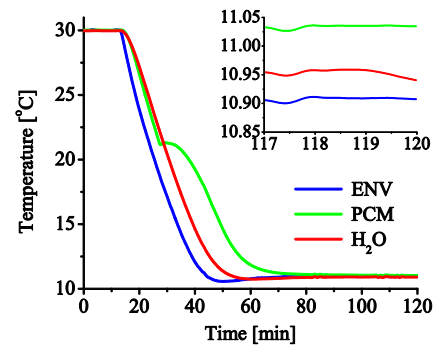
Figure 12. The Ser_Par configuration - PCM T-history curves when using cubic fitting.
