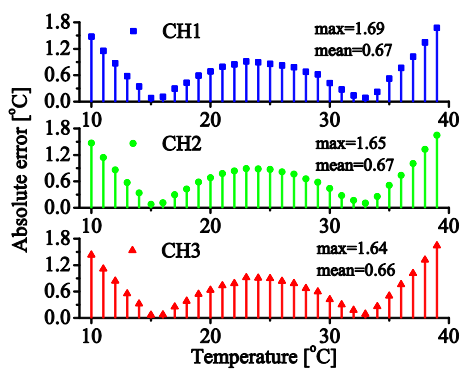
Figure 5. Calibration measurement based absolute error values when using linear fitting for WB linearization circuit; CH1 – later used for environment (ENV) measurement; CH2 – PCM measurement; CH3 – H 2 O measurement.
