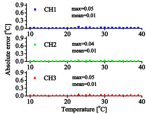
Figure 8. Calibration measurement based on absolute error values when using cubic fitting for the Ser_Par linearization circuit; CH1 – later used for environment (ENV) measurement; CH2 – PCM measurement; CH3 – H 2 O measurement.
