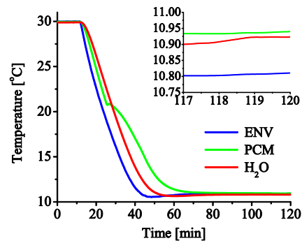
Figure 10. The WB configuration - PCM T-history curves when using cubic fitting.
