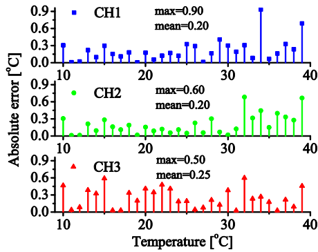
Figure 7. Calibration measurement based on absolute error values when using cubic fitting for the WB linearization circuit; CH1 – later used for environment (ENV) measurement; CH2 – PCM measurement; CH3 – H 2 O measurement.
