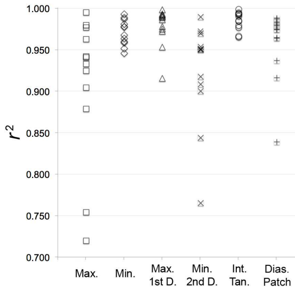
Figure 7 Coefficient of determination ( r^2 ) between mean pulse/heart rate values and the reference (ECG) for each of the 12 subjects by each of the six PPG methods.
