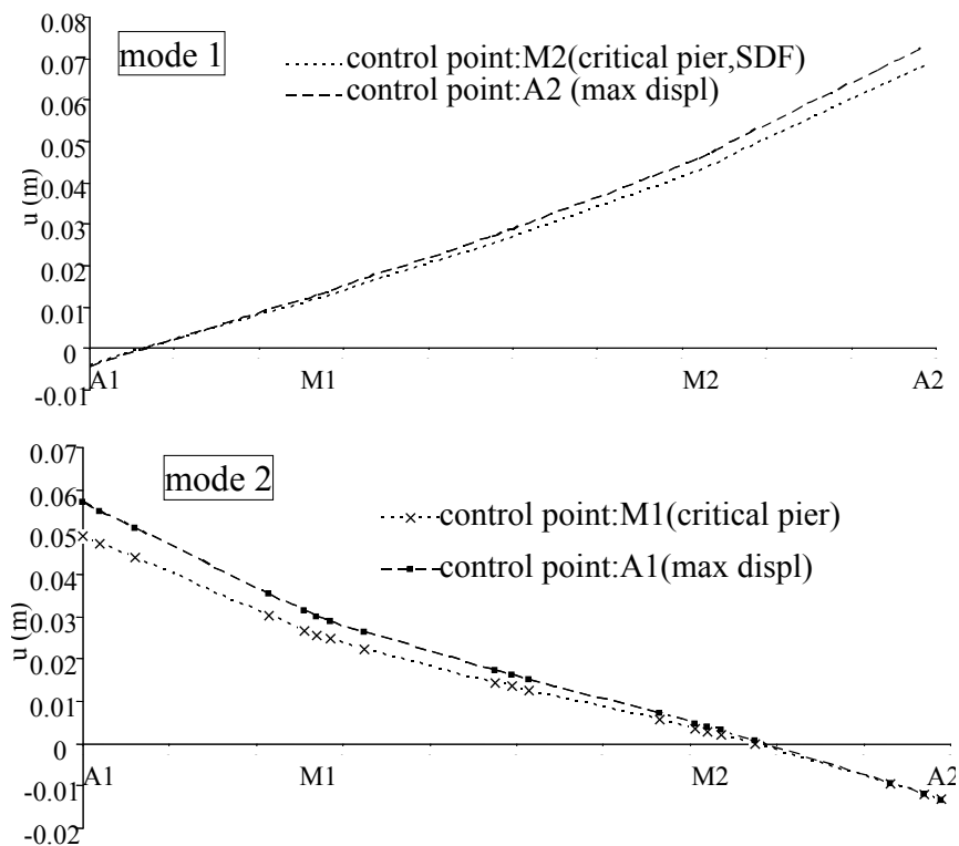
Figure 4: ‘Modal’ deck displacements derived with respect to different control points – inelastic behaviour of the overpass bridge ( A_g=0.16g )
