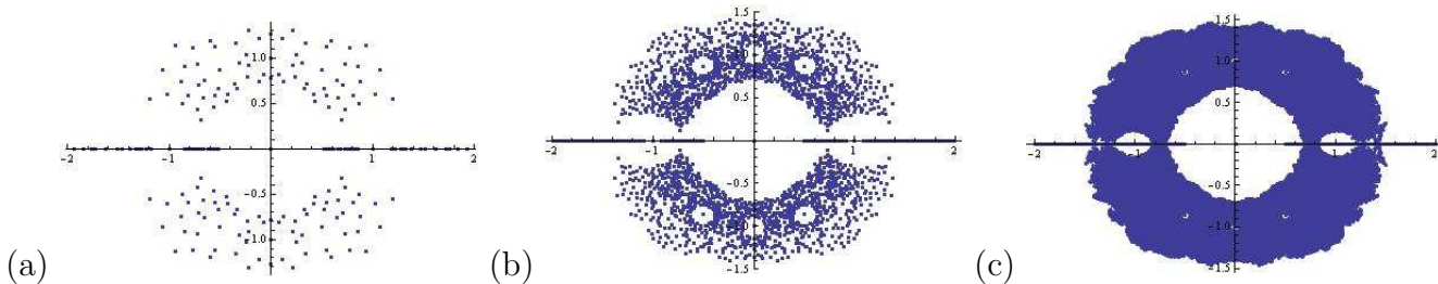
Figure 1: The position, on the complex plane, of the zeros of 50000 random integer polynomials with coefficients -1, 0 or 1 , for degrees upto 4, in part (a), 6, in part (b) and 10, in part (c).
