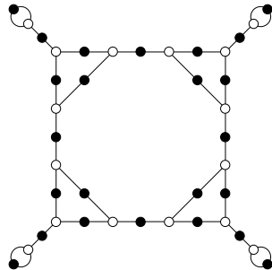
\Gamma(24; 24, 2, 2) 24, 8, 3, 3, 3, 3, 1, 1, 1, 1
