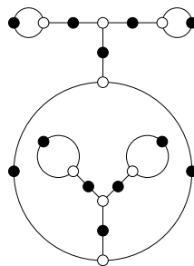
10, 10, 1, 1, 1, 1 ( \sqrt{5} )
