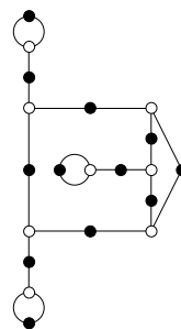
10, 8, 3, 1, 1, 1 ( \mathbb{Q} )
