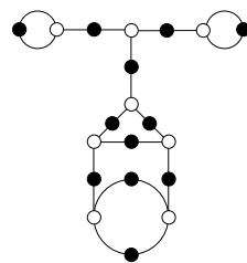
13, 4, 3, 2, 1, 1 ( \mathbb{Q} )
