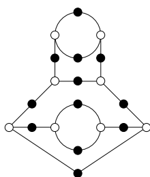
6, 6, 4, 4, 2, 2 ( \mathbb{Q} )
