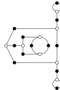
9, 8, 3, 2, 1, 1 (cubic)
