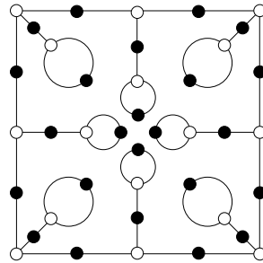
\Gamma(32; 32, 4, 2) 32, 8, 1, 1, 1, 1, 1, 1, 1, 1
