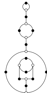
9, 7, 3, 2, 2, 1 (cubic)
