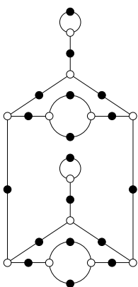
\Gamma_1(10) 10, 10, 5, 5, 2, 2, 1, 1
