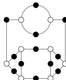
6, 6, 4, 3, 3, 2 ( \mathbb{Q} )
