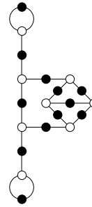
11, 5, 3, 3, 1, 1 ( \sqrt{5} )
