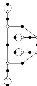
10, 10, 1, 1, 1, 1 ( \sqrt{5} )
