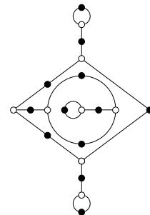
9, 7, 5, 1, 1, 1 ( \mathbb{Q} )
