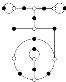
12, 6, 3, 1, 1, 1 ( \mathbb{Q} )
