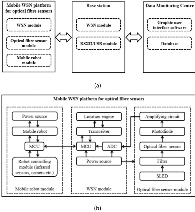
Fig. 1. (a) System architecture of the WSN platform for the optical fiber sensors. (b) Schematic of mobile WSN platform for the optical fiber sensors.
