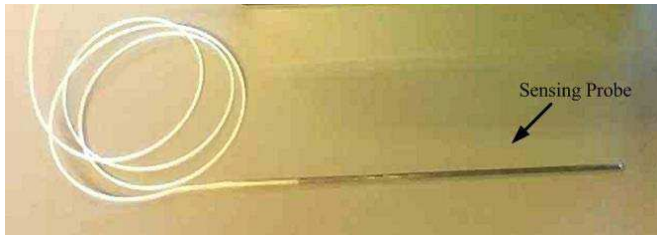
Fig. 2. Photograph of the FBG temperature sensor created for a WSN protected by an aluminium tube.
