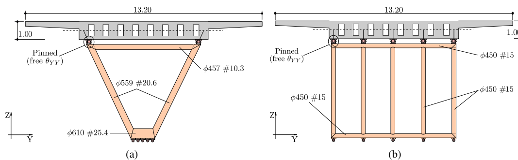
Figure 2. Schematic cross section of the considered UD-CSB, where \phi is the diameter and # is the thickness of the metallic struts: (a) Concentrated diverting struts; (b) Expanded diverting struts. Units of the deck in metres and units of steel struts in millimetres.
