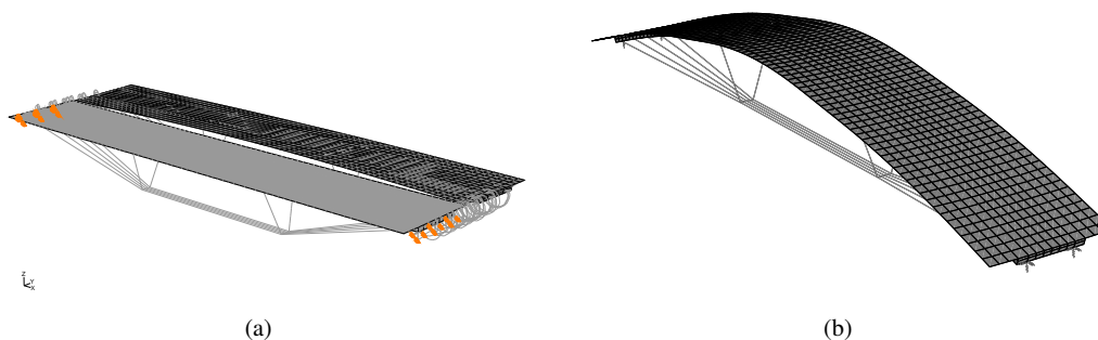
Figure 5. Fundamental vibration modes in models with different support conditions: (a) model with laminated elastomeric bearings (LEB): transverse rigid body displacement. T_{1T} = 1.43 s; (b) model with pot bearings (POT), classical layout: first order vertical flexure of the deck. T_1 = 1.28 s
