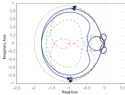
Fig. 11. Nyquist diagrams for the case of the subject motorcycle fitted with an optimized steering compensator. The acceleration-related inertial forces are: -2 \text{ m/s}^2 (black) dotted line, 0 \text{ m/s}^2 (blue) solid line, 2 \text{ m/s}^2 (green) dashed line and 4 \text{ m/s}^2 (red) dash-dot line. The machine speed is 80 m/s and its roll angle is 0^\circ .
