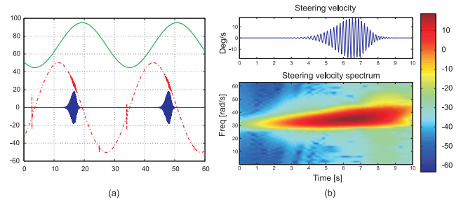
Fig. 3. a) Simulated weave-mode burst oscillations in the subject motorcycle under straight-running conditions. The speed is shown as the solid (green) line, 10 \times the acceleration is shown as the dot-dashed (red) line, while 10 \times the steering velocity is shown as the solid (blue) bursting characteristic (in rad/s). (b) Short-Period Fourier Transform of the steering velocity signal given in (a). Data between 10 s and 20 s was extracted for analysis - bursting is apparent between 14 s and 18 s (a). The bursting frequency increases from approximately 33 rad/s to approximately 38 rad/s in sympathy with the speed increase on this time interval.
