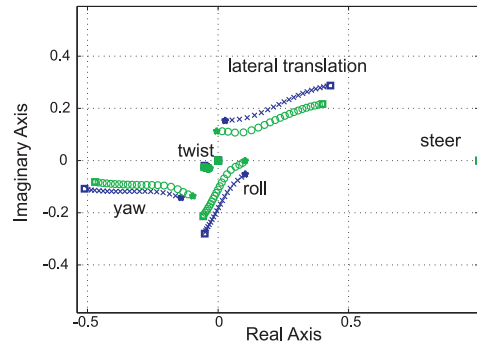
Fig. 6. Straight-running weave-mode eigenvector loci for the subject motorcycle (steering damper fitted) with acceleration-related inertial force the varied parameter for speeds of 70 m/s (blue \times ) and 80 m/s (green \circ ). The acceleration-related inertial forces are varied between -4 \text{ m/s}^2 and 4 \text{ m/s}^2 . The 13 eigenvector components corresponding to the generalised coordinates are shown; the eigenvectors are normalized so that the steer angle component is +1. The largest acceleration-related inertial force ( 4 \text{ m/s}^2 ) is marked with a \star , while braking at -4 \text{ m/s}^2 is marked with a \square . As with the classical weave mode, the five dominant components are: the machine's lateral translation, and the yaw, roll, frame twist and steer angles. The acceleration-related inertial forces reduce the amplitude of the lateral translation, and the yaw, roll and twist angle components. Under acceleration the weave mode of the subject motorcycle becomes 'wobble like'.
