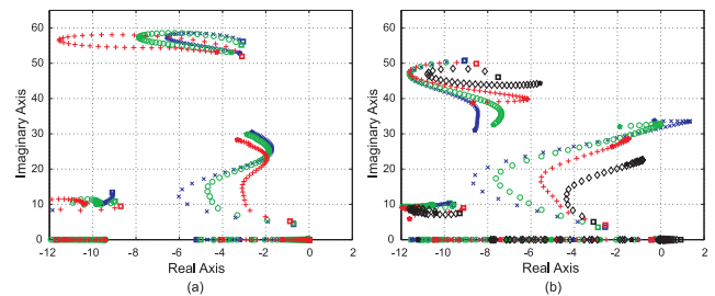
Fig. 7. Root-loci of the subject motorcycle with a steering damper fitted. Speed is the varied parameter for roll angles of 0^\circ (blue \times ), 15^\circ (green \circ ), 30^\circ (red + ) and 45^\circ (black \diamond ). The speed is varied from 9 m/s to 95 m/s in steps of 2 m/s. The highest speed is marked with a \star and the lowest speed with a \square . In (a) the braking-related acceleration is -4 \text{ m/s}^2 , while in (b) the acceleration is 4 \text{ m/s}^2 .
