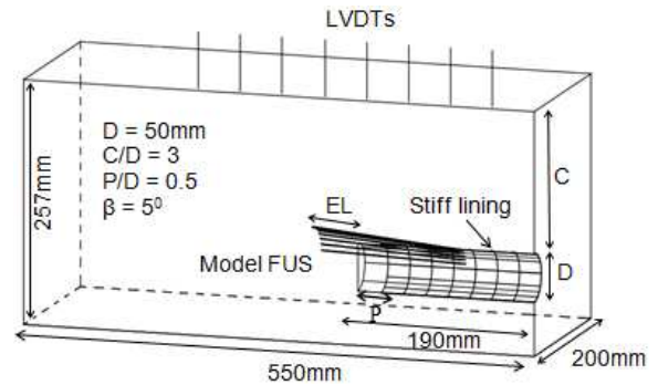
Figure 5. Diagram of model apparatus.
