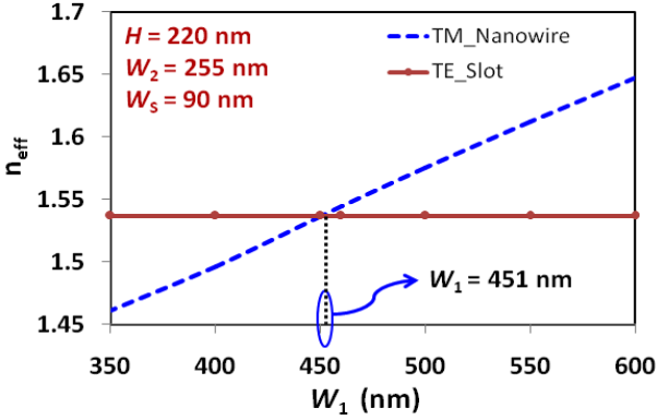
Fig. 2. Variation of n_{\text{eff}}\text{-TM} of strip WG with W_1 in the absence of slot WG. The horizontal line represents the n_{\text{eff}}\text{-TE} (1.53716) inside the Slot WG in absence of strip WG.
