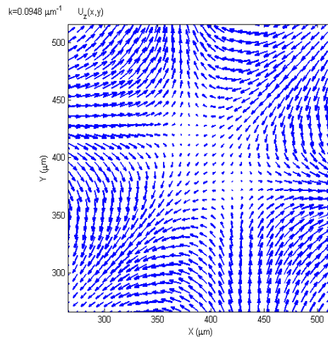
Figure 2.24. The shear S_{21} mode of \vec{U}_t = \vec{U}_x + \vec{U}_y .
