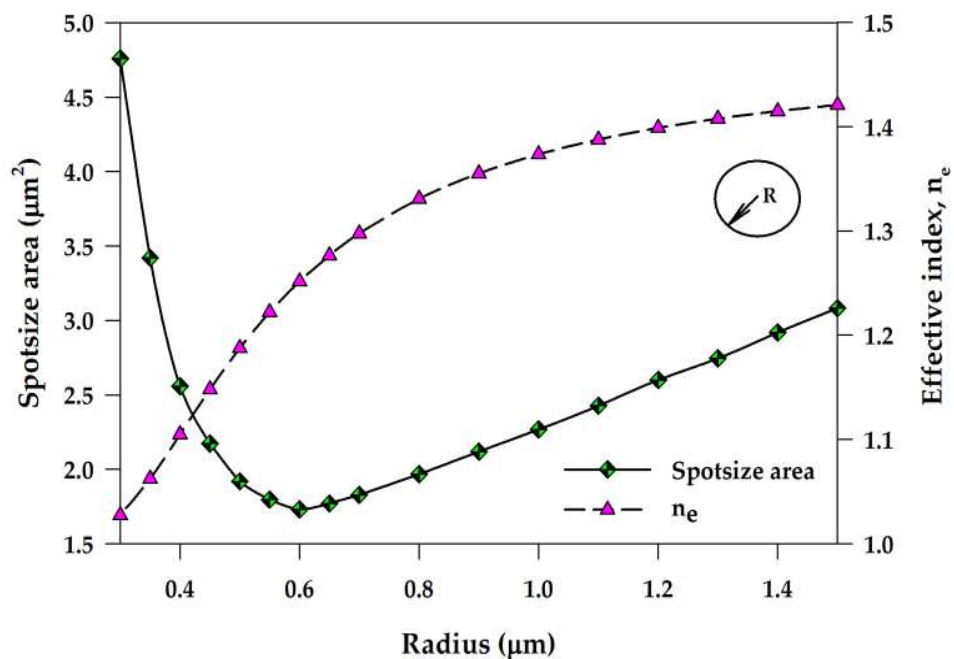
Figure 4.12. Variation of effective index and spot size area with the radius for silica nanowire at \lambda=1.55 \mu\text{m} .
