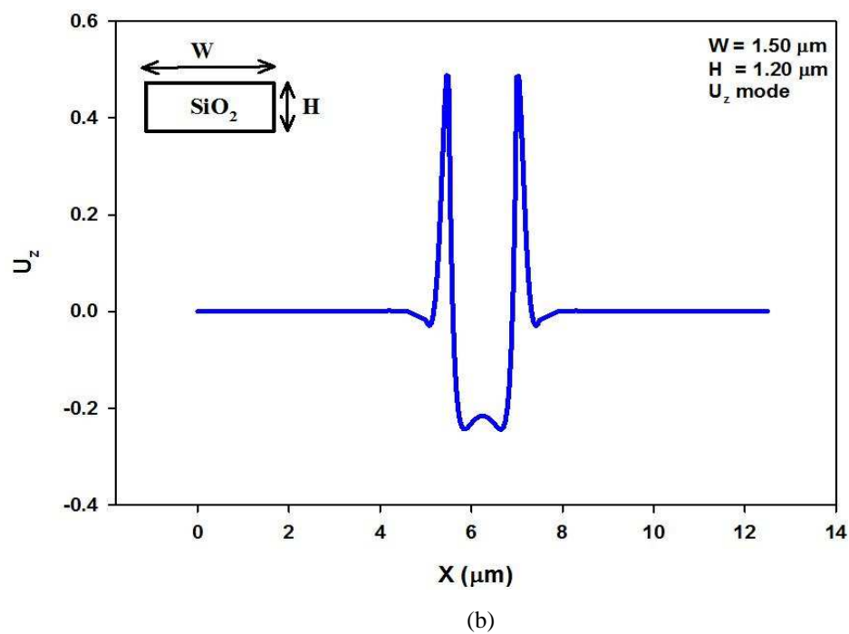
Figure 5.31. The variation of (a) U_y along y -axis and (b) U_z along x -axis of the R1 ( U^y_{12} ) mode at k = 10.0 \mu\text{m}^{-1} .
