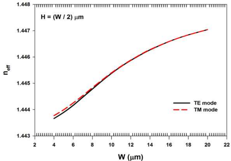
Figure 5.14. The n_{\text{eff}} variation of the quasi-TE and TM modes with the width of the waveguide.
