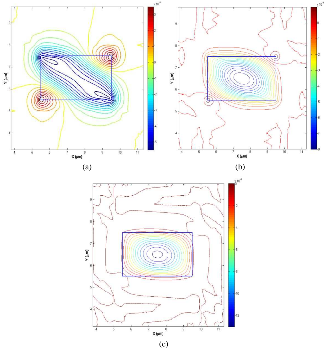
Figure 5.7. The contour plots of U_x displacement vector at (a) k=11 \mu\text{m}^{-1} , (b) k=20 \mu\text{m}^{-1} and (c) k=30 \mu\text{m}^{-1} of the U_{11}^y mode for the H2W4 guide.
