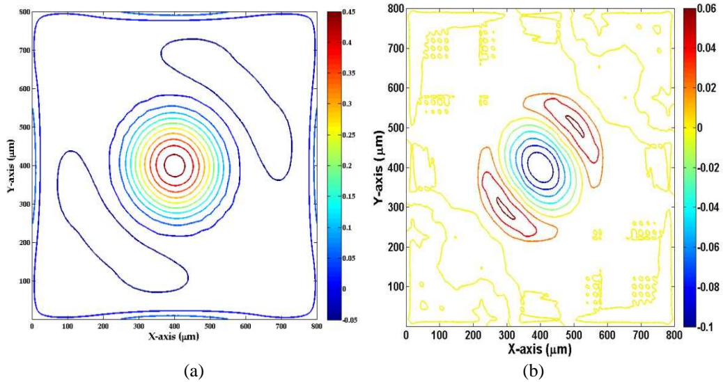
Figure 4.7. U_z distribution of S_{11} at (a) fa=5.838 \mu\text{m.GHz} and (b) fa=28.374 \mu\text{m.GHz} of the R_{01} mode.
