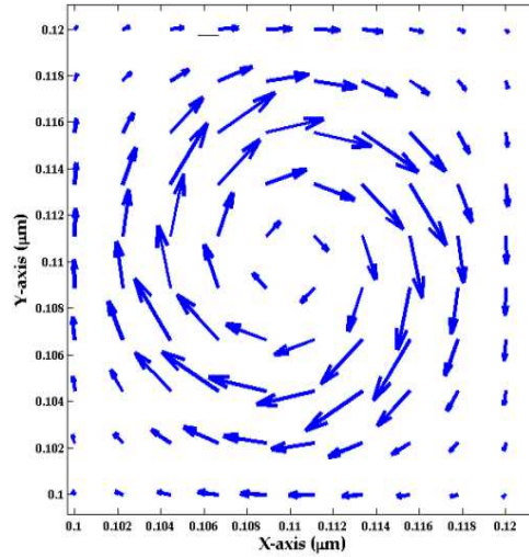
Figure 3.18. The vector fields U_t = \bar{U}_x + \bar{U}_y of the torsional mode at k=200 \text{ m}^{-1} .
