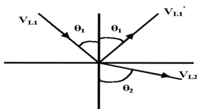
Figure 2.4. The diagram of reflected and refracted longitudinal ( \mathbf{V}_L ) wave.
