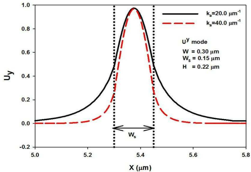
Figure 6.5. Variation of the displacement vector U_y along the x -axis for the U^y mode in a slot waveguide at k=20.0 \mu\text{m}^{-1} and k=40.0 \mu\text{m}^{-1} .
