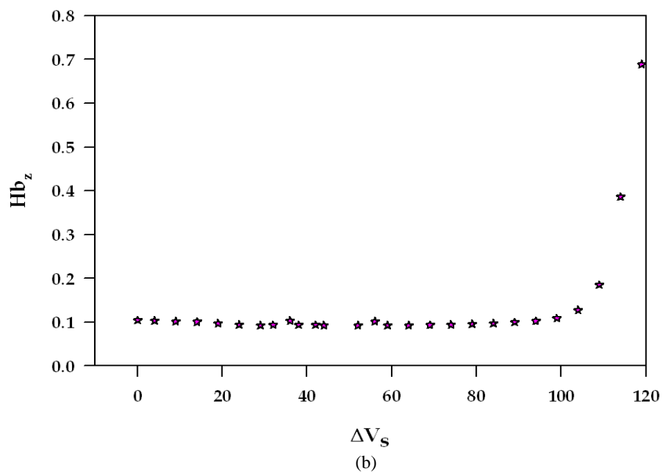
Figure 4.10. (a) Variation of phase velocity and (b) Hybridness of the L_{01} mode with the \Delta V_S from Case 2.
