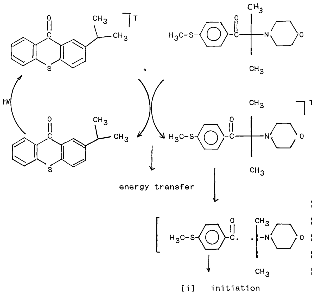
Scheme I Energy-transfer induced \alpha -cleavage of 2-methyl-1-[4-(methylthio)phenyl]-2-morpholino-propan-1-one Irg 907
