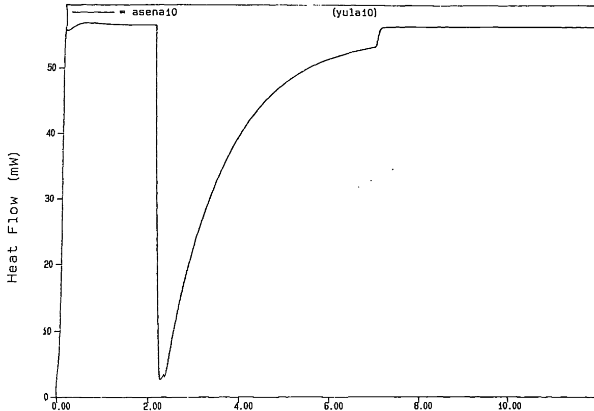
Fig 6.14. DSC trace of photopolymerisation of 2% IRG-651/3% IPM/LA.
