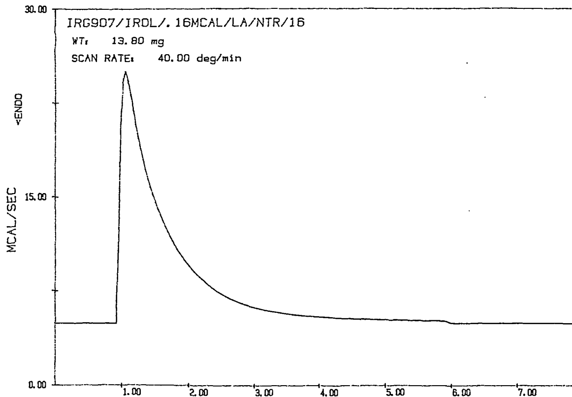
Fig 8.19 DSC trace for photopolymerisation of 2%IRG-907/ 1% S(-)-N-Methyl-1,1-Diphenylprolinol (AA4)/LA in nitrogen.
