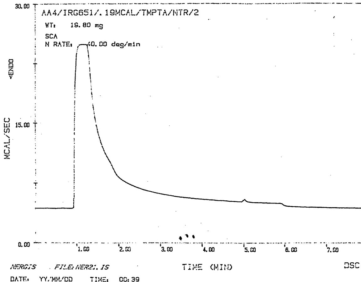
Fig 8.23. DSC trace for photopolymerisation of 2% IRG-651/S(-)-N-Methyl-1,1-Diphenylprolinol (1%) (AA4)/LA in nitrogen.
