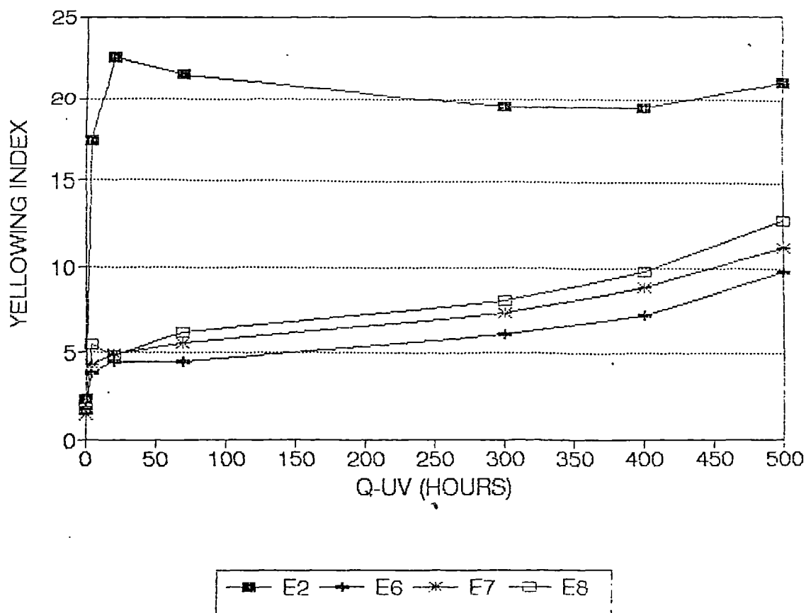
Fig 9.3 The yellowing indices for samples E2, E6, E7 and E8 during Q-UV exposure hours
