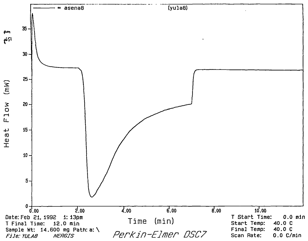
Fig 6.13. DSC trace of photopolymerisation of 2% IRG-651/1% IPM/LA.
