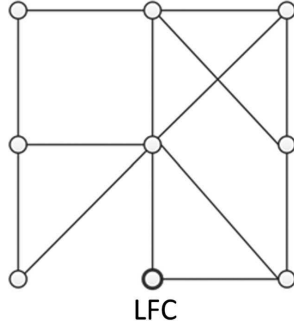
Fig. 2. Randomly built connected cluster.
