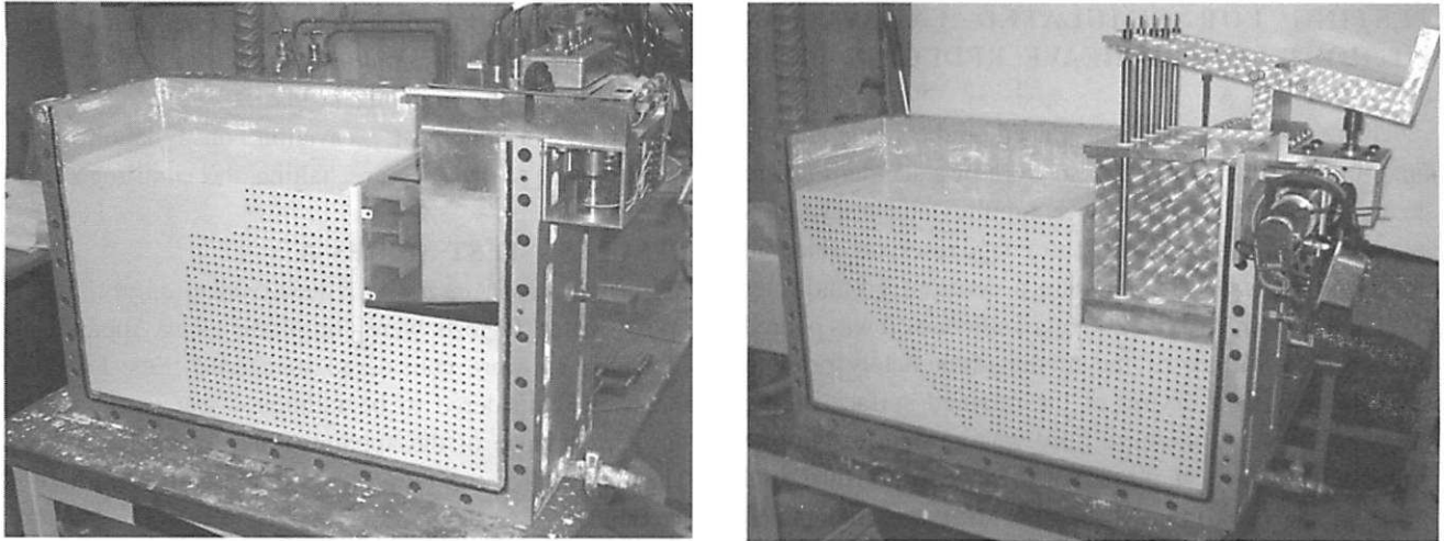
Fig. 16 Completed models prior to placement on the centrifuge a) Unloaded heave reducing piles b) Loaded heave reducing piles
