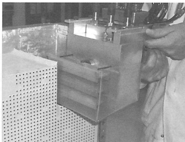
Fig. 3 Walings attached to miniature hydraulics cylinders and mounted in main body of apparatus. Also shown is the polyethylene bag used to contain the heavy fluid for horizontal support of the wall
