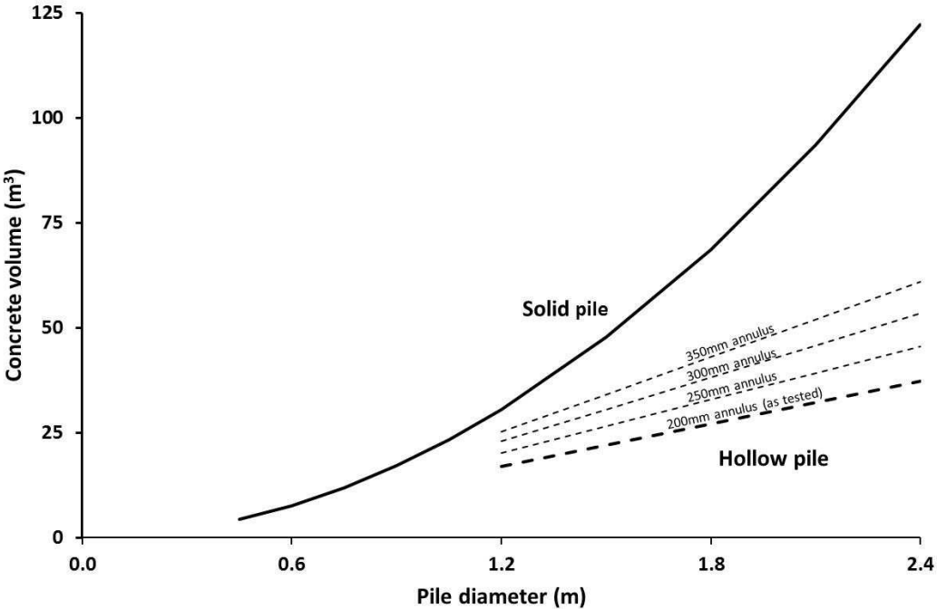
Figure 1 Comparison of concrete volume necessary to construct 27m long solid and hollow piles. A range of annulus thicknesses are shown to demonstrate the reducing benefit as the thickness of the annulus is increased.
