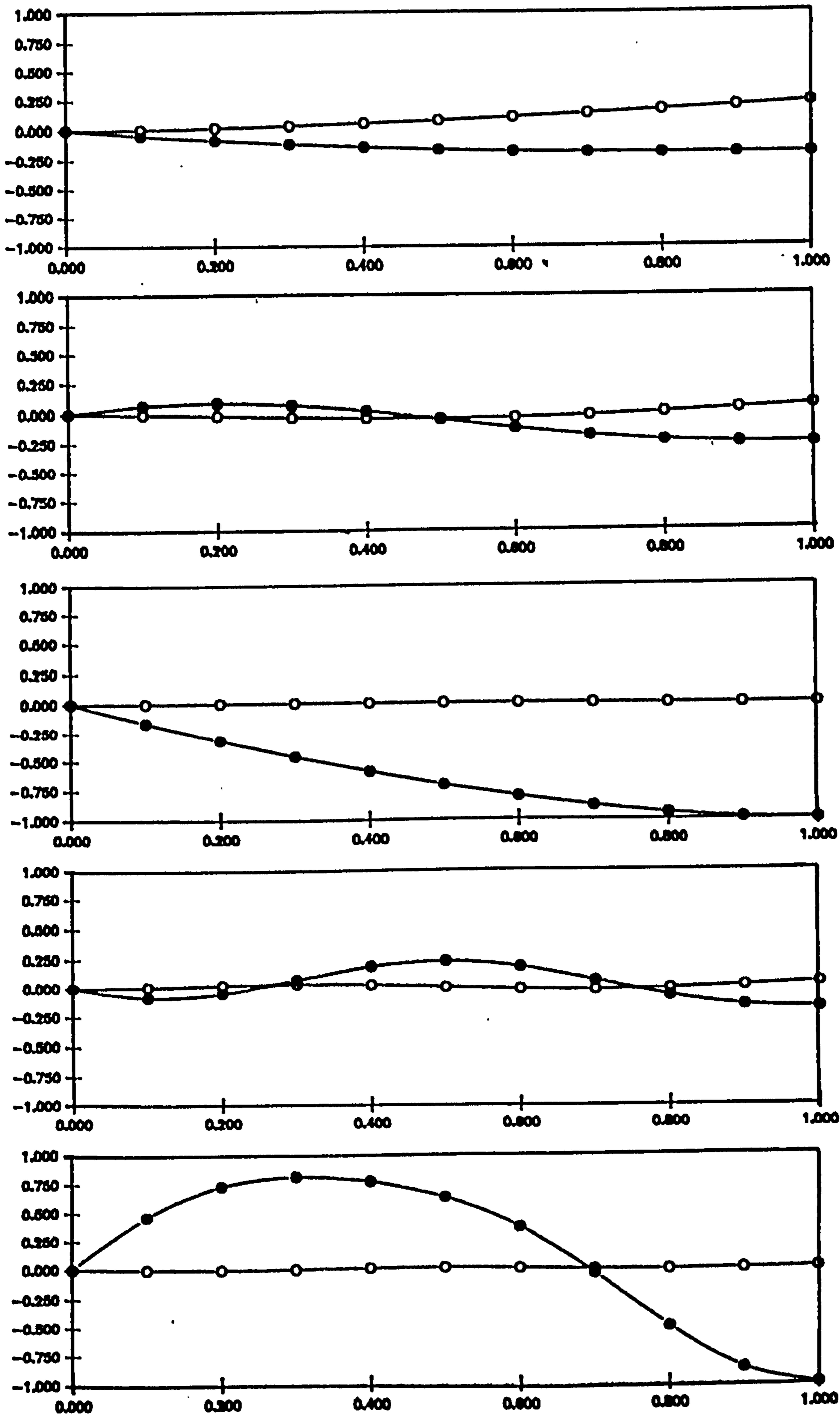
Figure 6.8 Normal mode Shapes for [\pm 45/0] case
