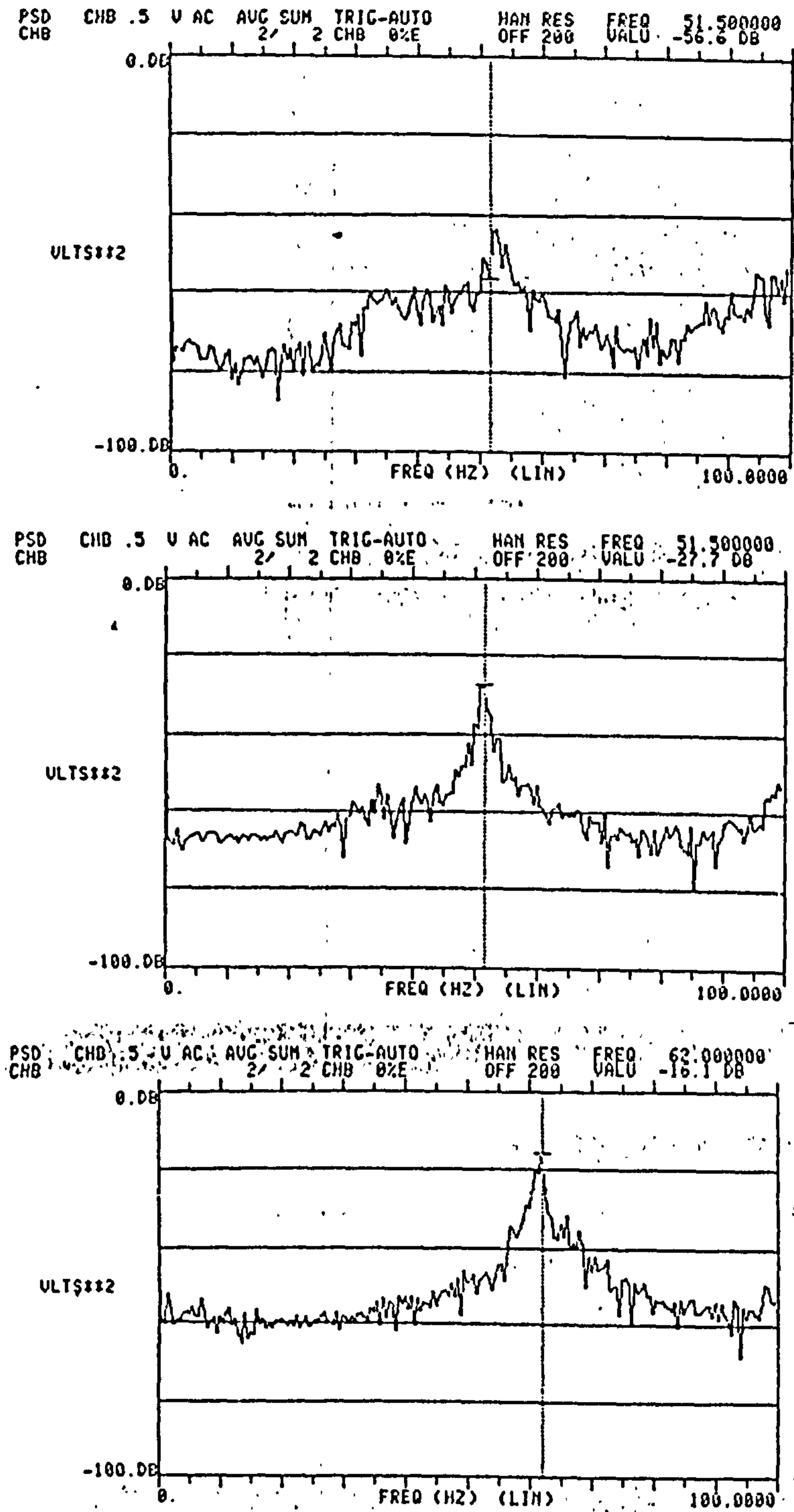
Figure 8.4 PSD of acceleration response plots for [\pm 45/0]_2 composite wing with 0^\circ sweep (i) 40.23 m/s, (ii) 43.83 m/s (iii) 47.22 m/s
