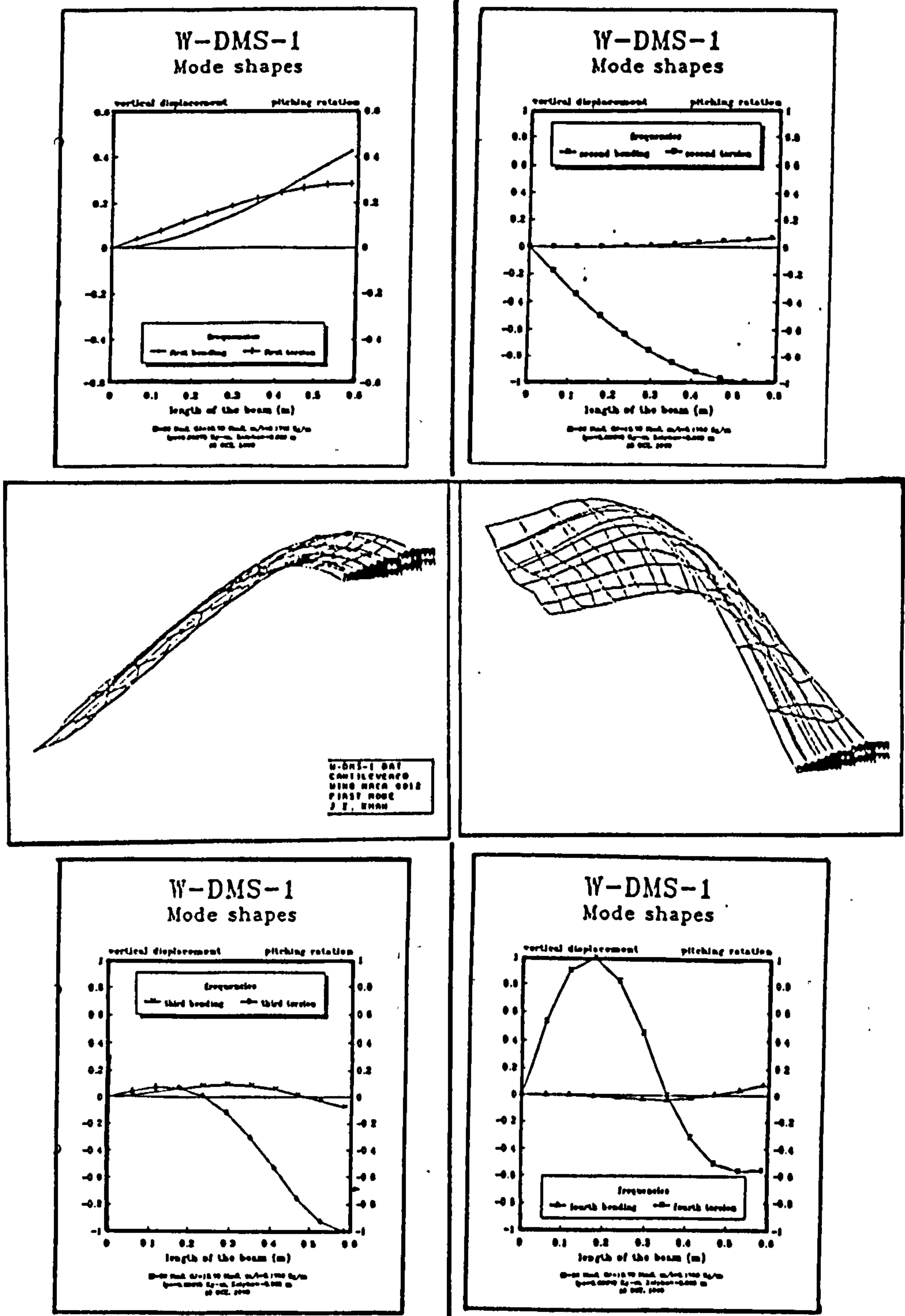
: Figure 7.26 Representative normal mode shapes for thin-walled composite closed sections compared with experimental results
