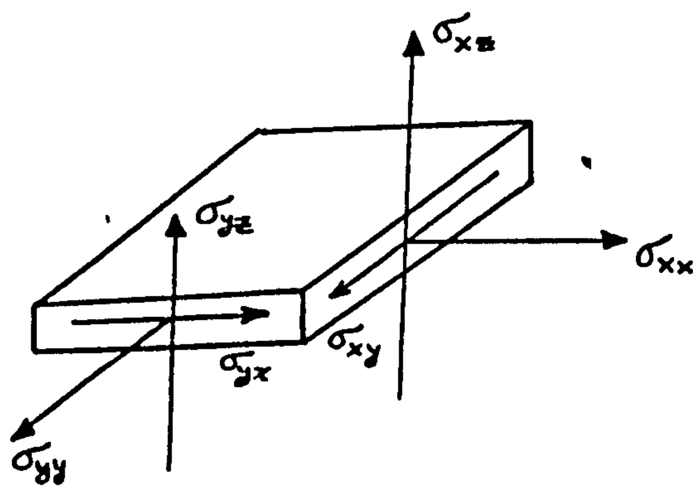
Figure 4.2(b) Stresses
