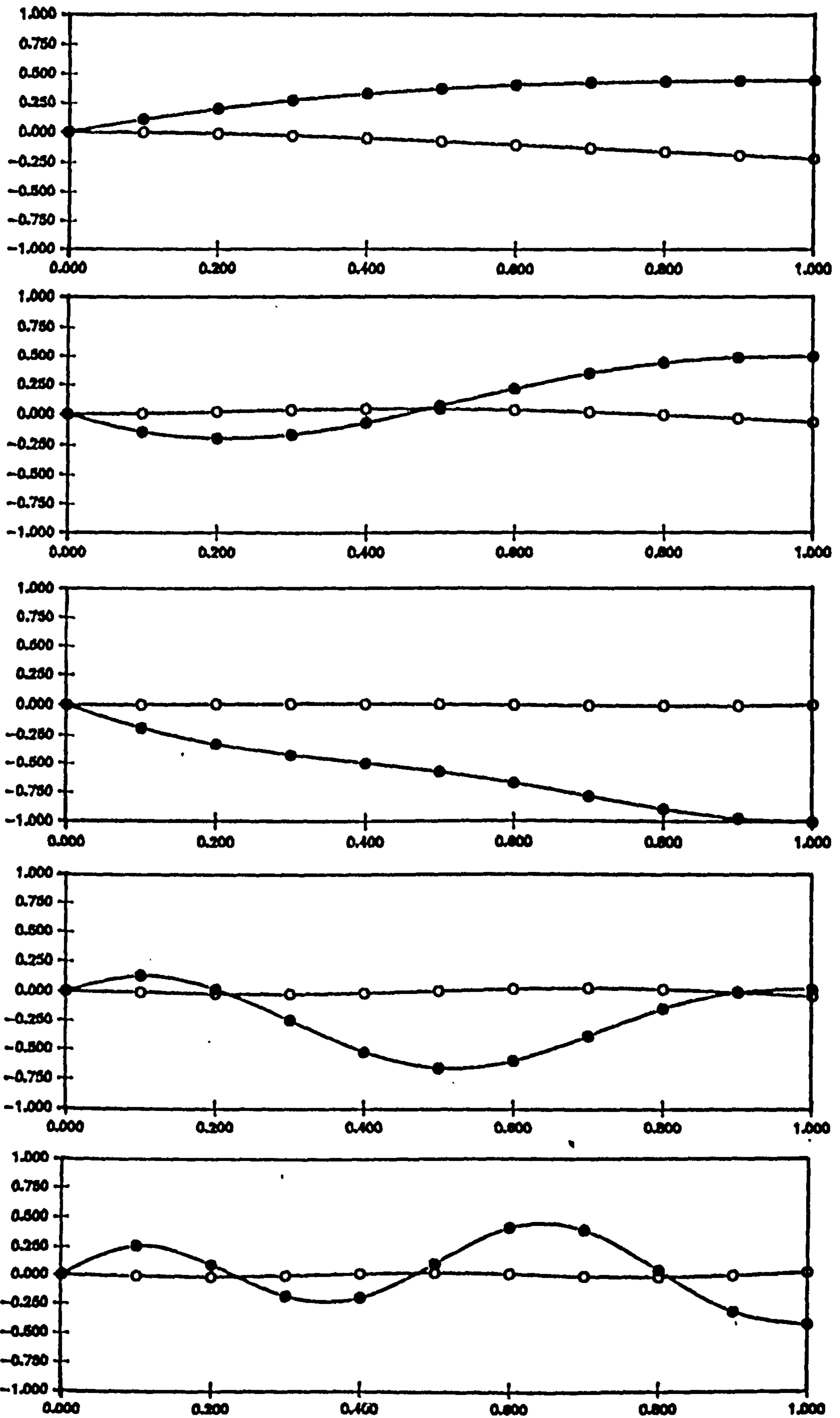
Figure 6.9 Normal mode Shapes for [+45 2 /0] case
