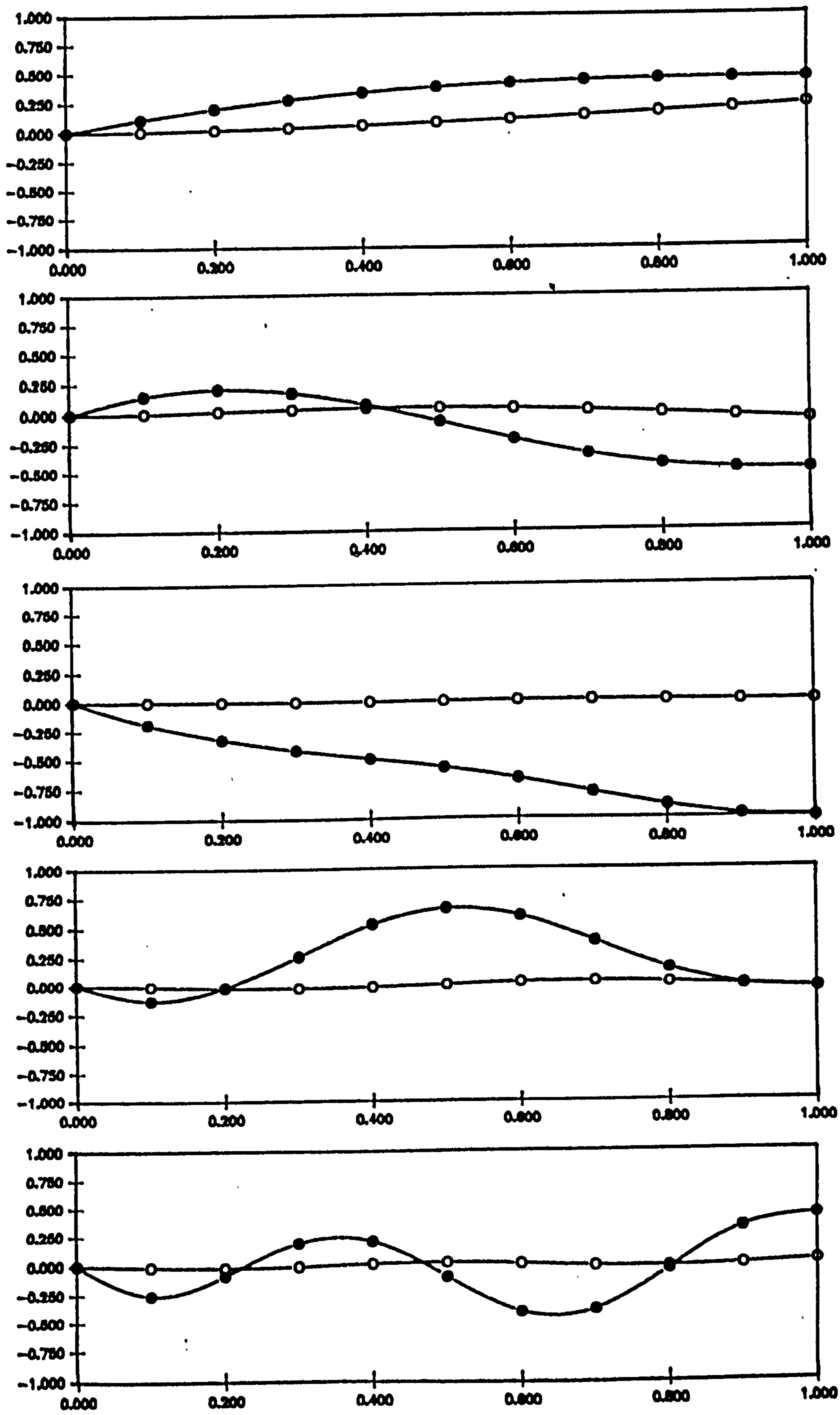
Figure 6.10 Normal mode Shapes for [-45^{\circ}/0] case
