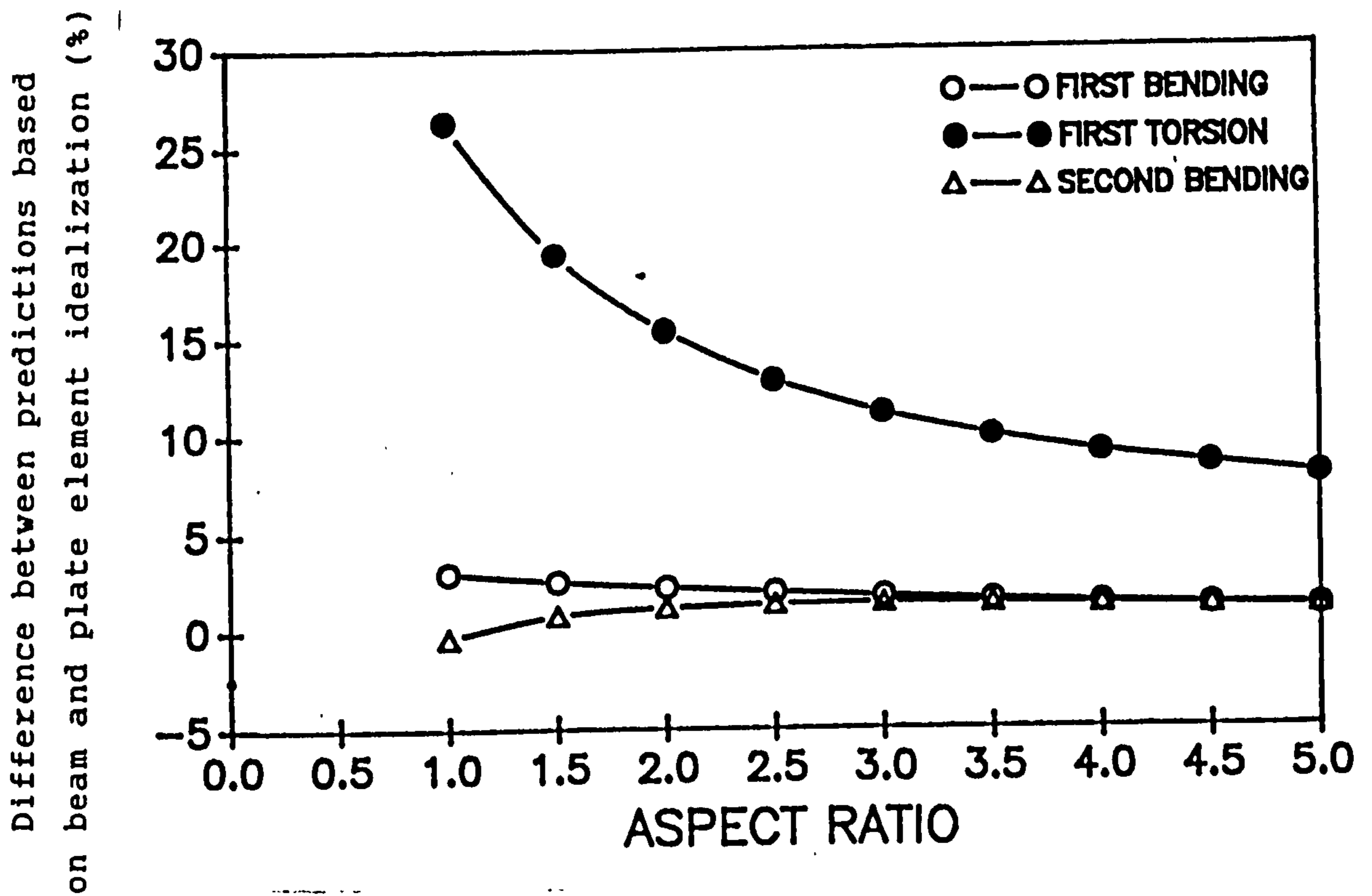
Figure 6.3 Effect of aspect ratio on the accuracy of calculation of natural frequencies of a plate structure using beam element idealization.
