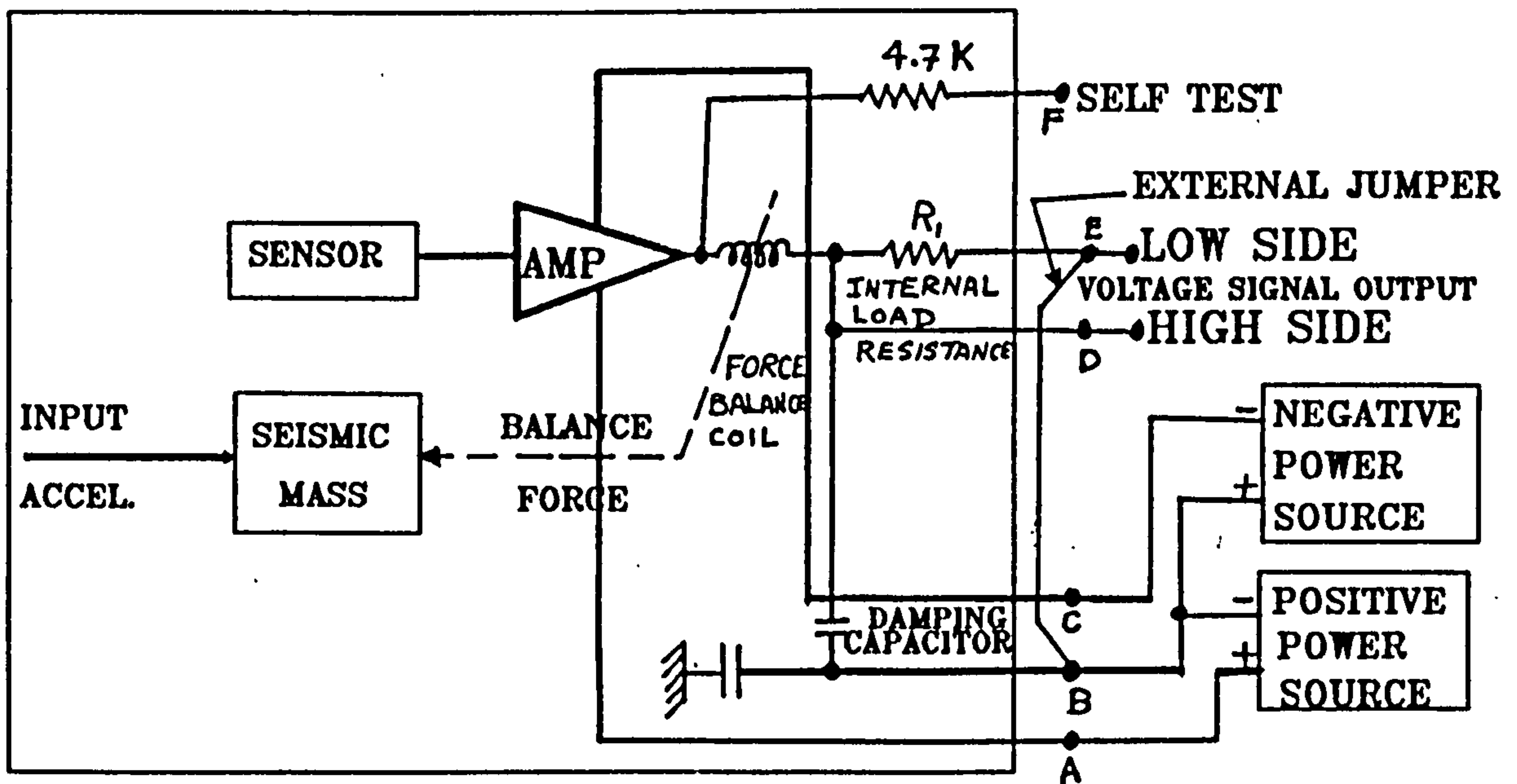
FIG. 5.2 CIRCUIT DIAGRAM
