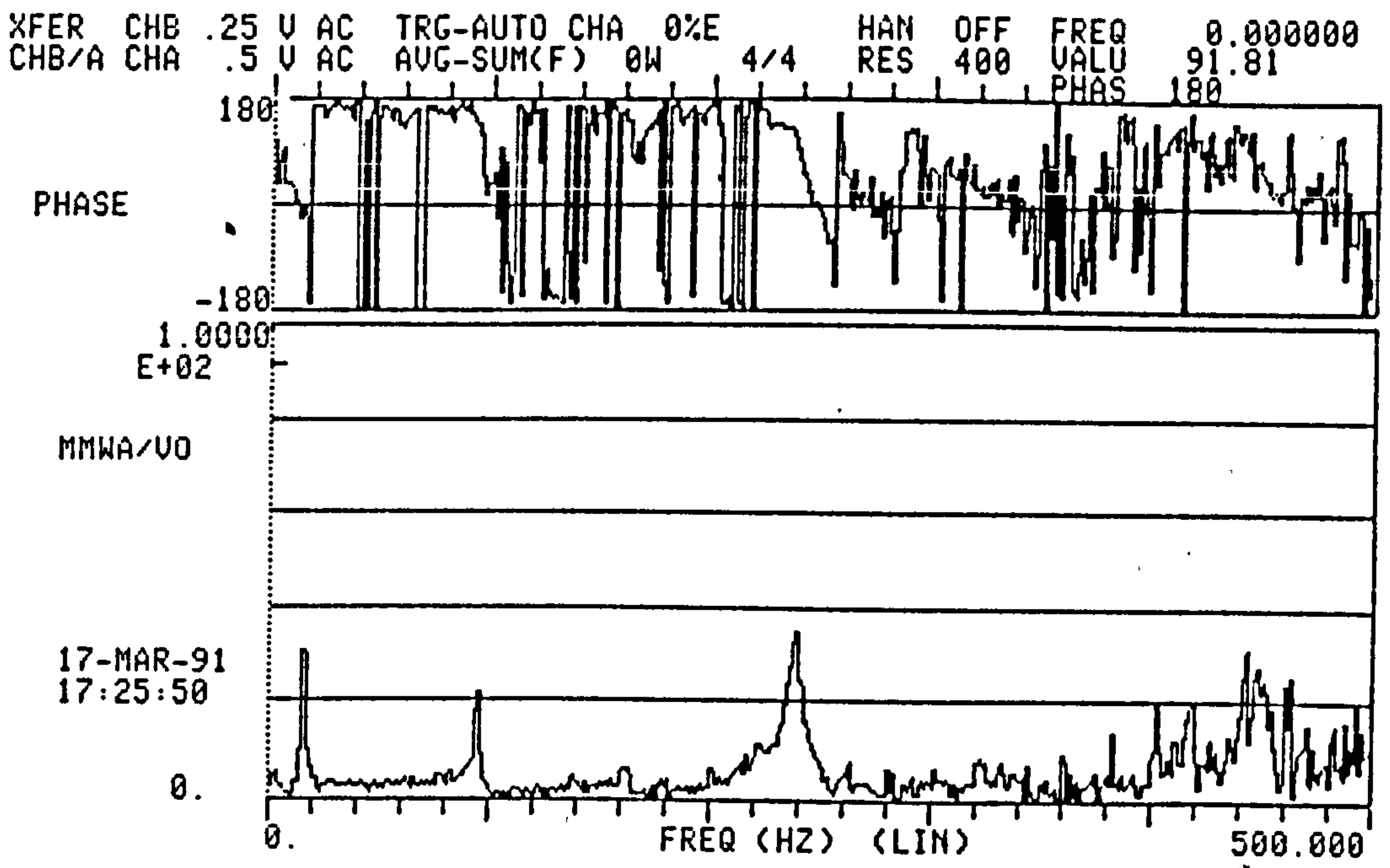
Figure 7.24b Frequency Response plot for W-DMS-3A wing when excited at 3/4 of the length from the root.
