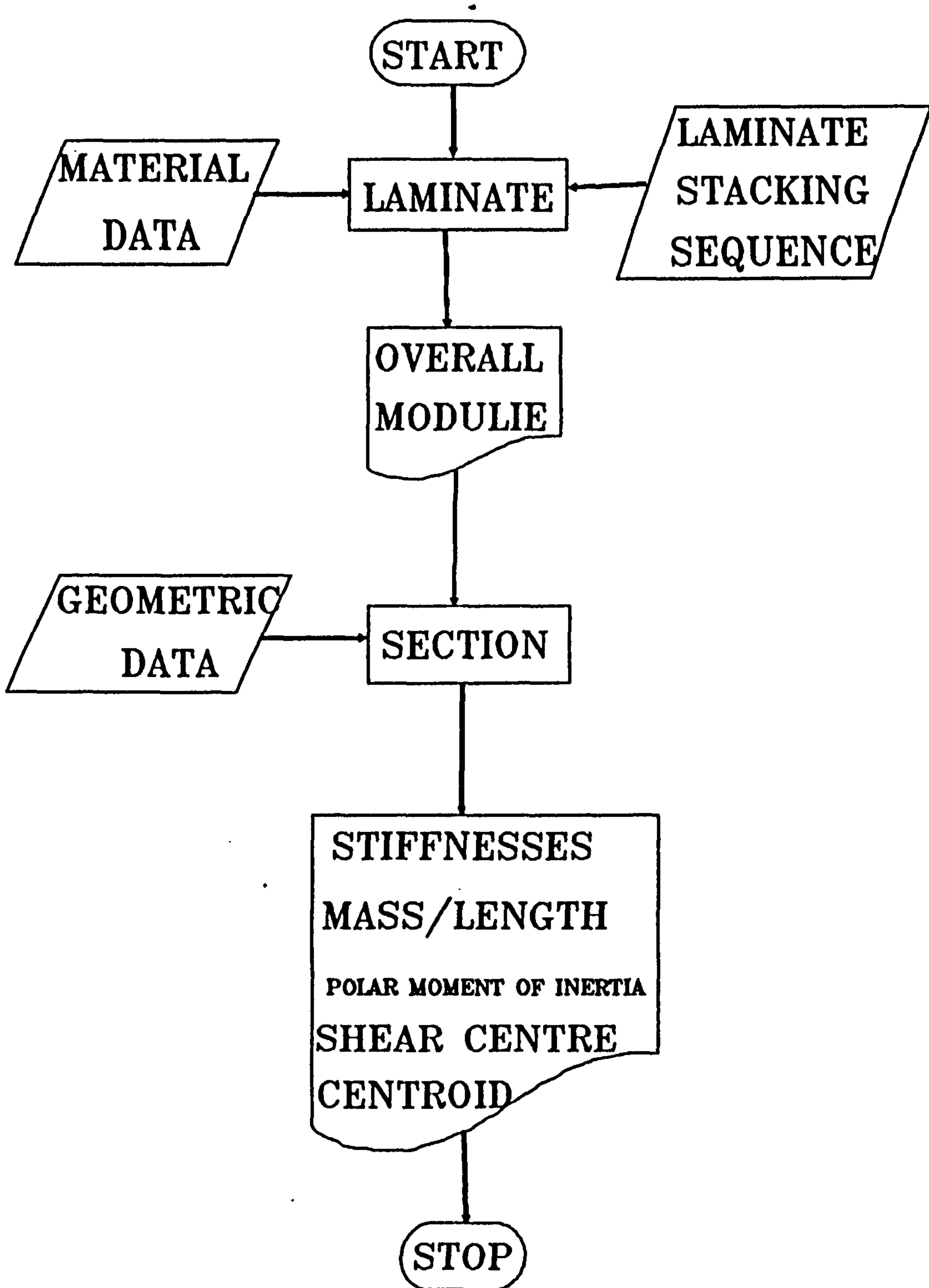
FIG. 4.8 FLOW CHART FOR COMPUTER PROGRAM "KSTIF"
