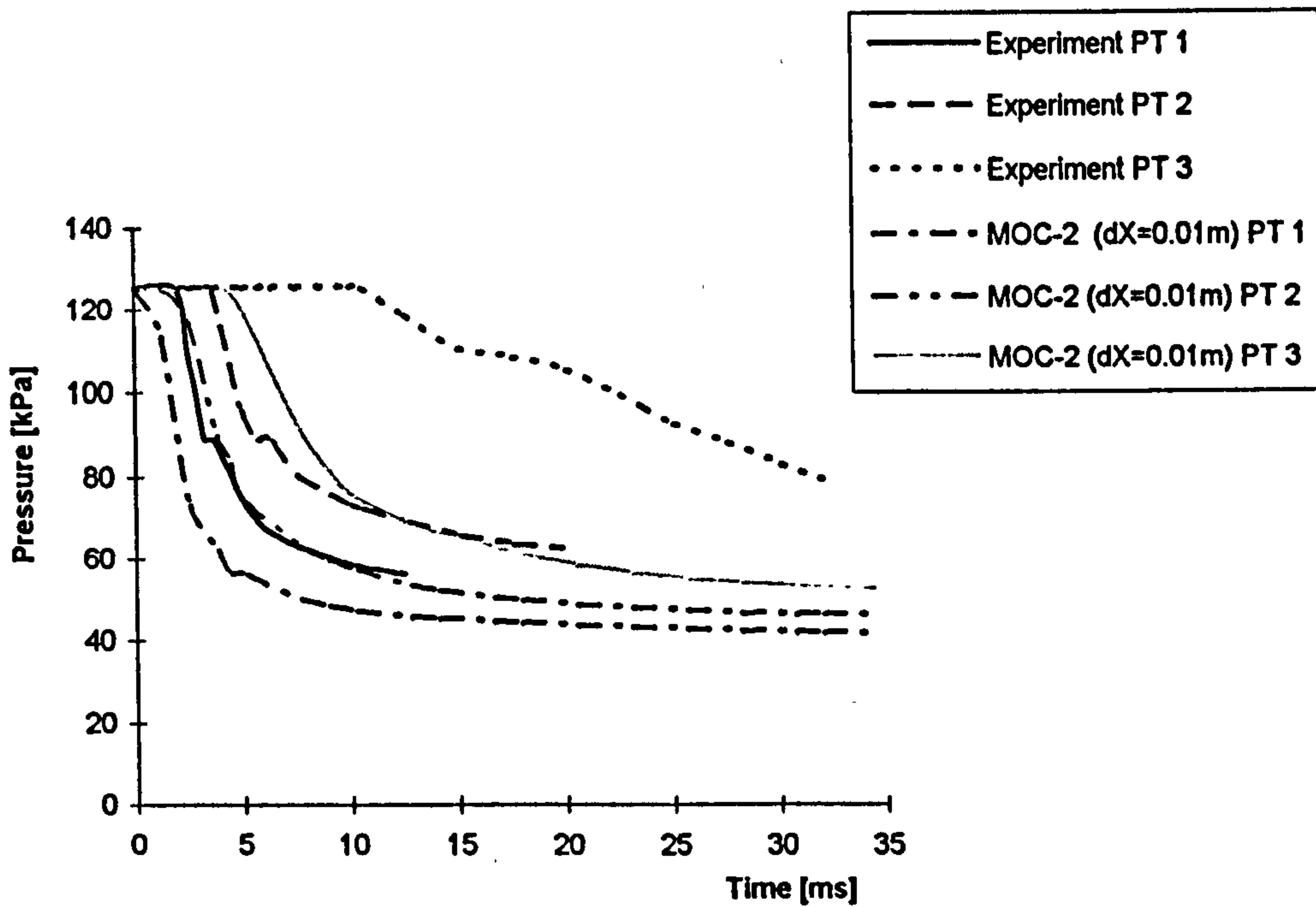
Fig. 6.18 p-t Curves for British Gas Test BGT3 Comparison with Second-order Method of Characteristics Prediction ( dX=0.01m )
