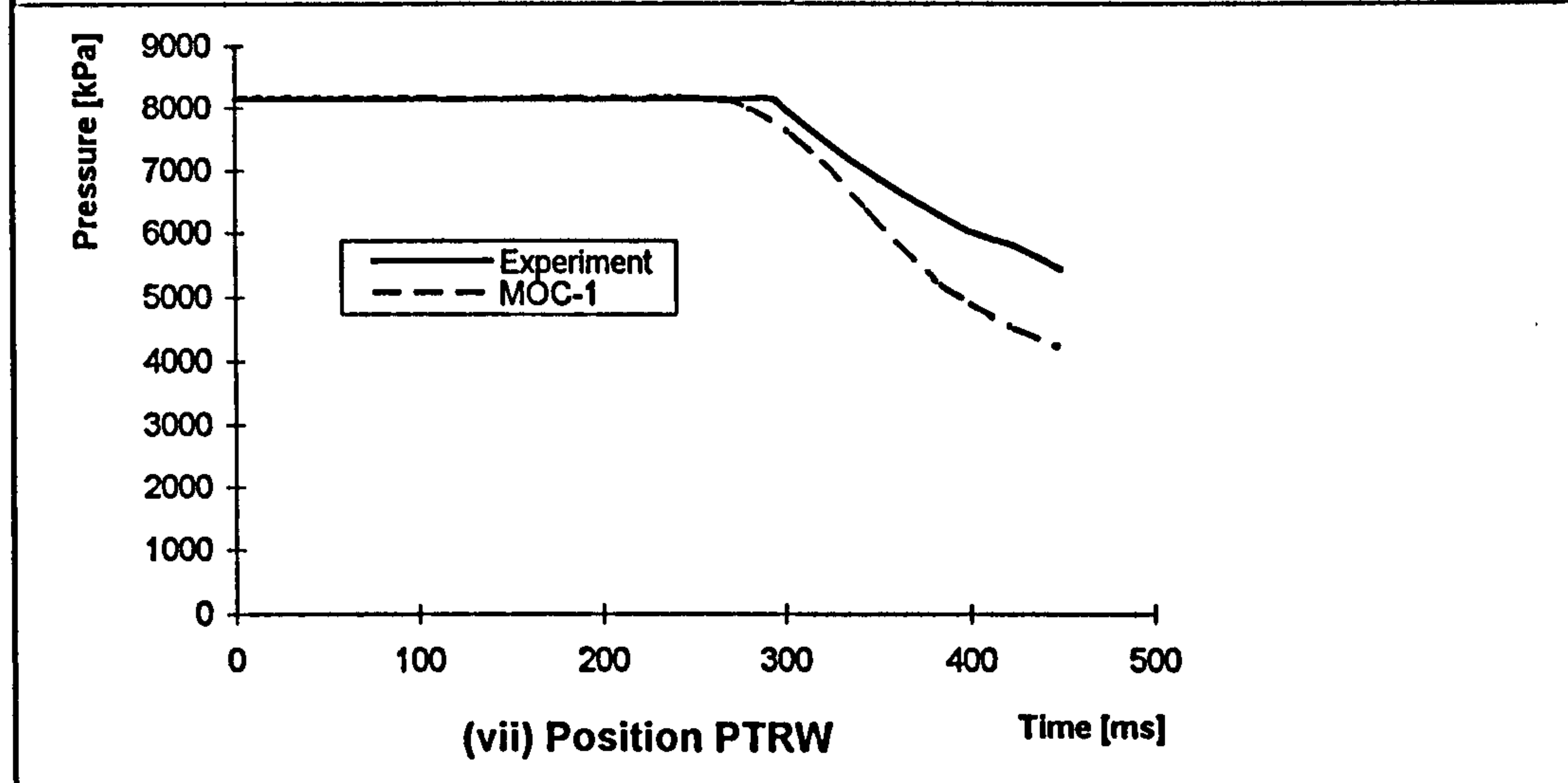
Fig. 6.6 p-t Curves for Foothills Test NABTF7 West Comparison With First-order Method of Characteristics Predictions
