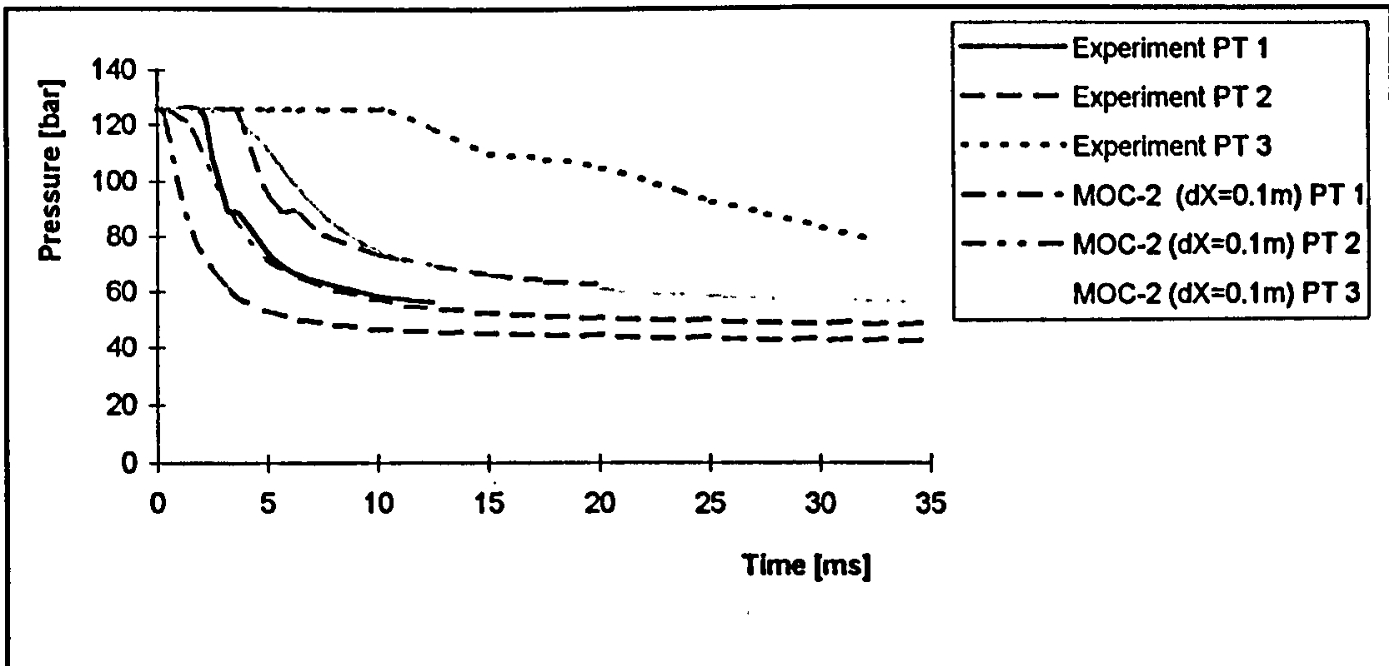
Fig. 6.19 p-t Curves for British Gas Test BGT3 Comparison with Second-order Method of Characteristics Predictions (dX=0.1m)
