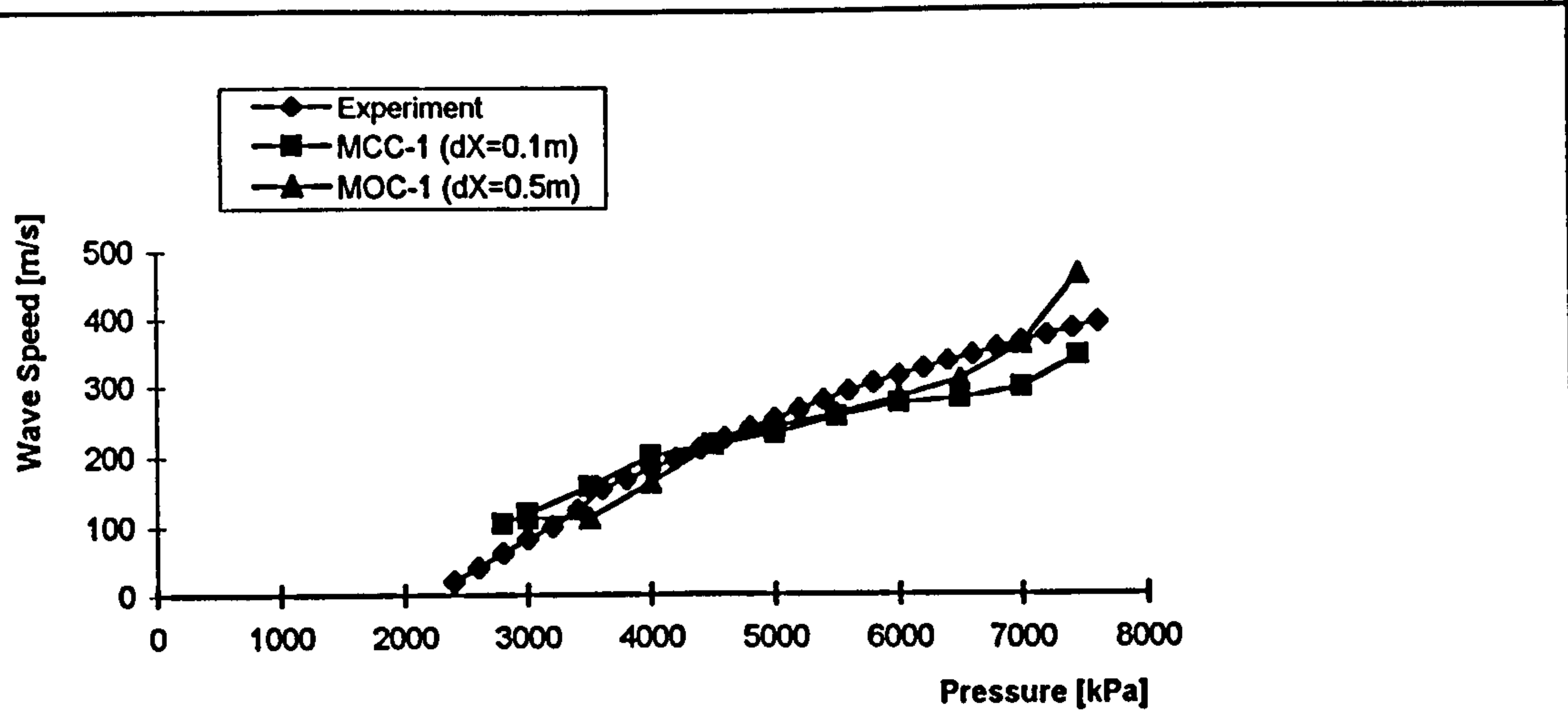
Fig. 6.5 Pressure Wave Propagation Speed for Foothills Test NABTF1 East
