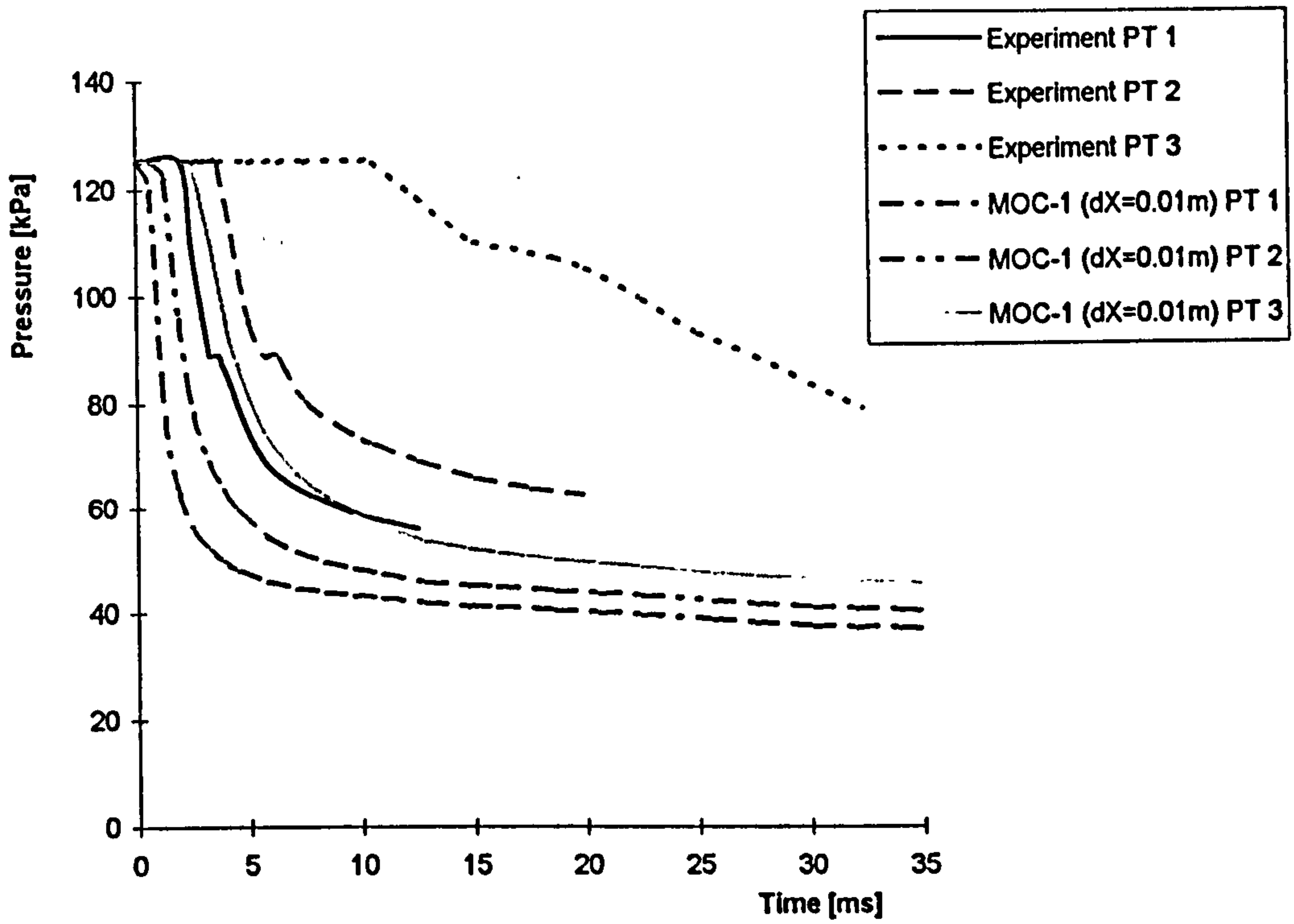
Fig. 6.17 p-t Curves for British Gas Test BGT3 Comparison With First-order Method of Characteristics Predictions ( dX=0.01m )
