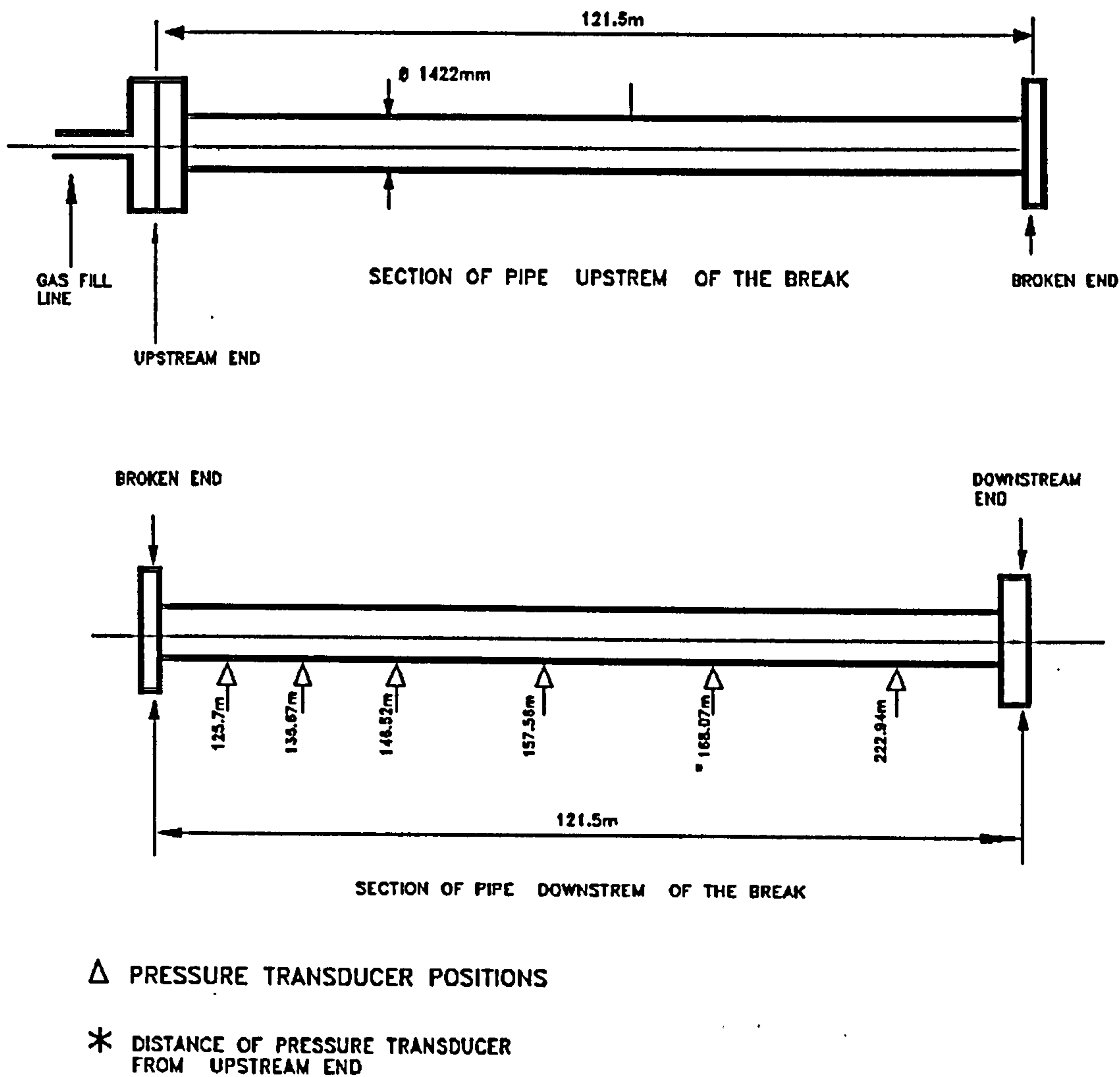
Fig. 6.1 Schematic of Foothills Test NABTF1
