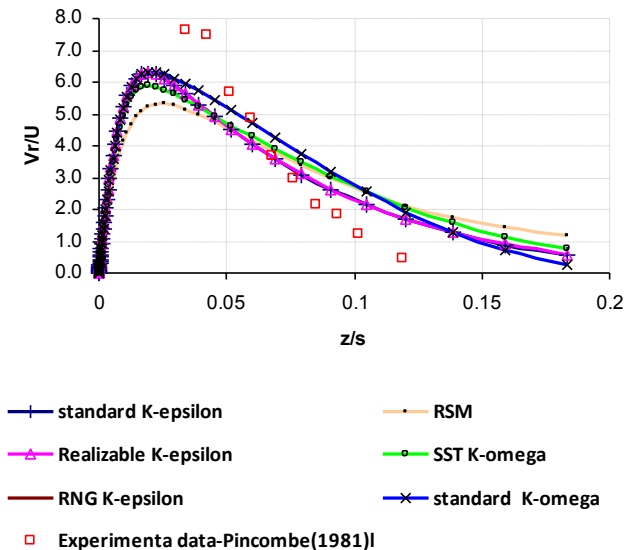
Figure 5. Validation Test Case No. 1. Axial Variation of radial velocity at r/b=0.833 using Different Turbulence Models and Comparison with Experimental Data.
