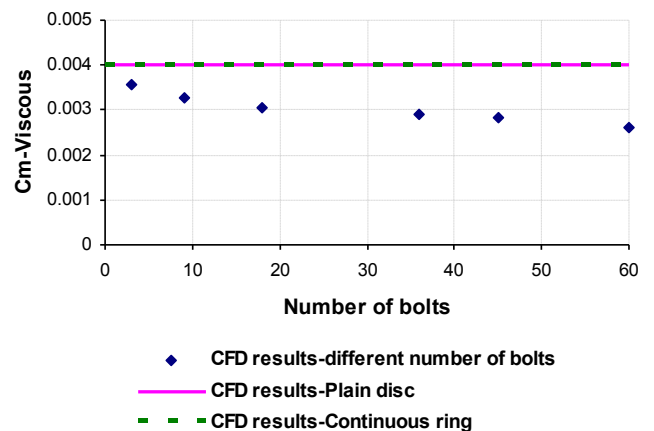
Figure 18 Variation of Moment Coefficient due to Skin Friction with Number of Bolts, Re = 6.8 \times 10^6 and C_w = 10^5 ( \lambda_T = 0.35 ).
