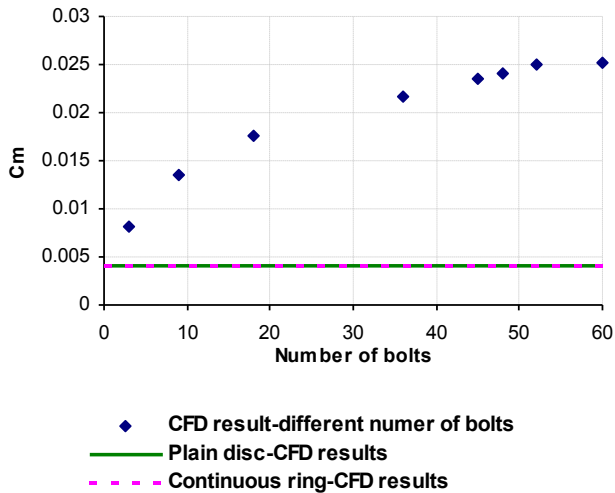
Figure 16. Predicted Variation of Moment Coefficient with Number of Bolts, N for Re = 6.8 \times 10^6 , C_w = 10^5 ( \lambda_T = 0.35 ).
