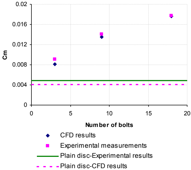
Figure 15. Variation of Moment Coefficient with Number of Bolts N . Comparison Between Numerical and Experimental Results for 3, 9 and 18 bolts and also a plain disc: Re = 6.8 \times 10^6 , C_w = 10^5 ( \lambda_T = 0.35 ).
