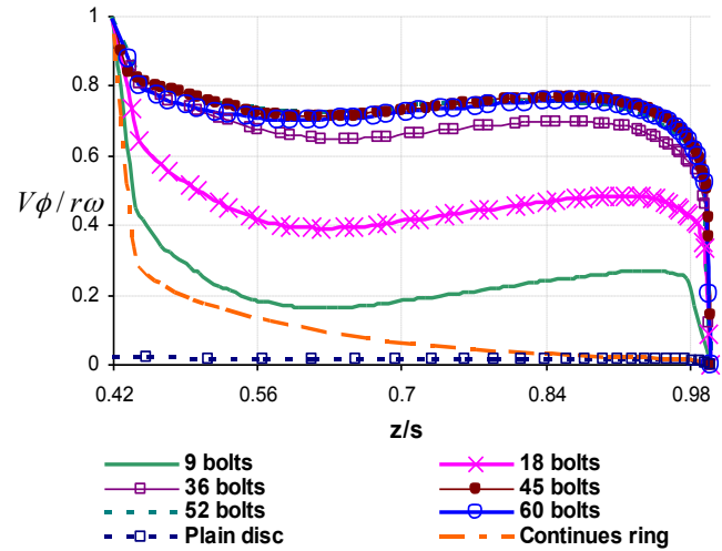
Figure 17. Predicted Axial Variation of Dimensionless Tangential Velocity at r/b = 0.9 , Re = 6.8 \times 10^6 and C_w = 10^5 ( \lambda_T = 0.35 ).
