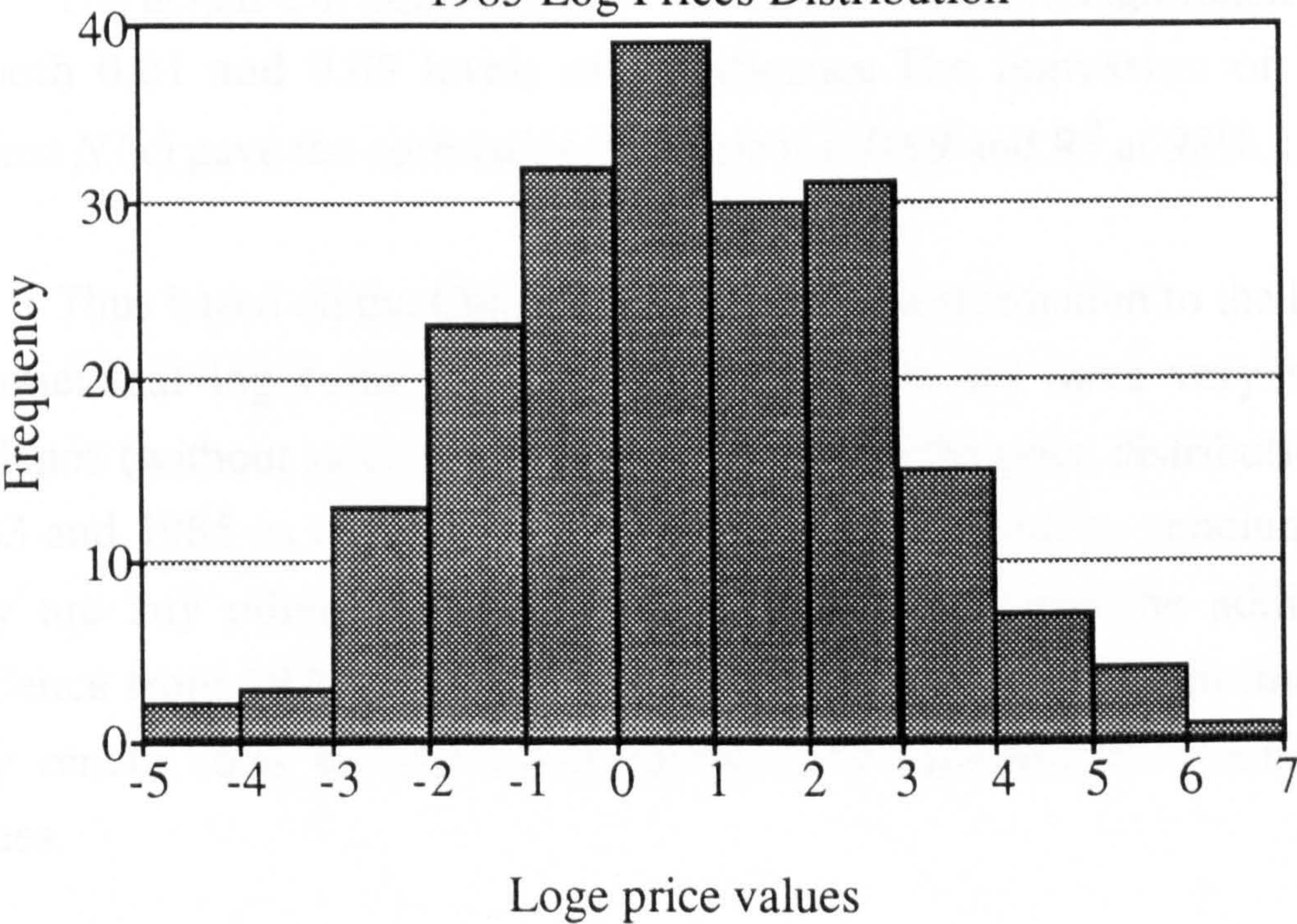
Figure 6.24 1985 Log Prices Distribution
