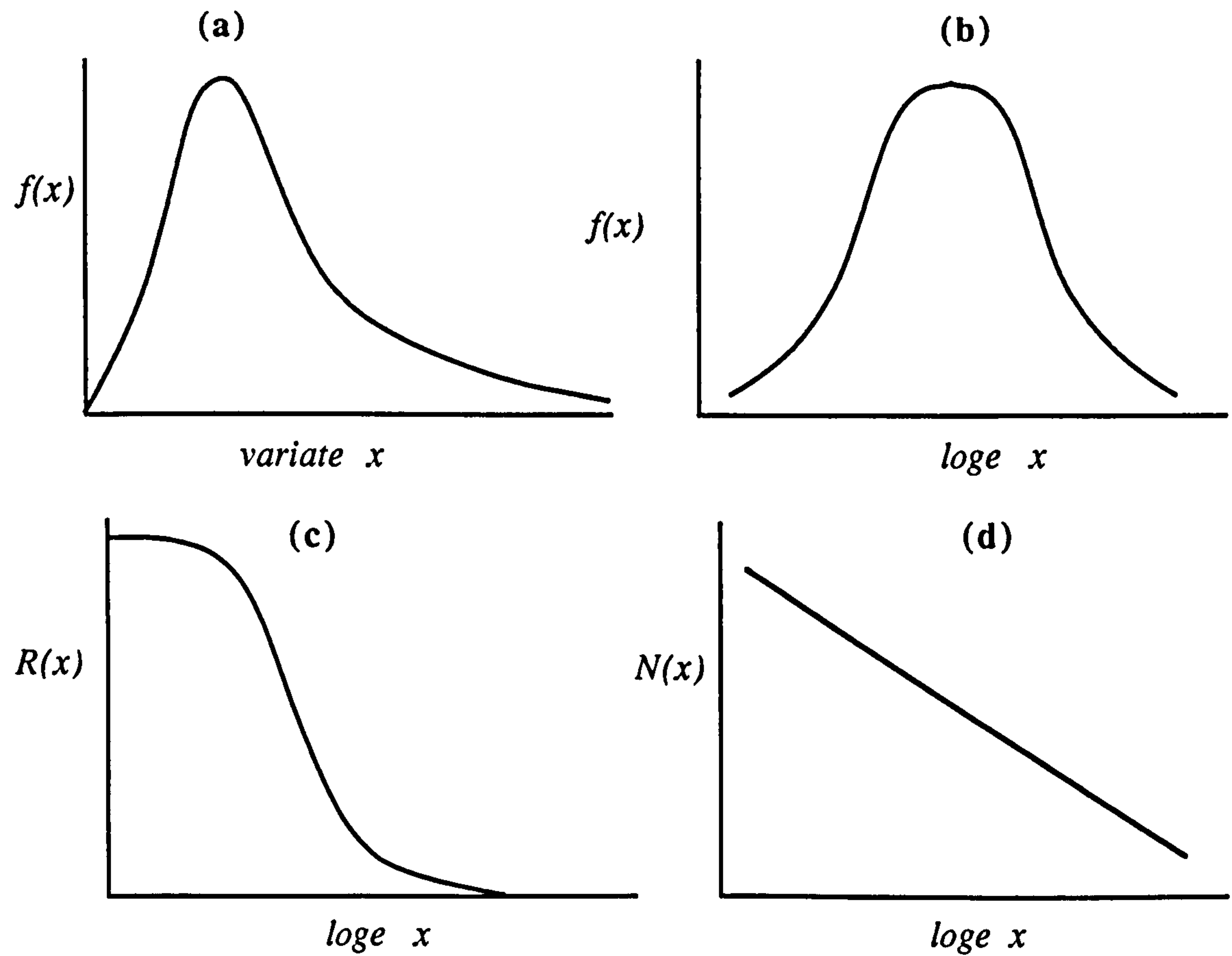
Figure 1.4 Lognormal transformation
