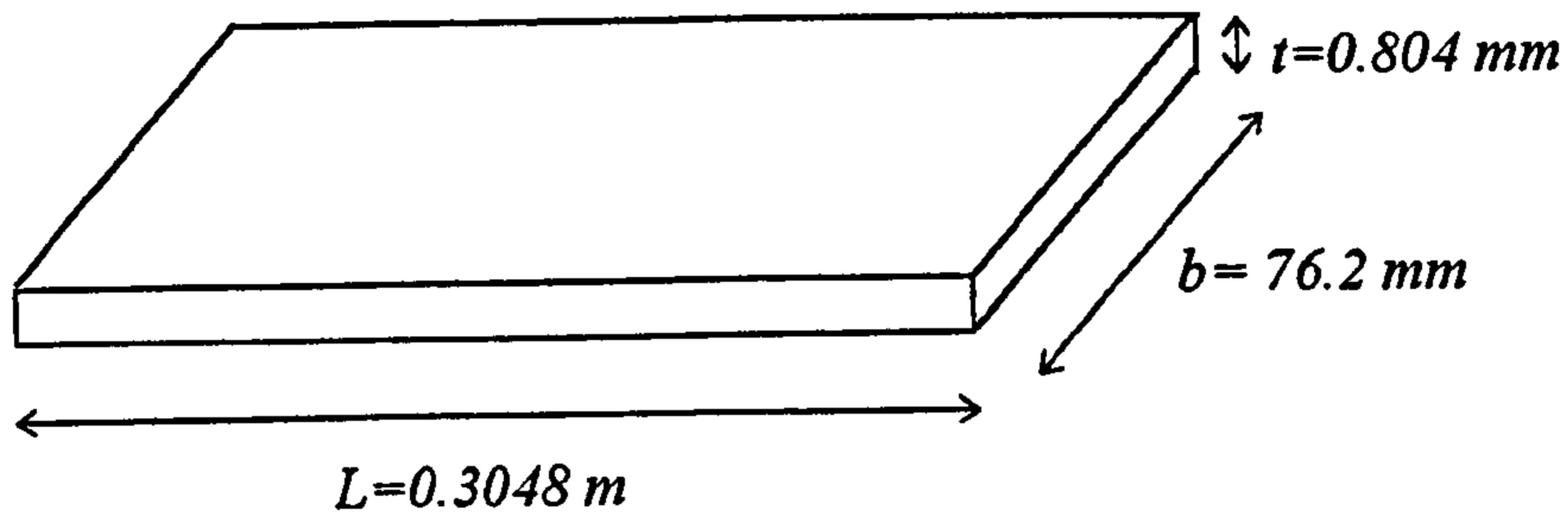
Figure 3-1(a) Configuration of the laminated flat beam.
