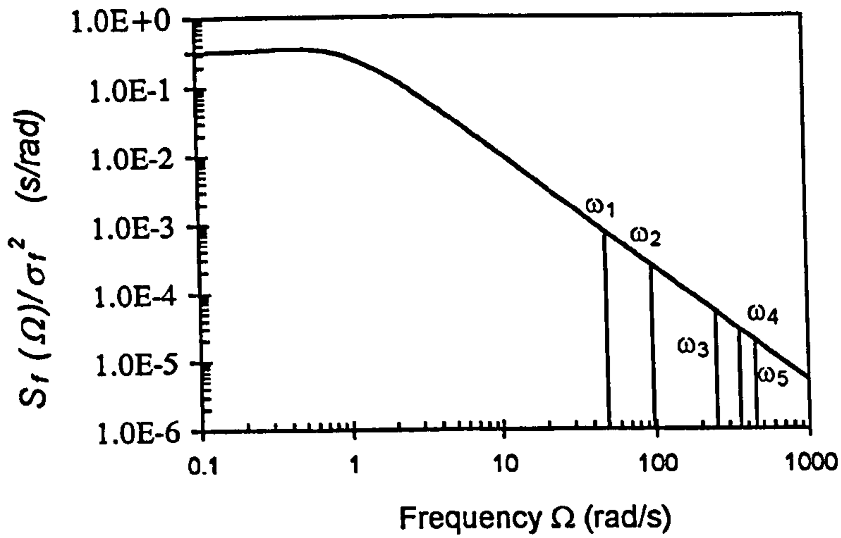
Figure 7-12. The von Karman PSD function ( L_p/V=1 )
