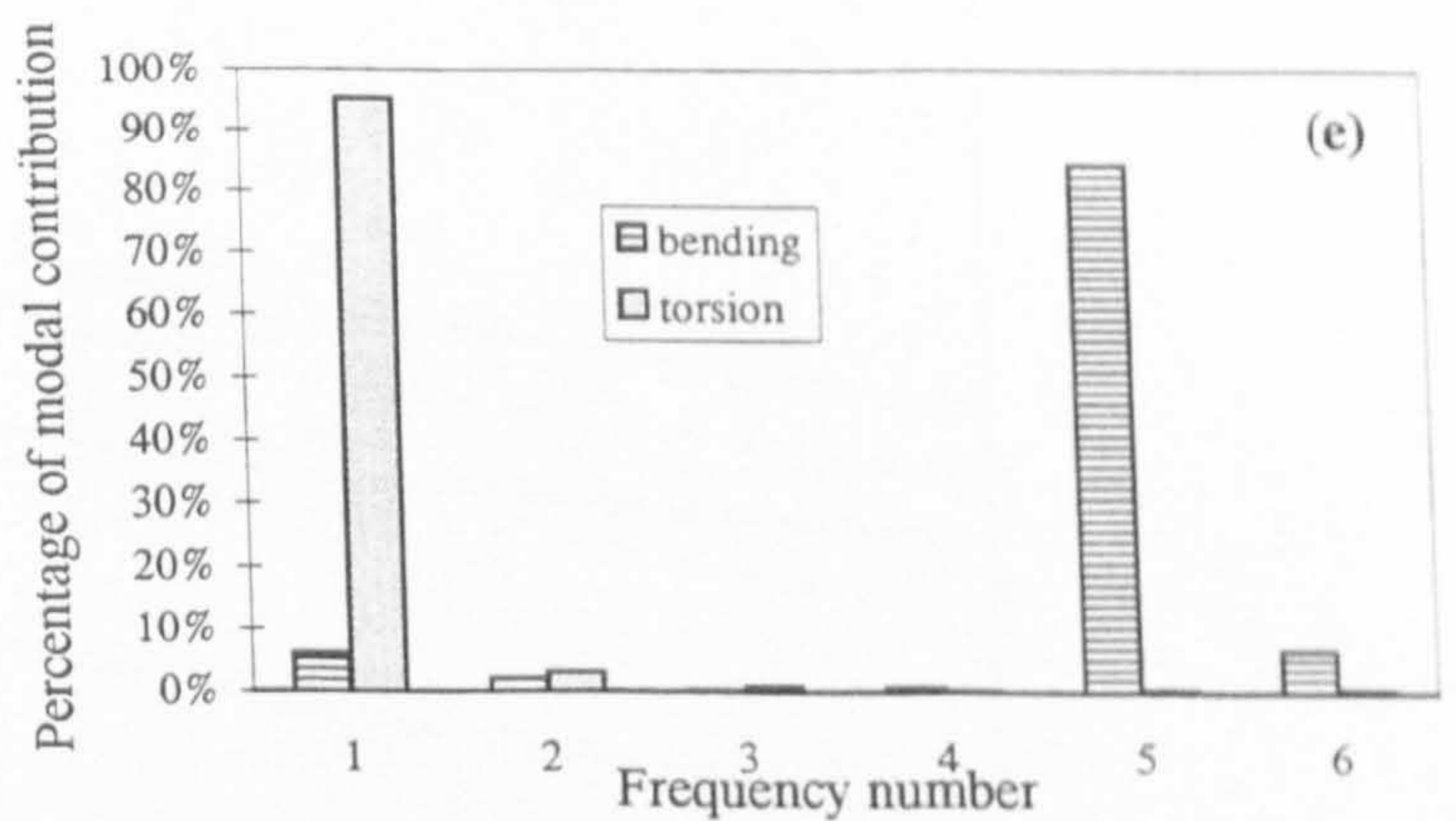
Figure 7-27. Significance of generalised mass in the dynamic response characteristics of a bending-torsion coupled concrete beam with a channel cross-section (Bercin and Tanaka, 1997).
