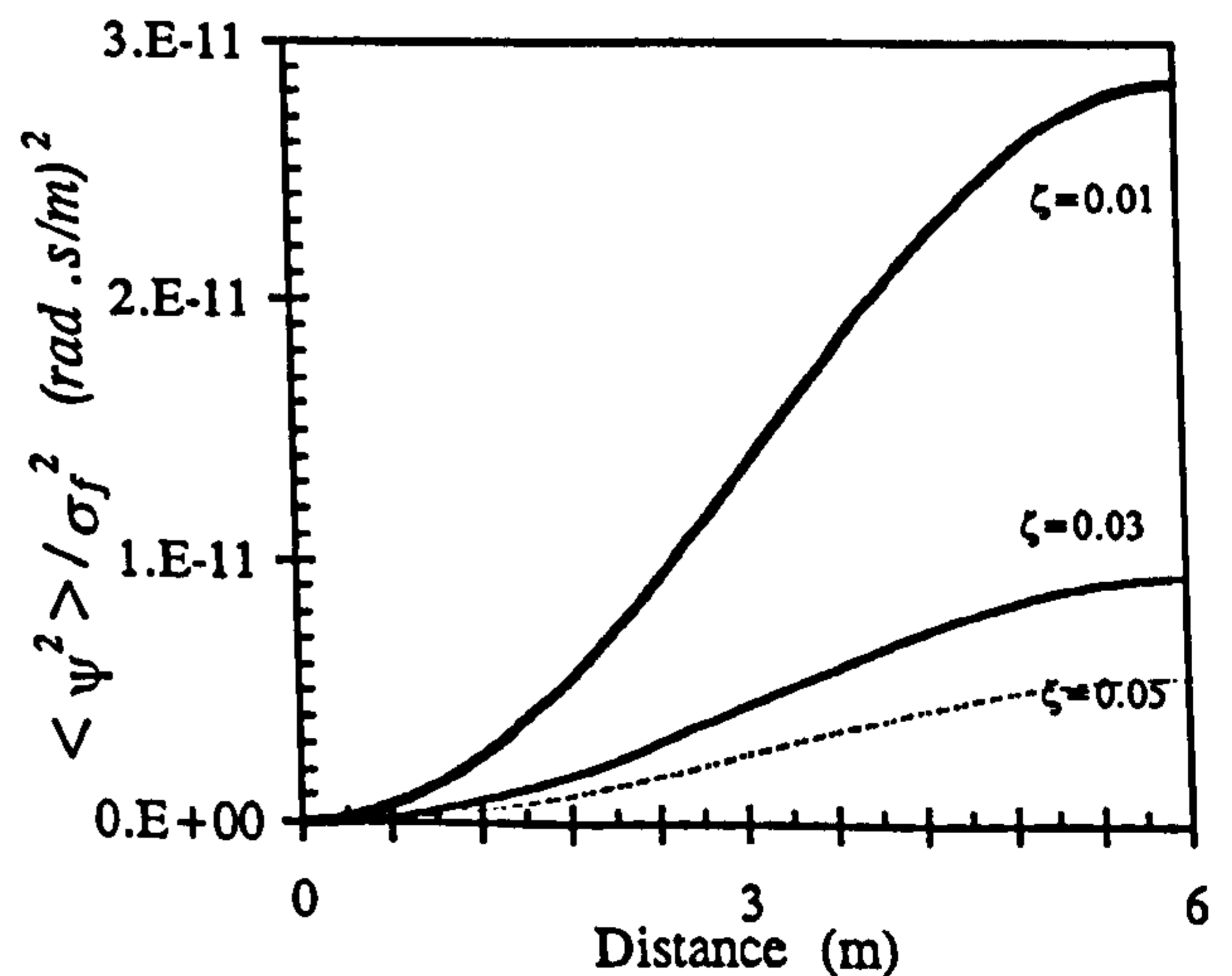
Figure 7-16. Variation of the mean square value of the torsional rotation along the Goland wing (C-F) for different damping coefficients ( L_p/V = 10 ).
