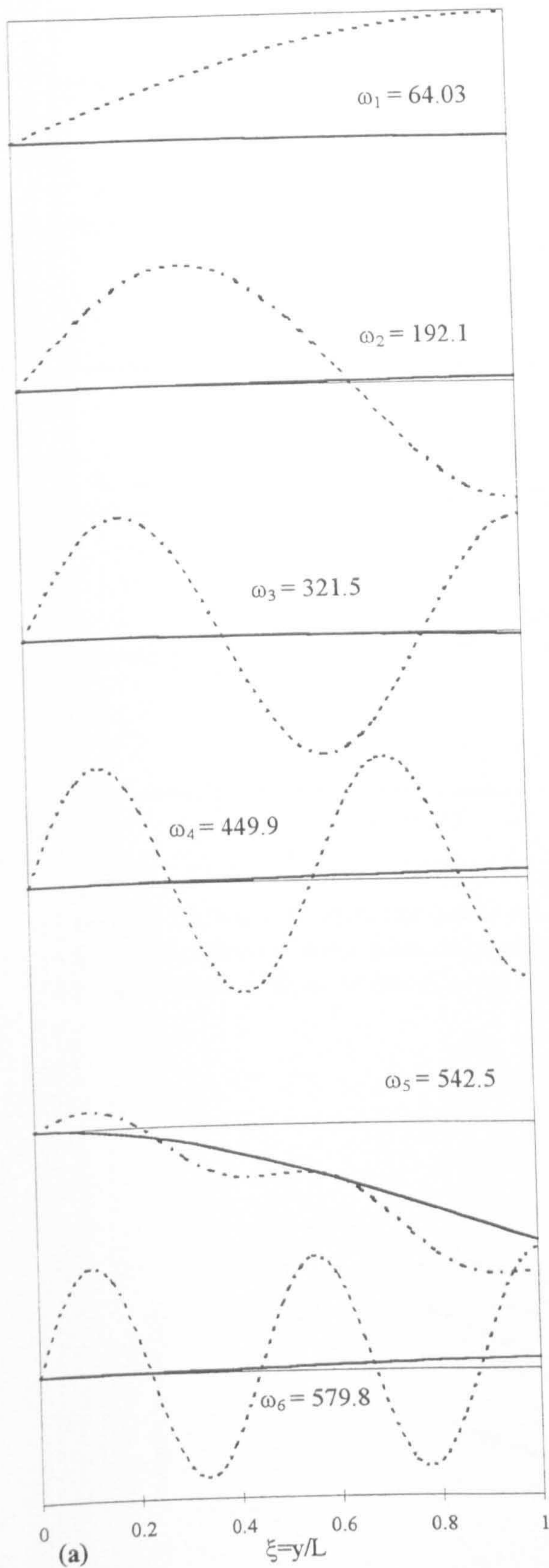
Figure 7-27. Significance of generalised mass in the dynamic response characteristics of a bending-torsion coupled concrete beam with a channel cross-section (Bercin and Tanaka, 1997).
