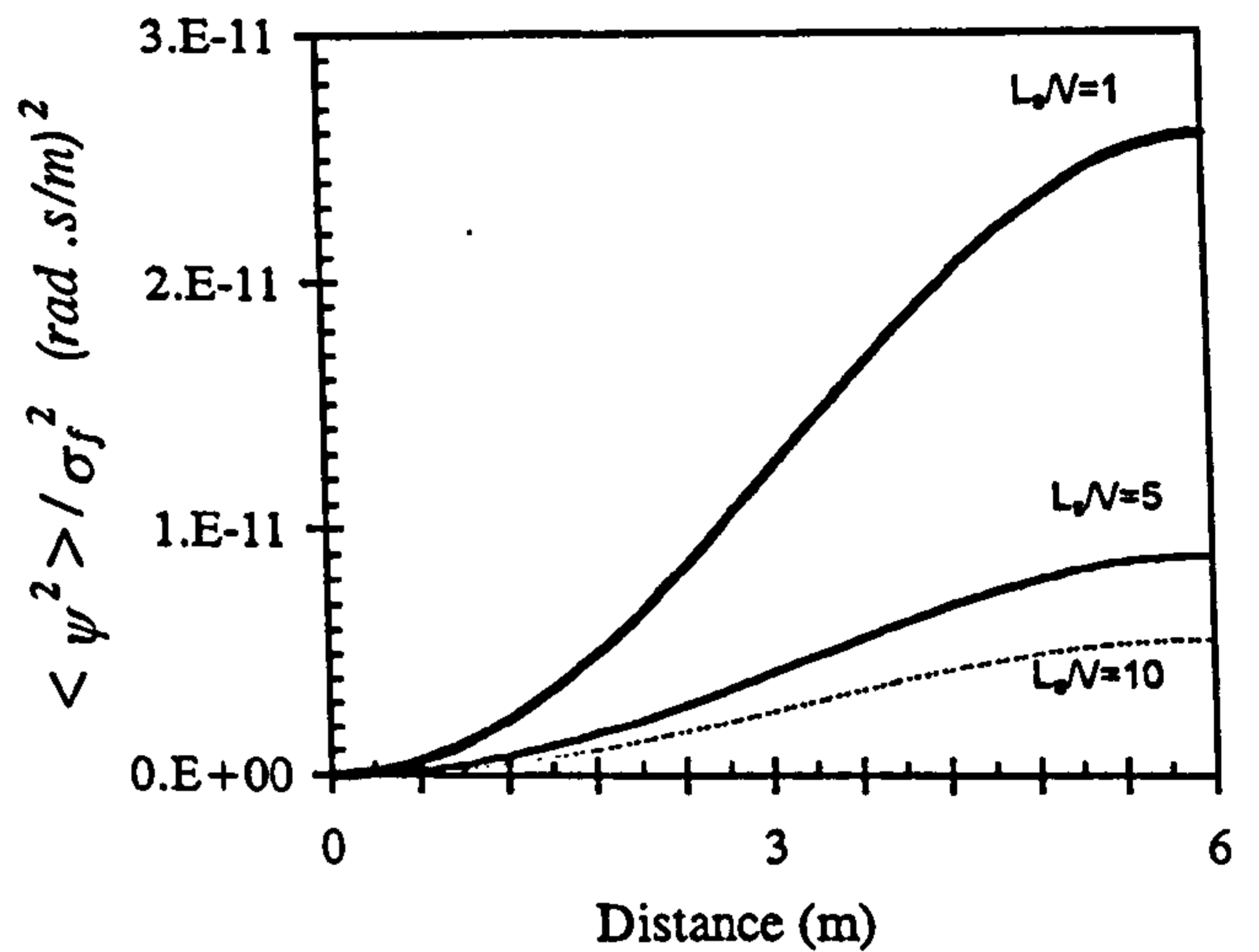
Figure 7-14. Variation of the mean square value of the torsional rotation along the Goland wing (C-F) for different L_p/V ratios (damping coefficient=0.05).
