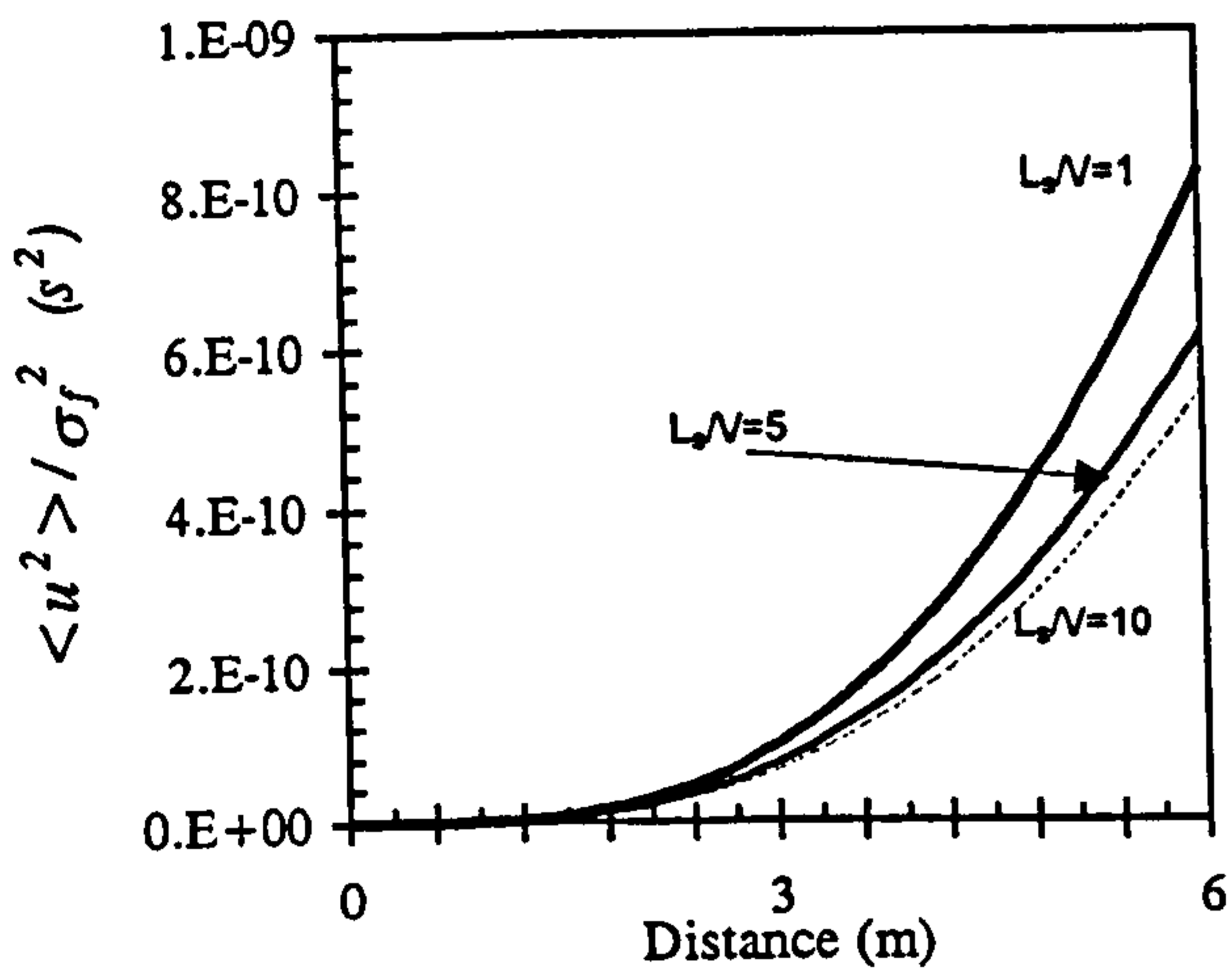
Figure 7-13. Variation of the mean square value of the flexural displacement along the Goland wing (C-F) for different L_p/V ratios (damping coefficient=0.05).
