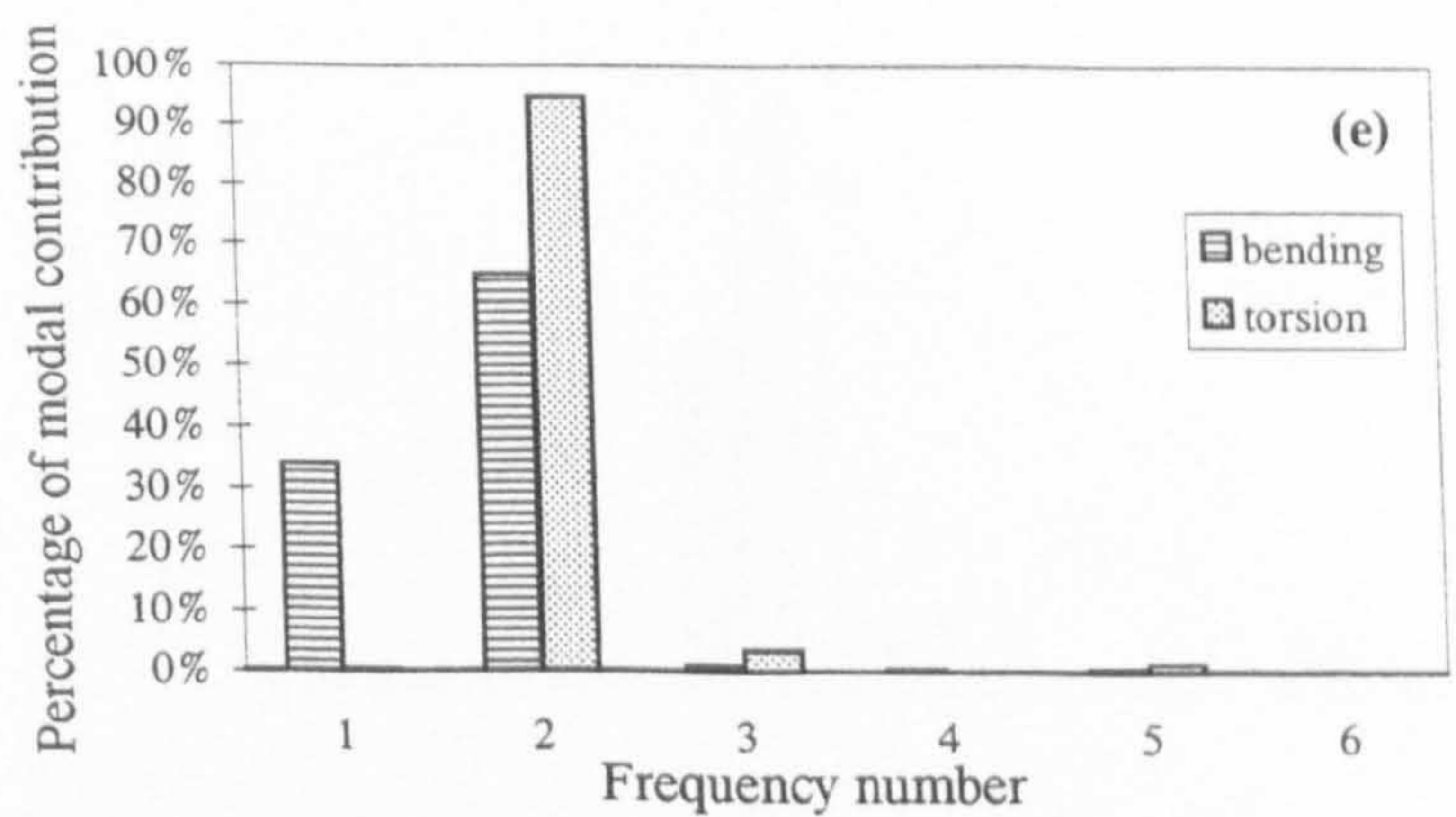
Figure 7-23. Significance of generalised mass in the dynamic response characteristics of a bending-torsion coupled beam. Using the example of Goland wing (Goland, 1945).
