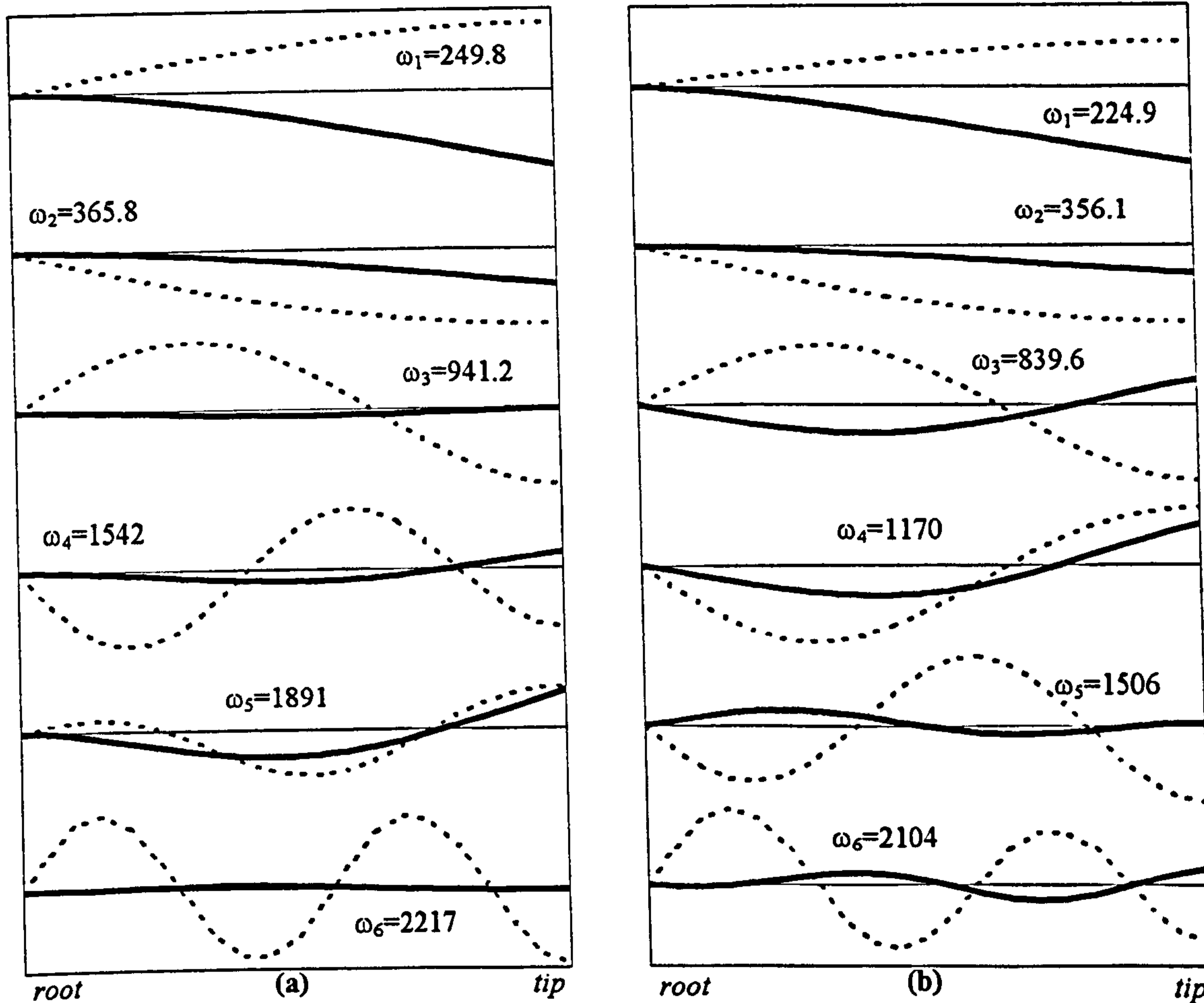
Figure 7-28. Natural frequencies (rad/s) and mode shapes of a turbine blade [L=2.6 m] (Petersen, 1979) (a) without effects of shear deformation and rotatory inertia (b) with effects of shear deformation and rotatory inertia
