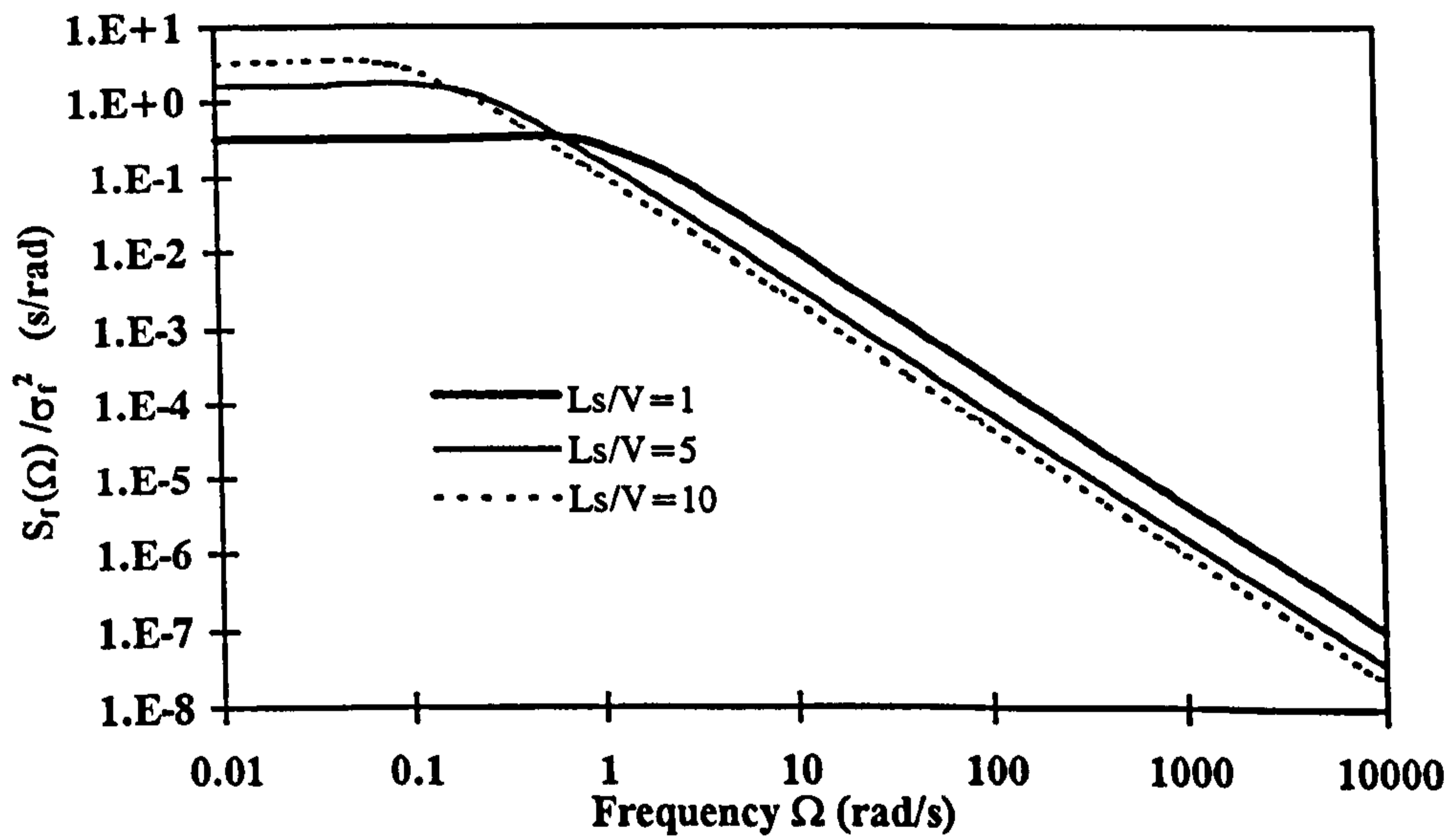
Figure 7-39 The von Karman PSD function for different values of L_v/V .
