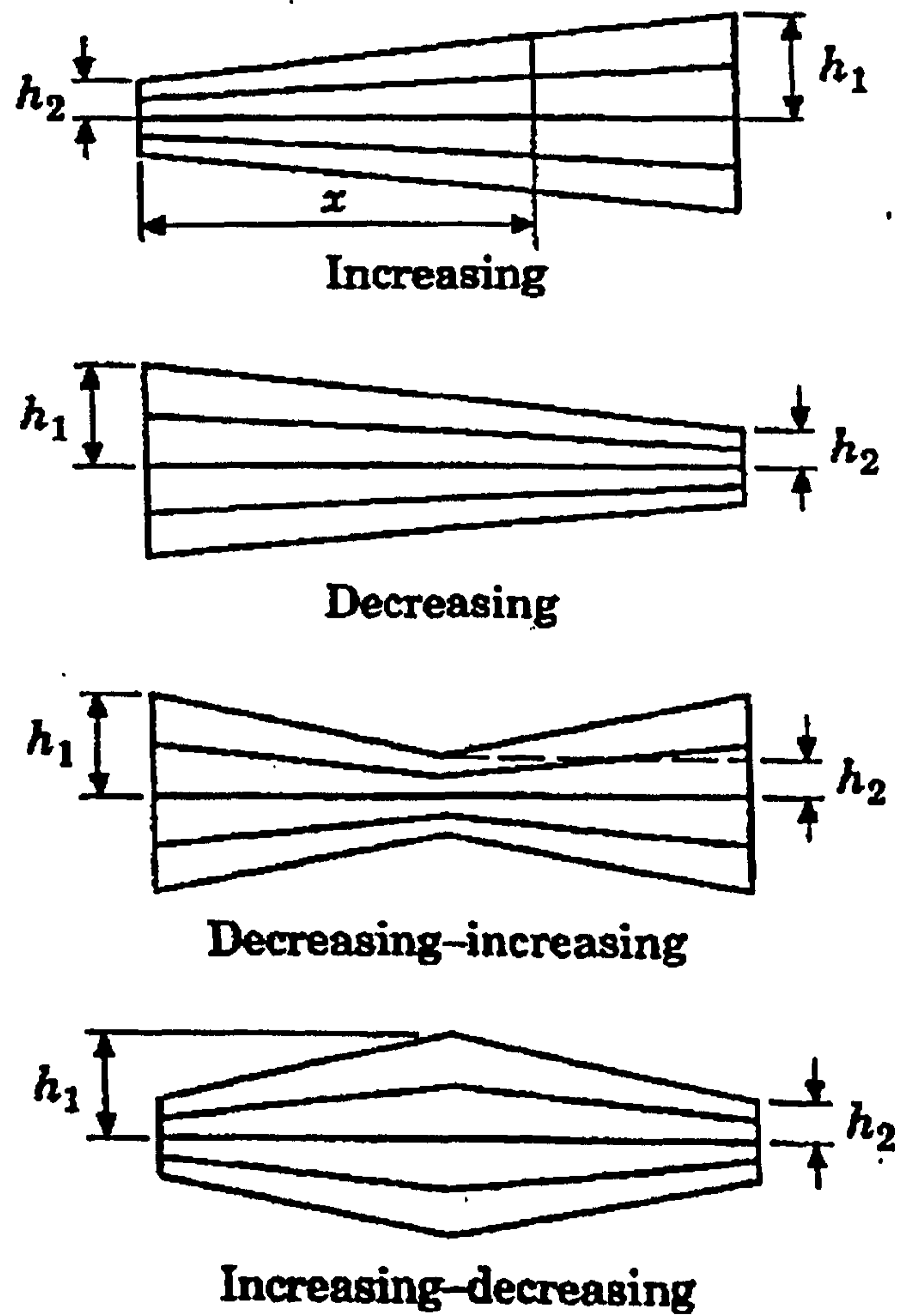
Figure E-2. Different types of taper profile (Rao and Ganesan, 1997).
