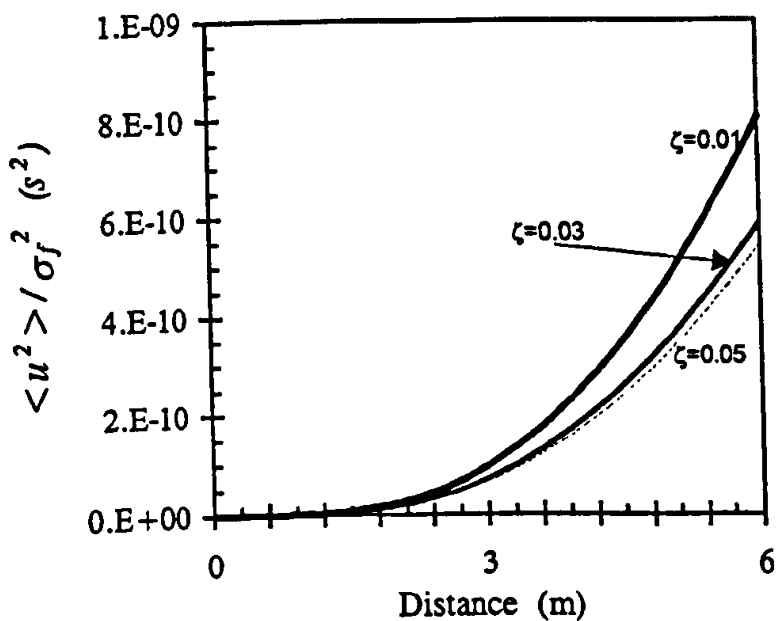
Figure 7-15. Variation of the mean square value of the flexural displacement along the Goland wing (C-F) for different damping coefficients ( L_p/V = 10 ).
