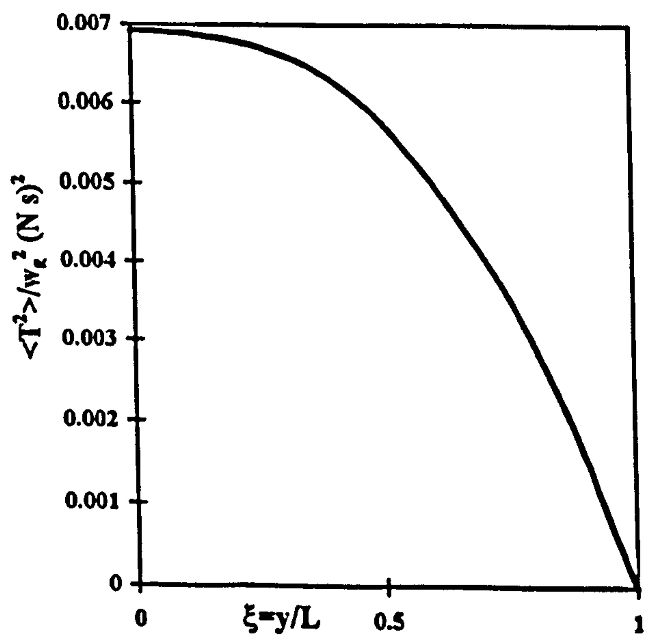
Figure 7-51(b) Variation of the mean square value of torque along the box wing.
