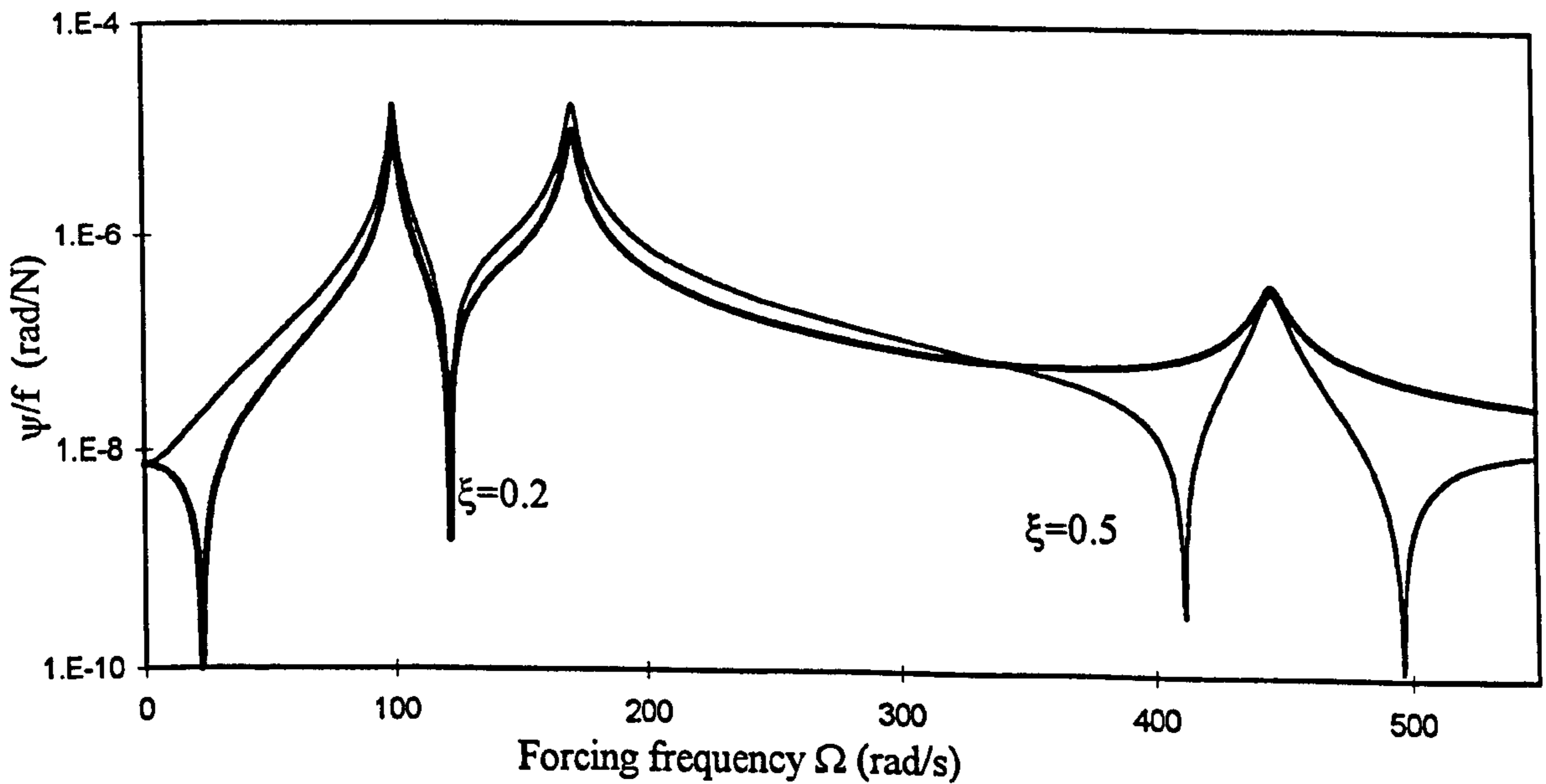
Figure 7-4. Dynamic torsional rotation of the Goland wing with (S-S) end conditions due to a unit harmonically varying force at the mid-span, response at \xi=0.2 and \xi=0.5 .
