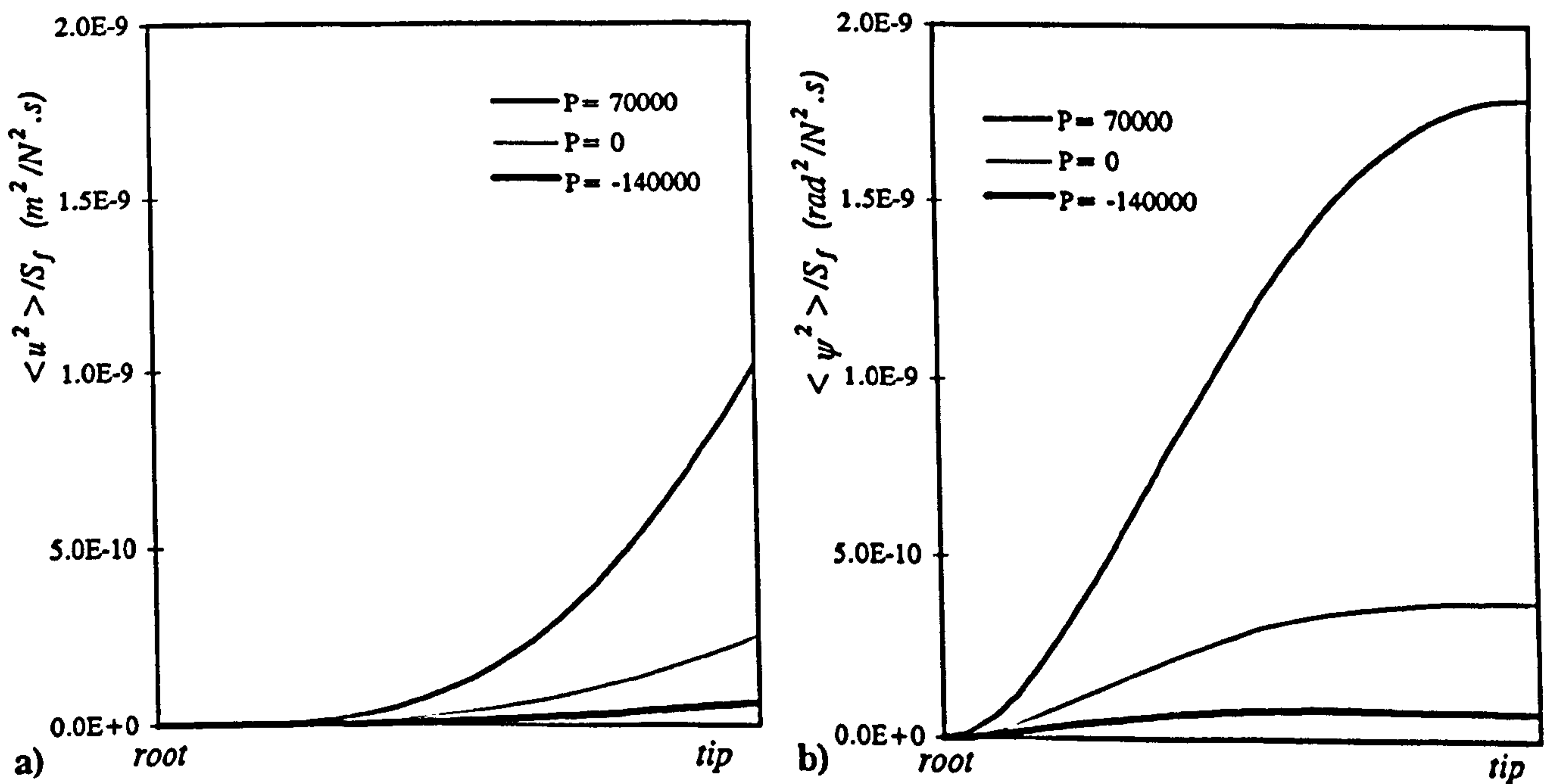
Figure 7-48. Variation of the mean square value of a) flexural b) torsional displacement along the bi-convex beam for different levels of axial load.
