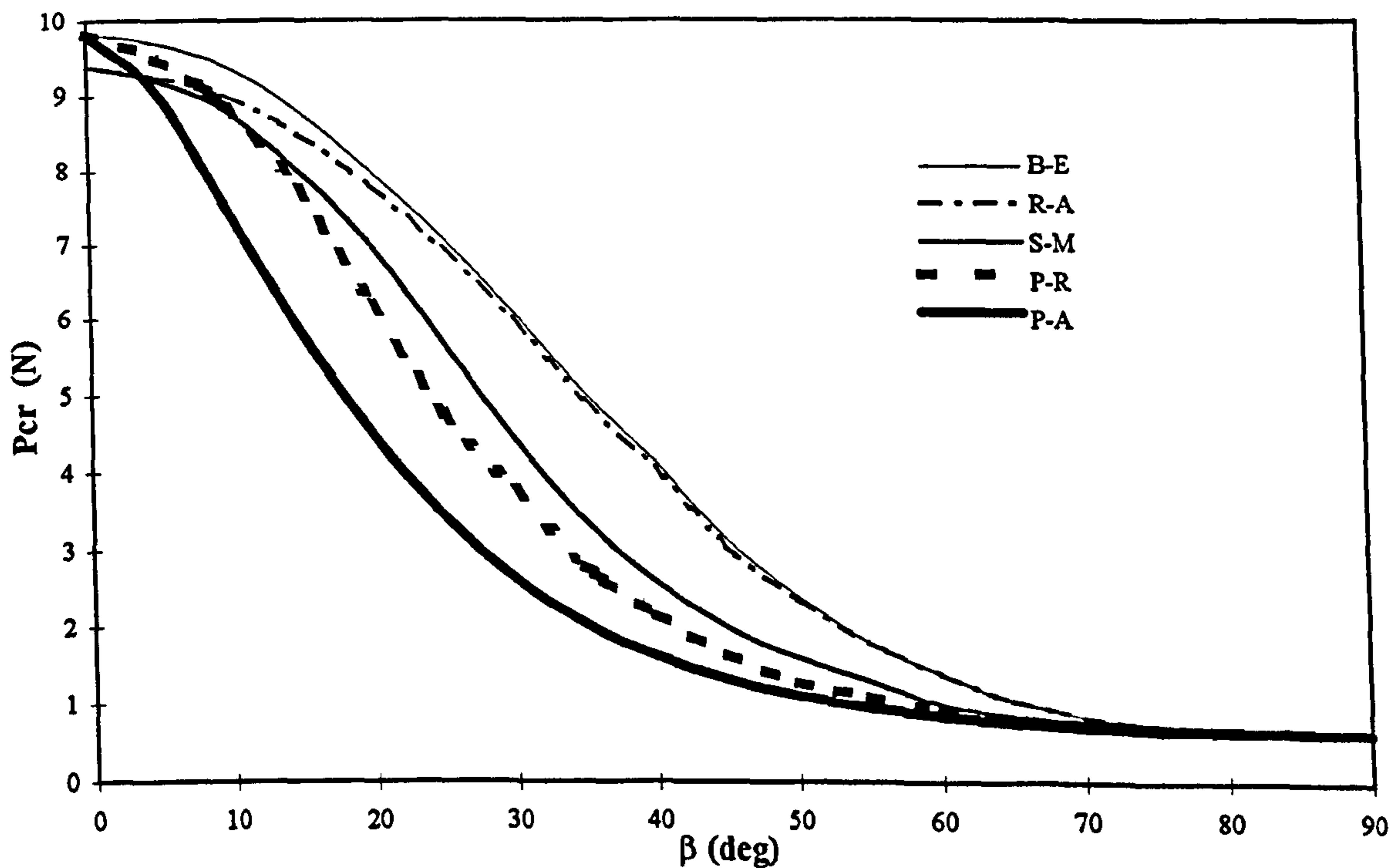
Figure 4-8. Variation of elastic buckling load of a composite box column (Shield and Morey, 1997) with ply angle; a comparison between different buckling theories for composite c
