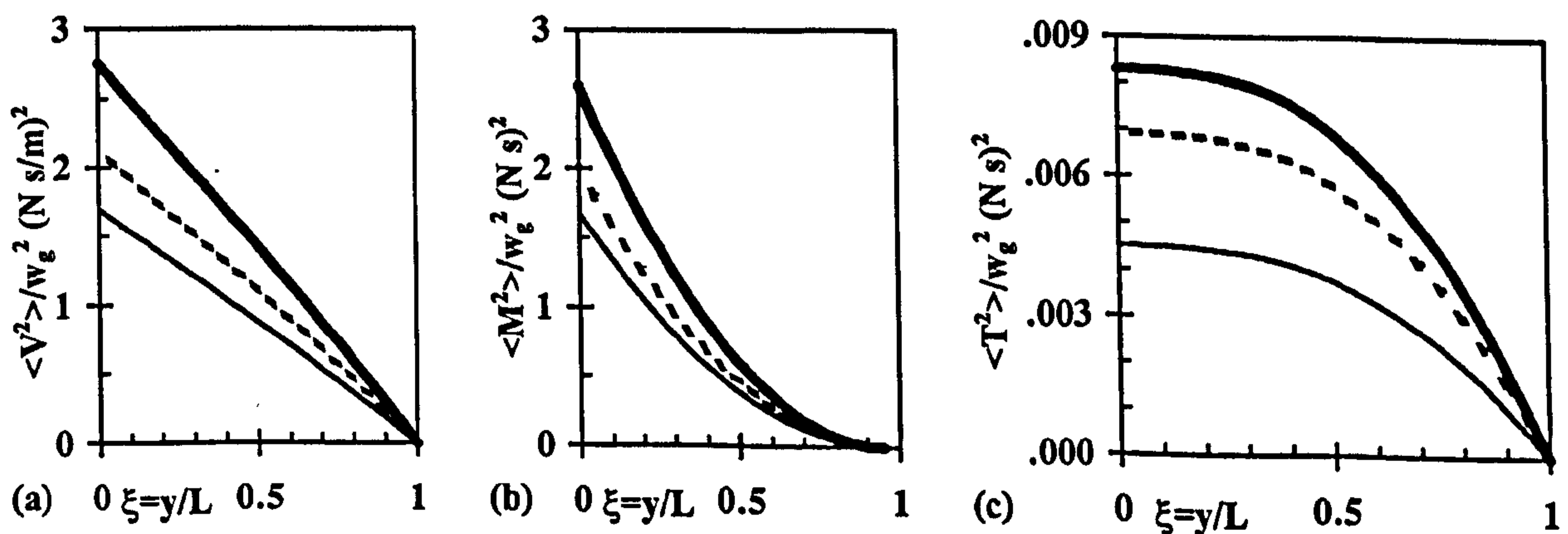
Figure 7-58 Variation of the mean square values of (a) shear force, (b) bending moment and (c) torque along the box wing for different levels of axial load; _____ compressive, - - - - unloaded, — tensile.
