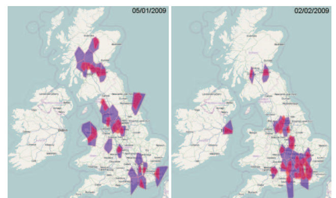
Fig. 22. The screenshots show the areas of the 50km (violet) and 30km (red) divisions having t-events in two selected time intervals.
