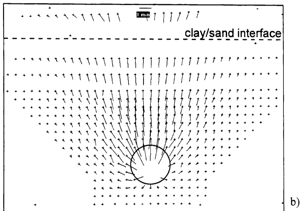
Figure 5.13 Vectors of movement (x15) during centrifuge test RJG20 a) at V \sim 5\% (measured by LVDTs) b) at V \sim 10\% (measured by LVDTs)
