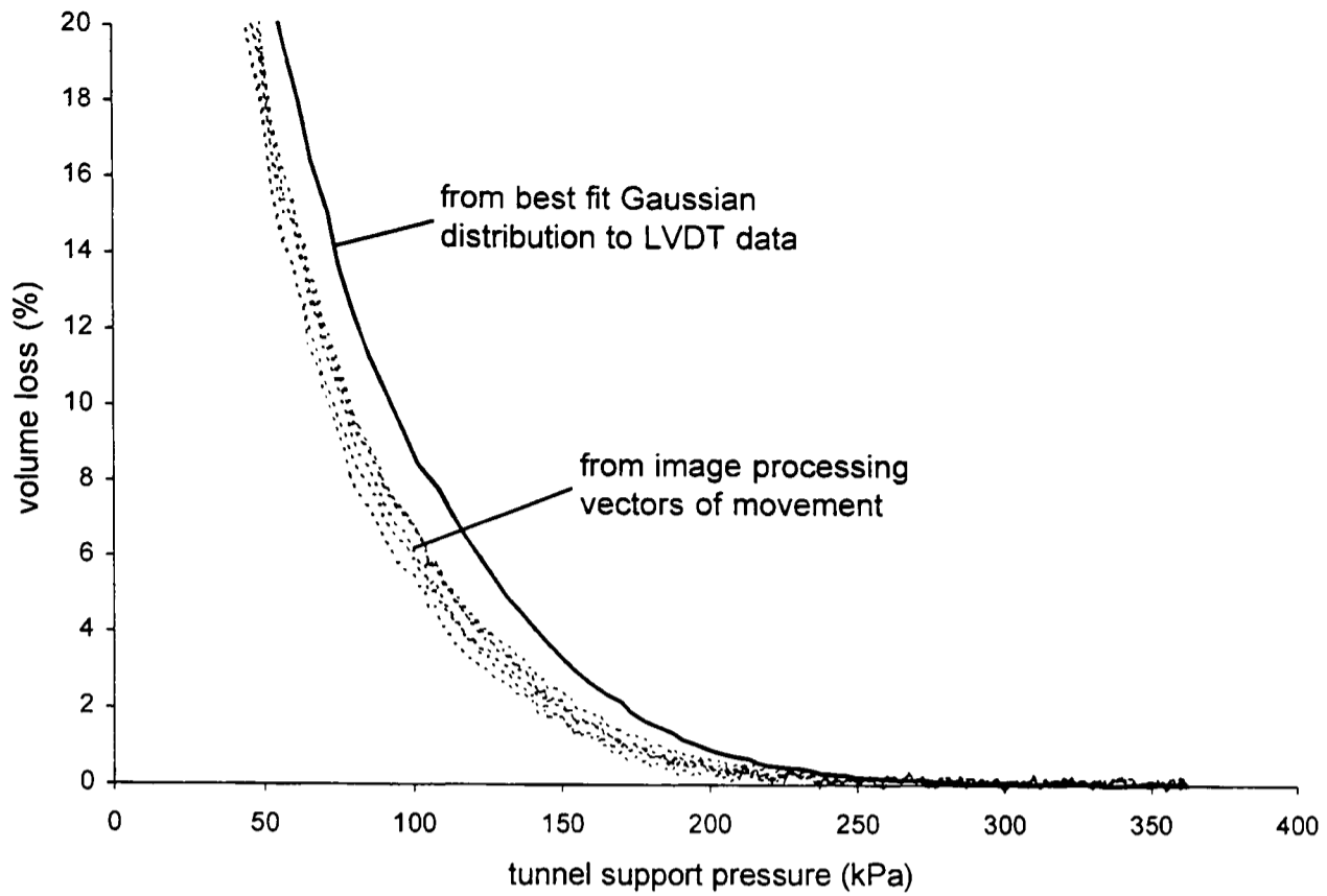
Figure 5.20 Volume losses calculated from LVDT measurements and image processing measurements at various subsurface levels (during centrifuge test RJG20)
