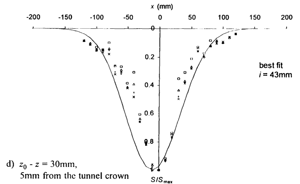
Figure 5.15 Normalised settlement troughs and best fit Gaussian distributions at various subsurface levels in the clay (test RJG20 - 1.5D sand over 2.5D clay above tunnel crown)
