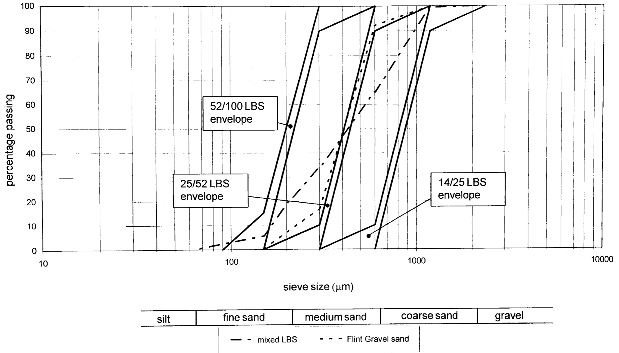
Figure 3.10 Gradings of sands used in tests (gradings for the Leighton Buzzard Sands from the David Ball Company Ltd., Cambridge)
