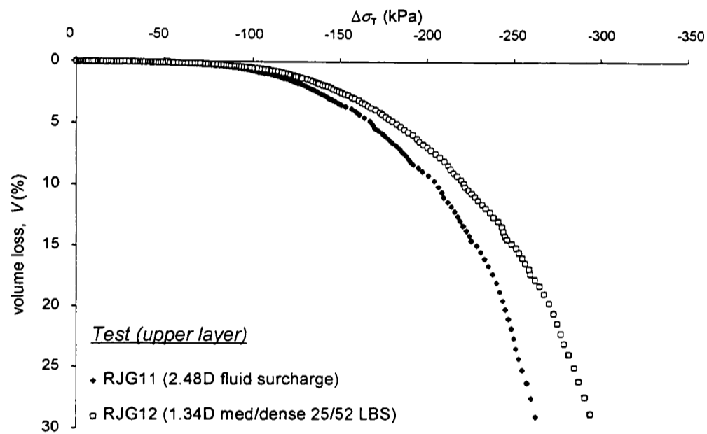
b) RJG11 & 12 (water surcharge equivalent to sand overburden, water table near ground surface)
