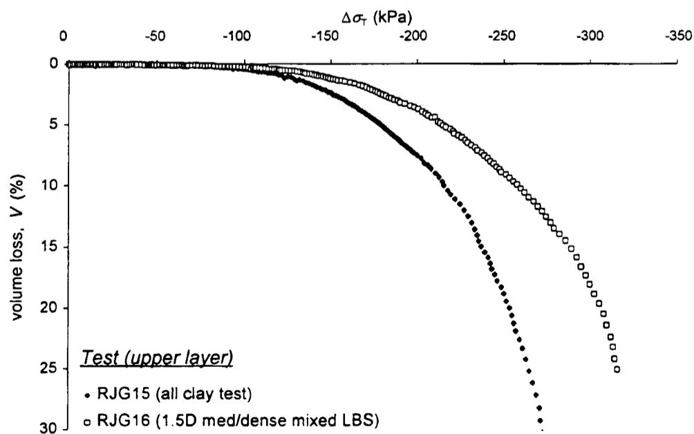
c) RJG15 & 16 (total cover 3D, water table near ground surface)
