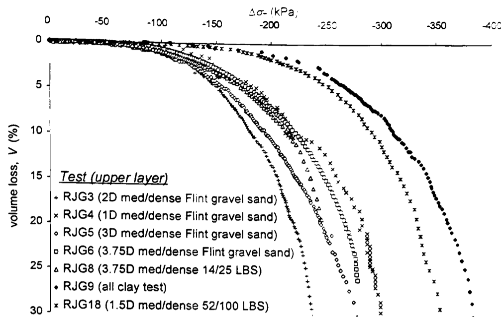
a) RJG3, 4, 5, 6, 8, 9 & 18 (total cover 4D, water table near ground surface)
