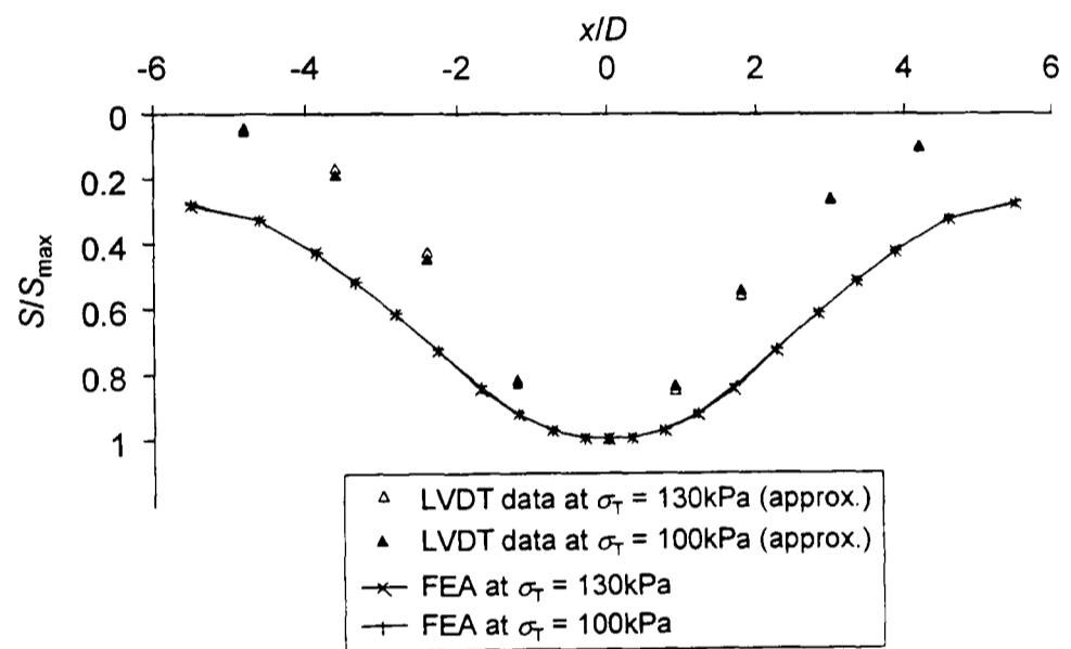
a) clay/sand interface
