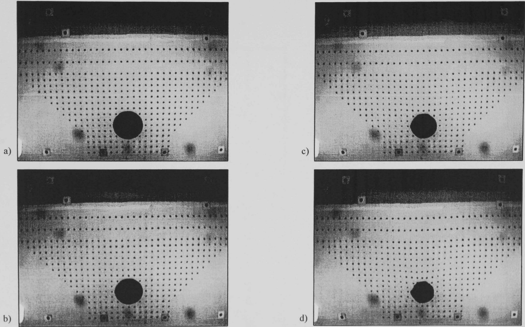
Figure 5.11 Digital images of test RJG20 (1.5D sand over 2.5D clay above tunnel crown) a) before reducing the tunnel pressure, b) when V \sim 10\% , c) when V \sim 20\% and d) when V > 40\% (effectively well after collapse)
