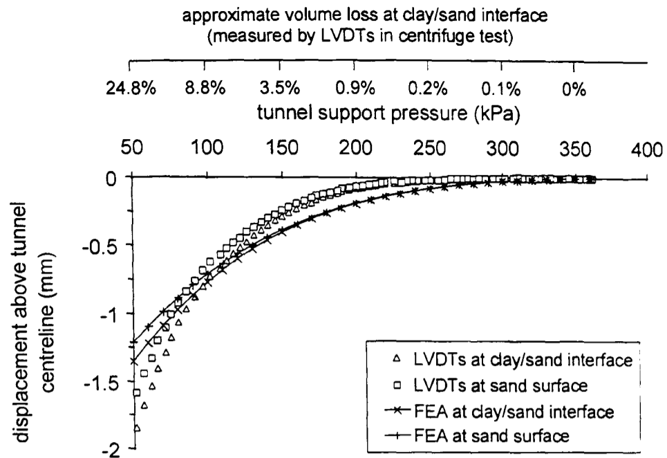
Figure 7.18 Comparison of displacements above the tunnel crown from centrifuge test RJG20 and corresponding finite element analysis RSG1
