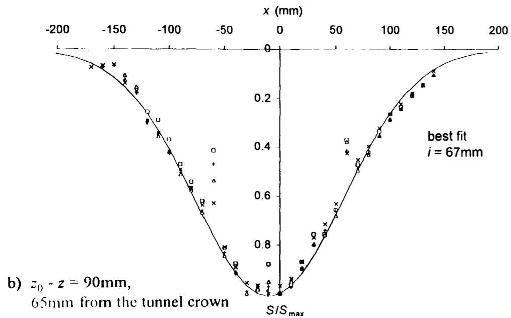
Figure 5.15 Normalised settlement troughs and best fit Gaussian distributions at various subsurface levels in the clay (test RJG20 - 1.5D sand over 2.5D clay above tunnel crown)
