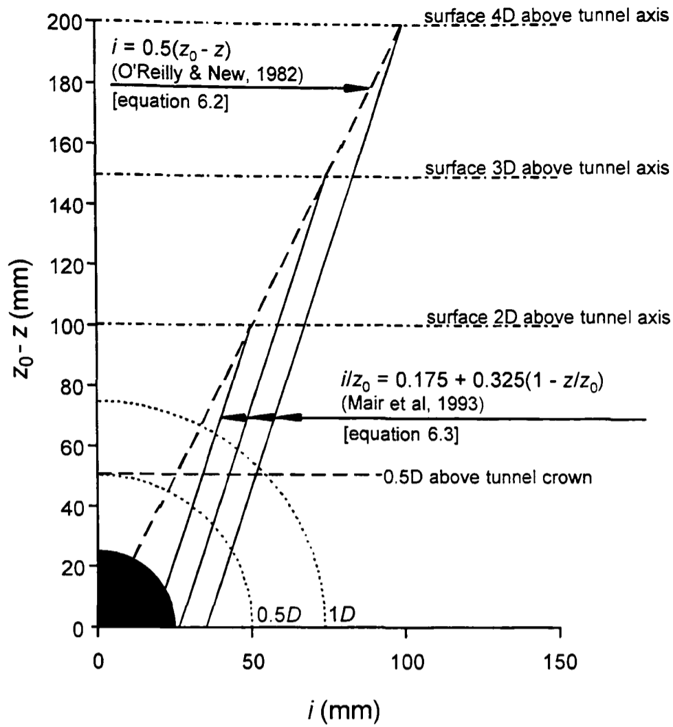
Figure 6.5 Illustration of the commonly applied distributions of i with depth
